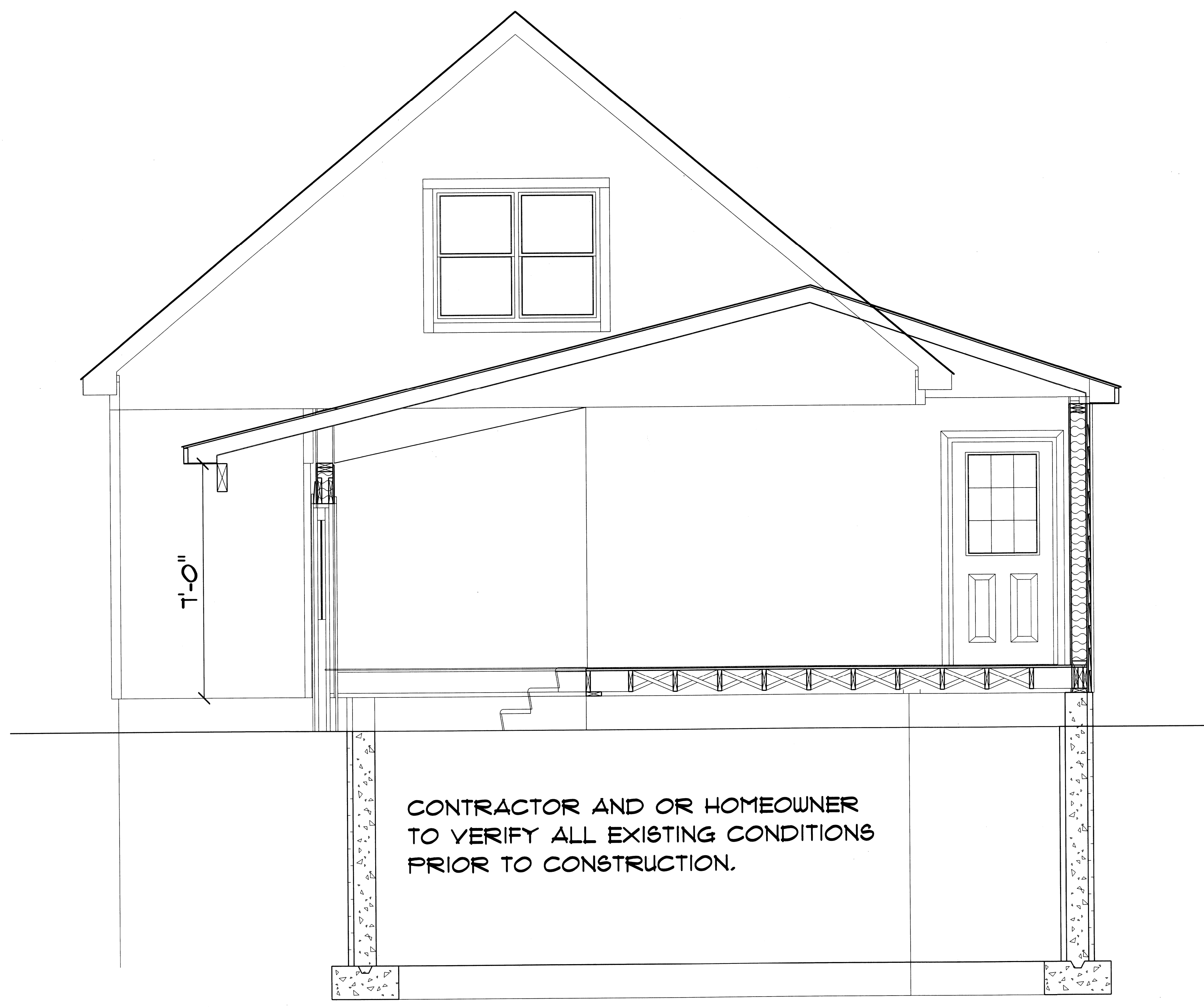
APPROXIMATE ROOF PLANE
