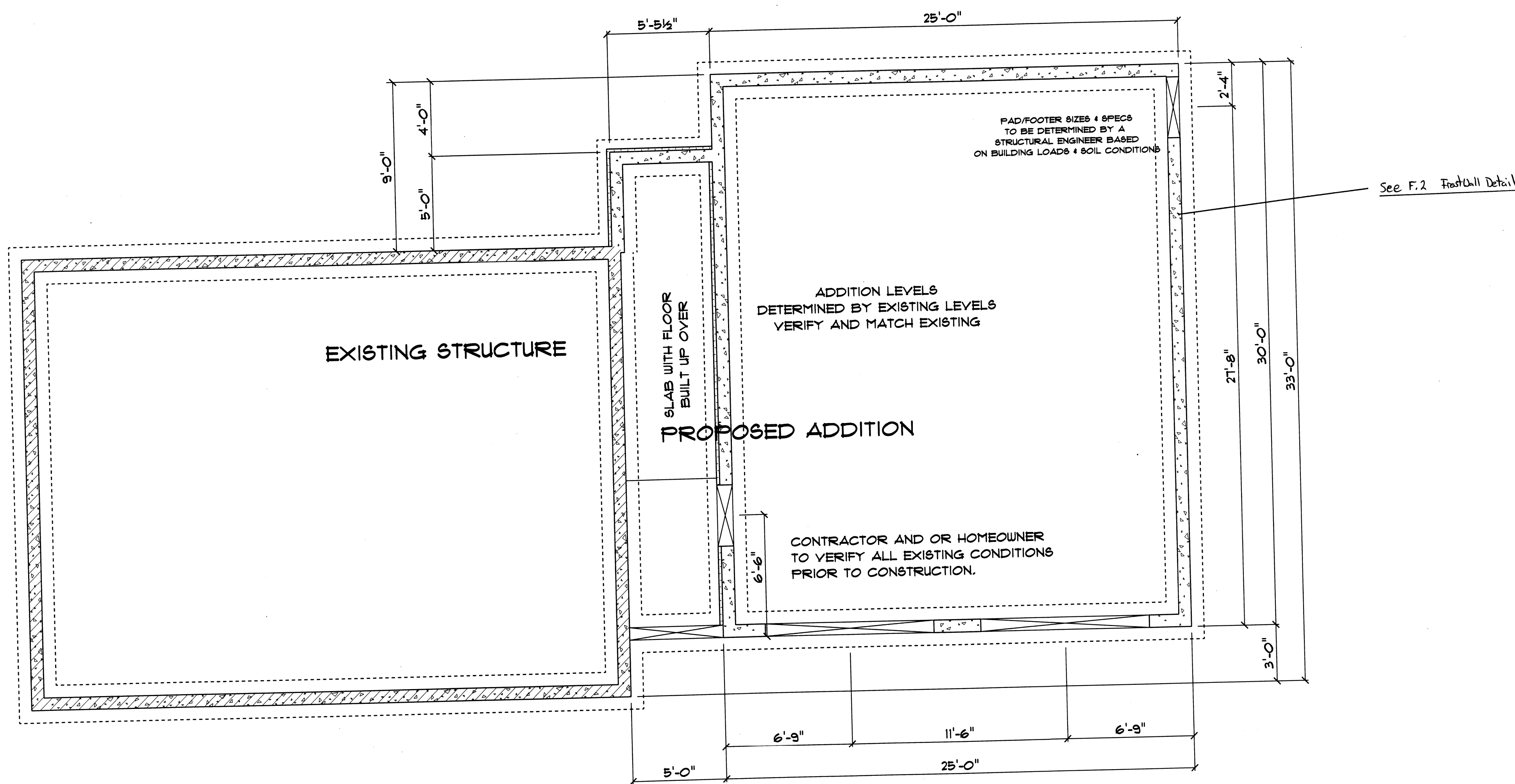
FOUNDATION SCALE: 1/4" = 1'-0"
