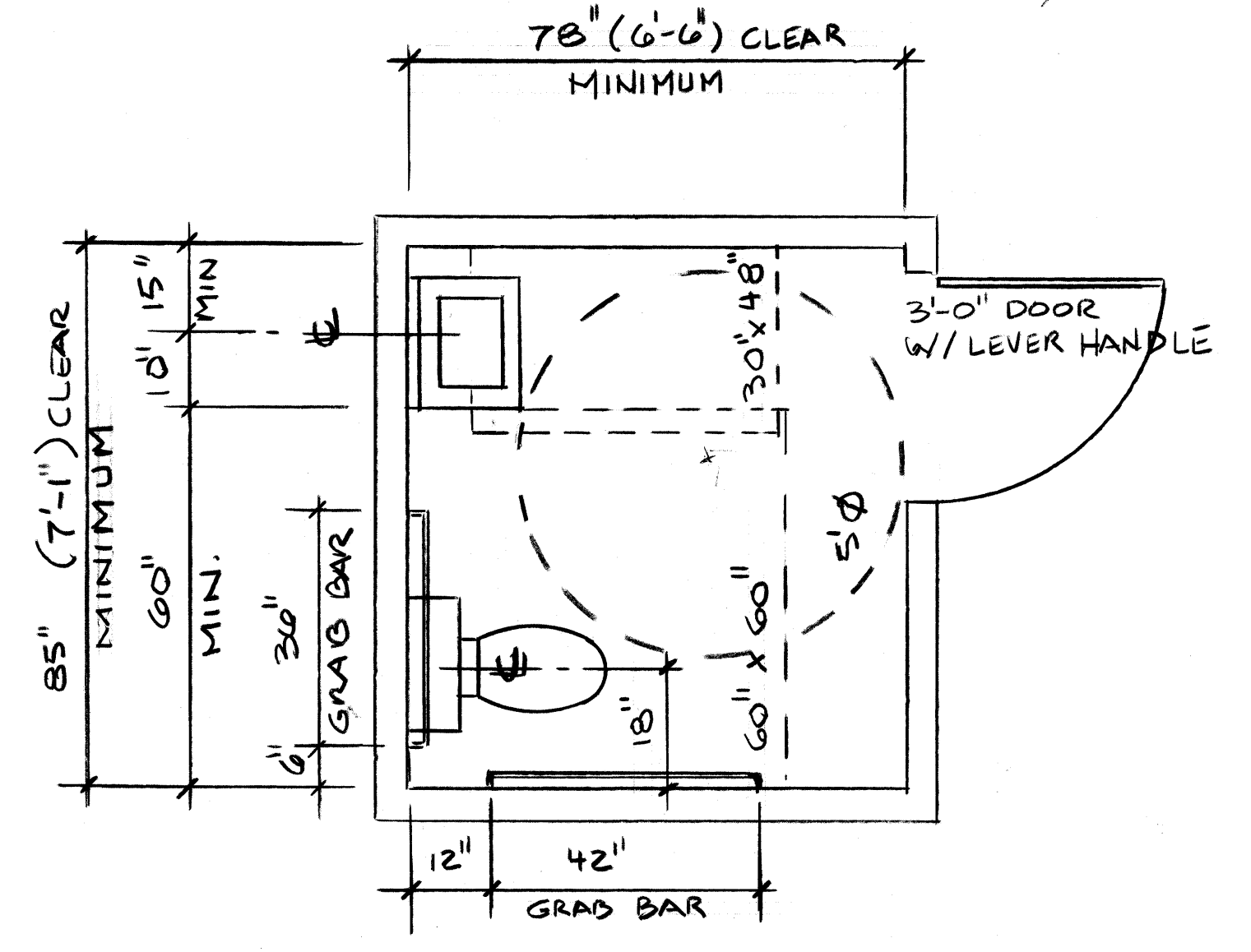
TYPICAL TOILET LAYOUT NTS
