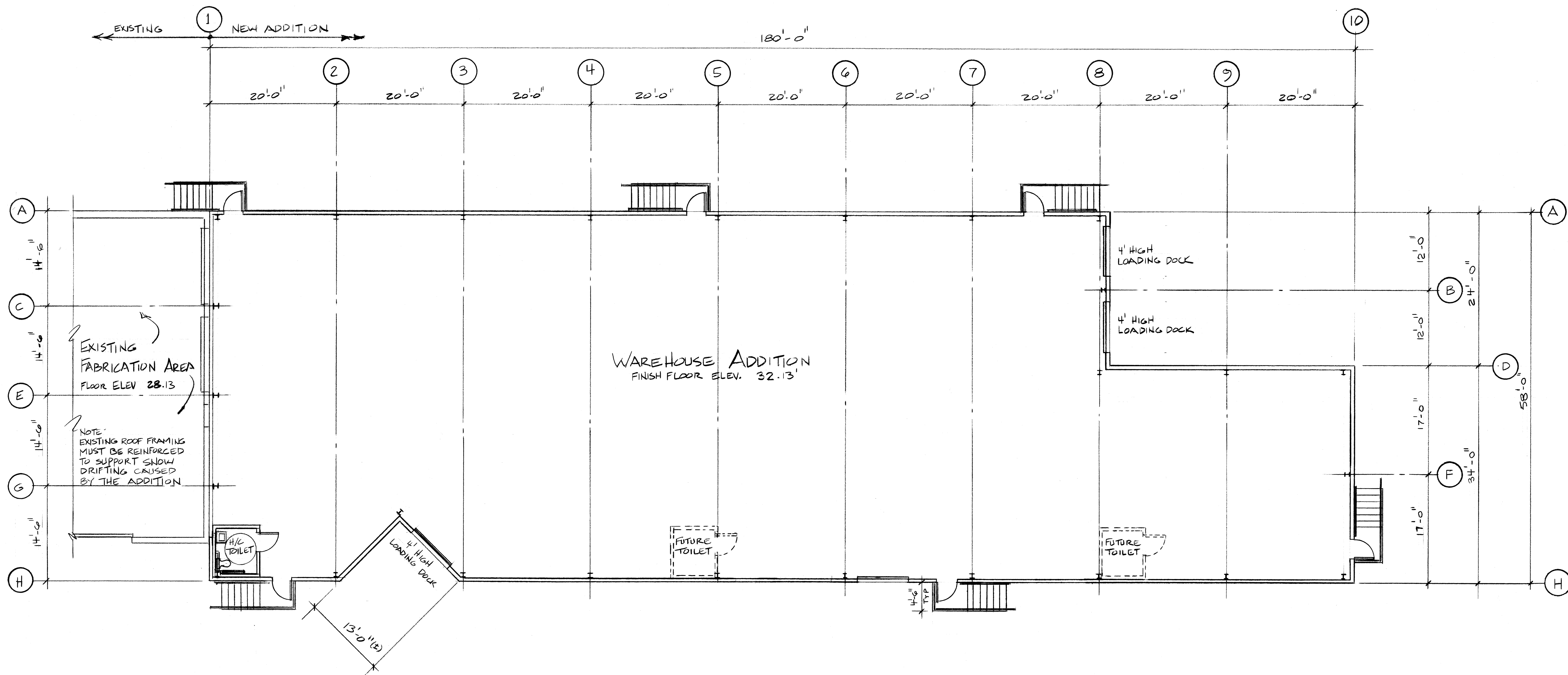
FLOOR PLAN 1/8" = 1'-0"
