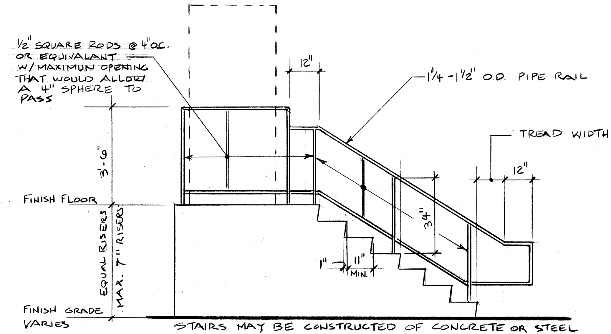
TYPICAL STAIR DETAIL NTS
