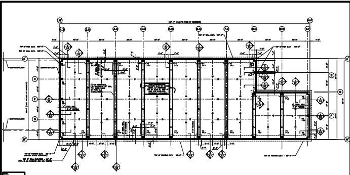
FOUNDATION PLAN
