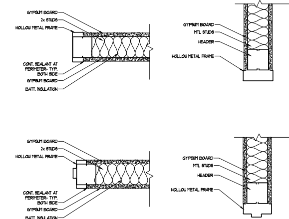
TYPICAL FRAME DETAILS SCALE: NTS
