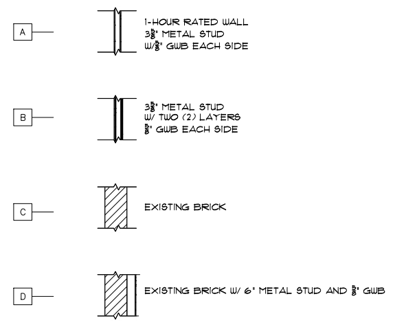
WALL PARTITION TYPE
