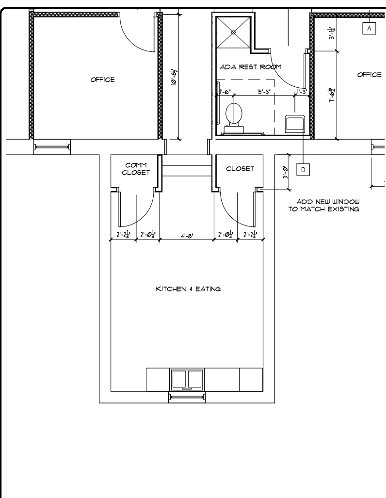
FIRST FLOOR TENANT FIT-UP SCALE: 1/4" = 1'-0"
