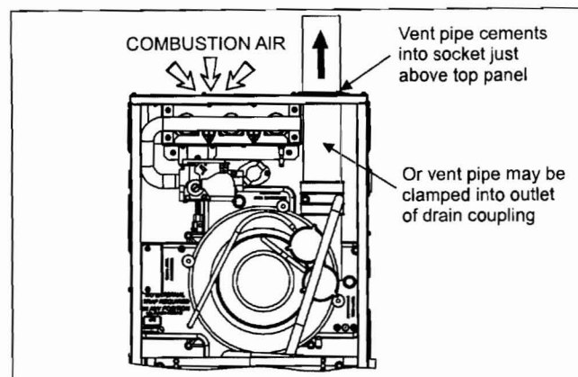
FIGURE 35: Combustion Airflow Path Through The Furnace Casing
