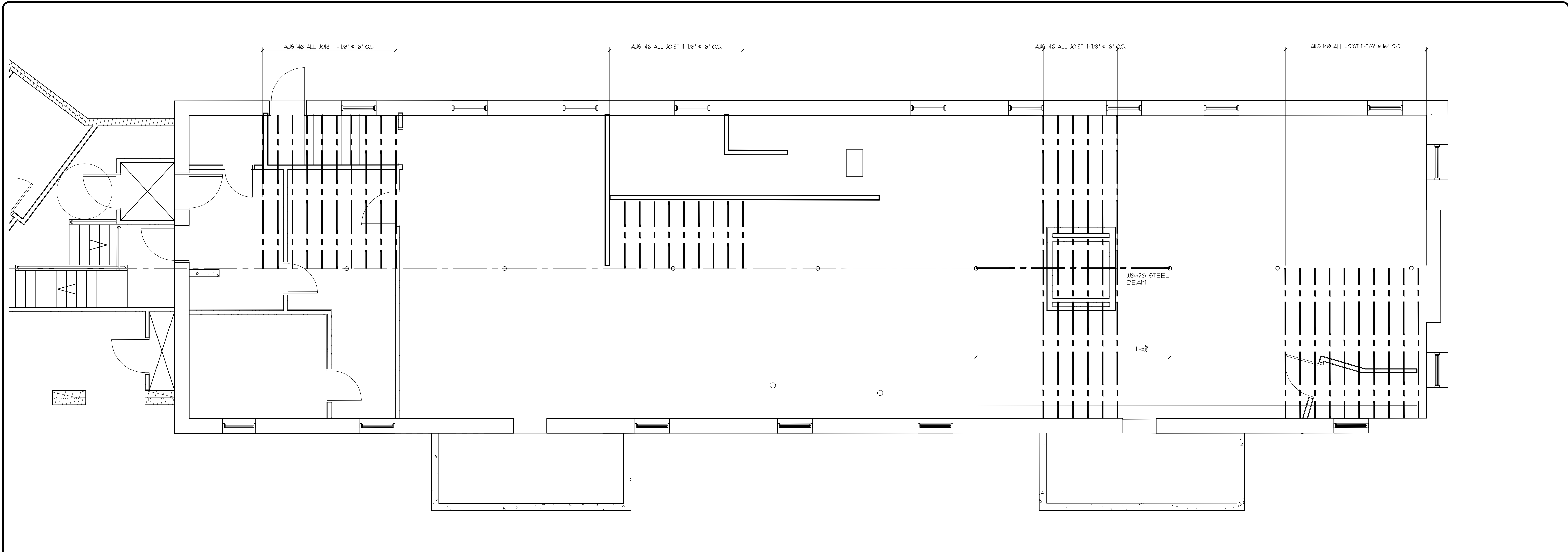
MAIN FLOOR LIFE-SAFETY PLAN SCALE: 1/4" = 1'-0"
