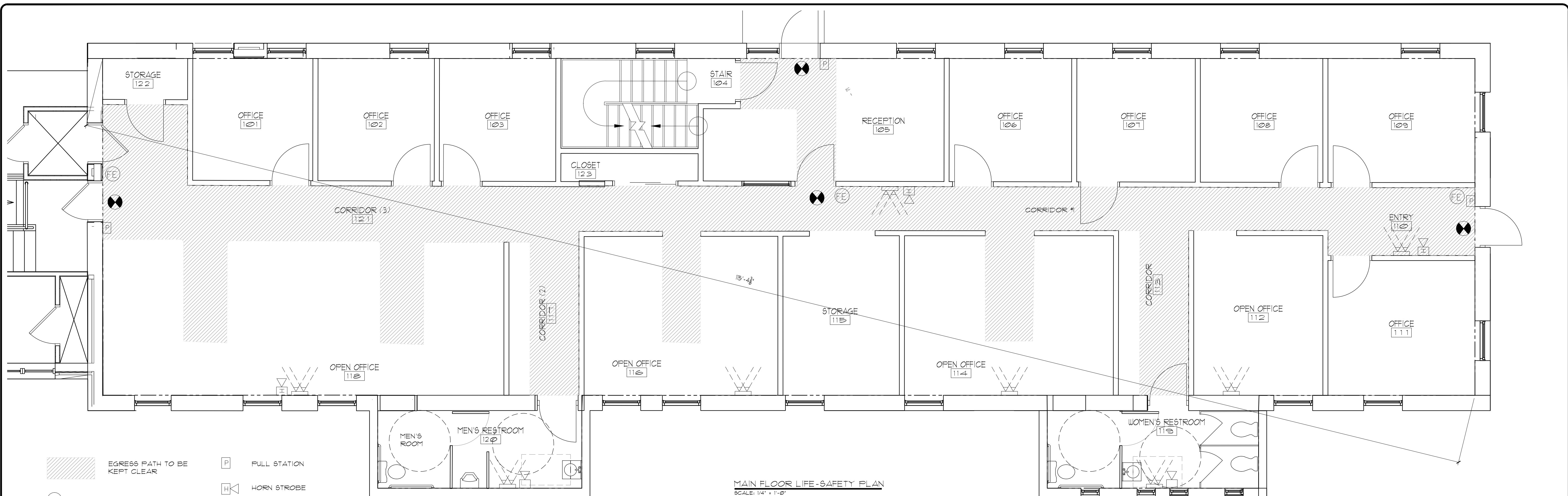
MAIN FLOOR LIFE-SAFETY PLAN SCALE: 1/4" = 1'-0"
