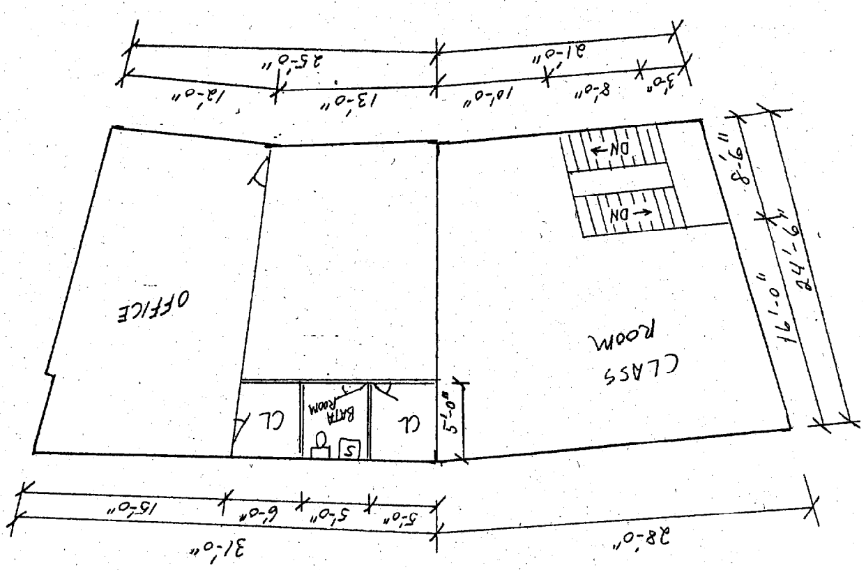
2nd FLOOR PLAN AFTER CONSTRUCTION
