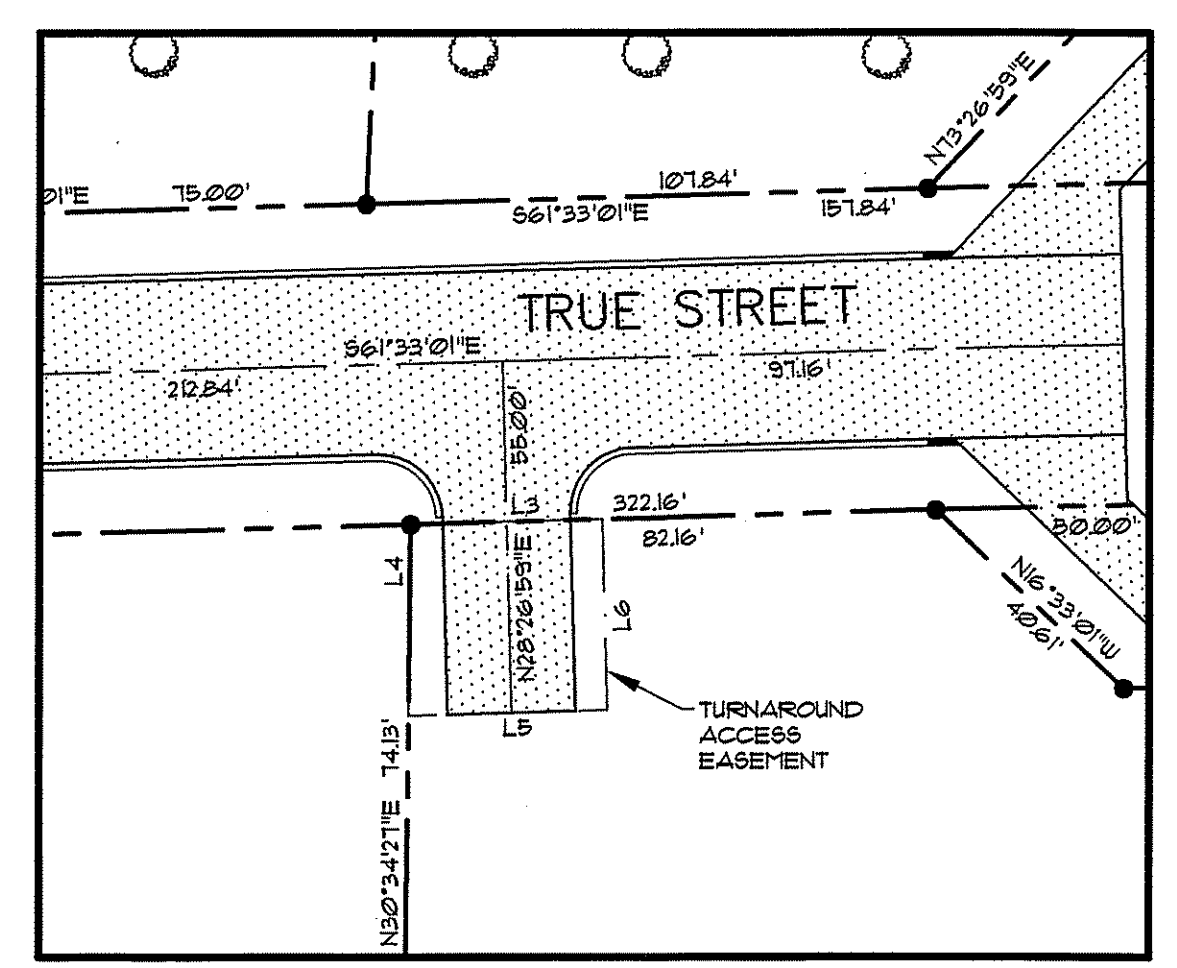
TURNAROUND DETAIL
