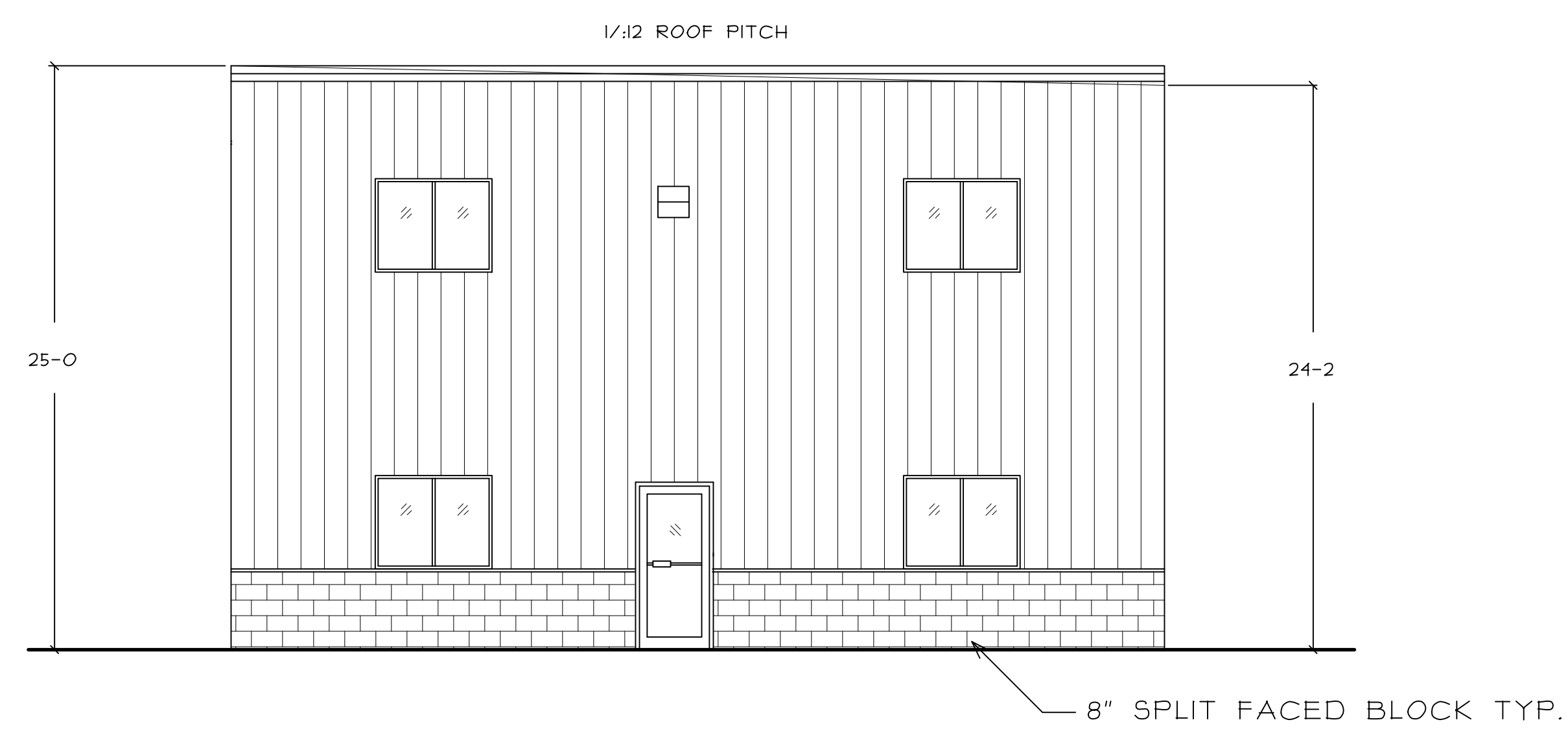
FRONT ELEVATION
