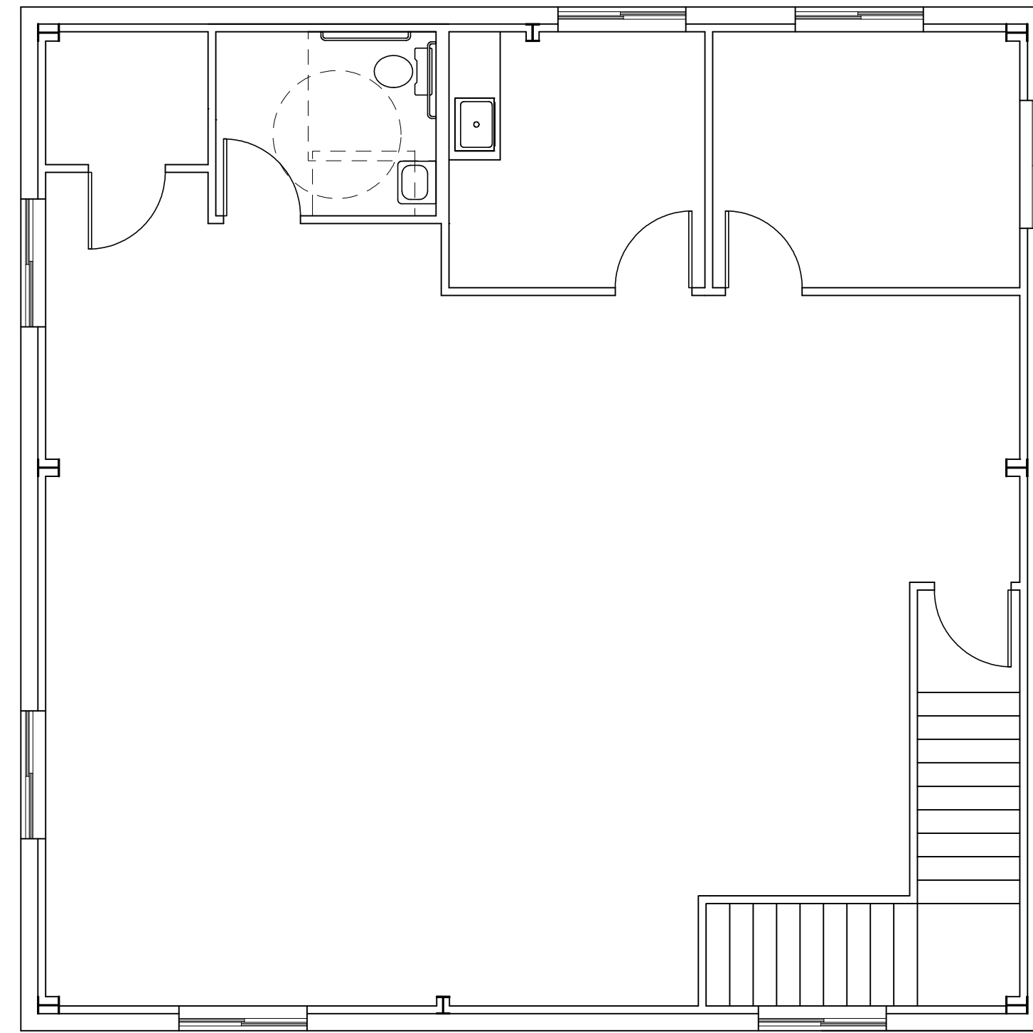
SECOND FLOOR
