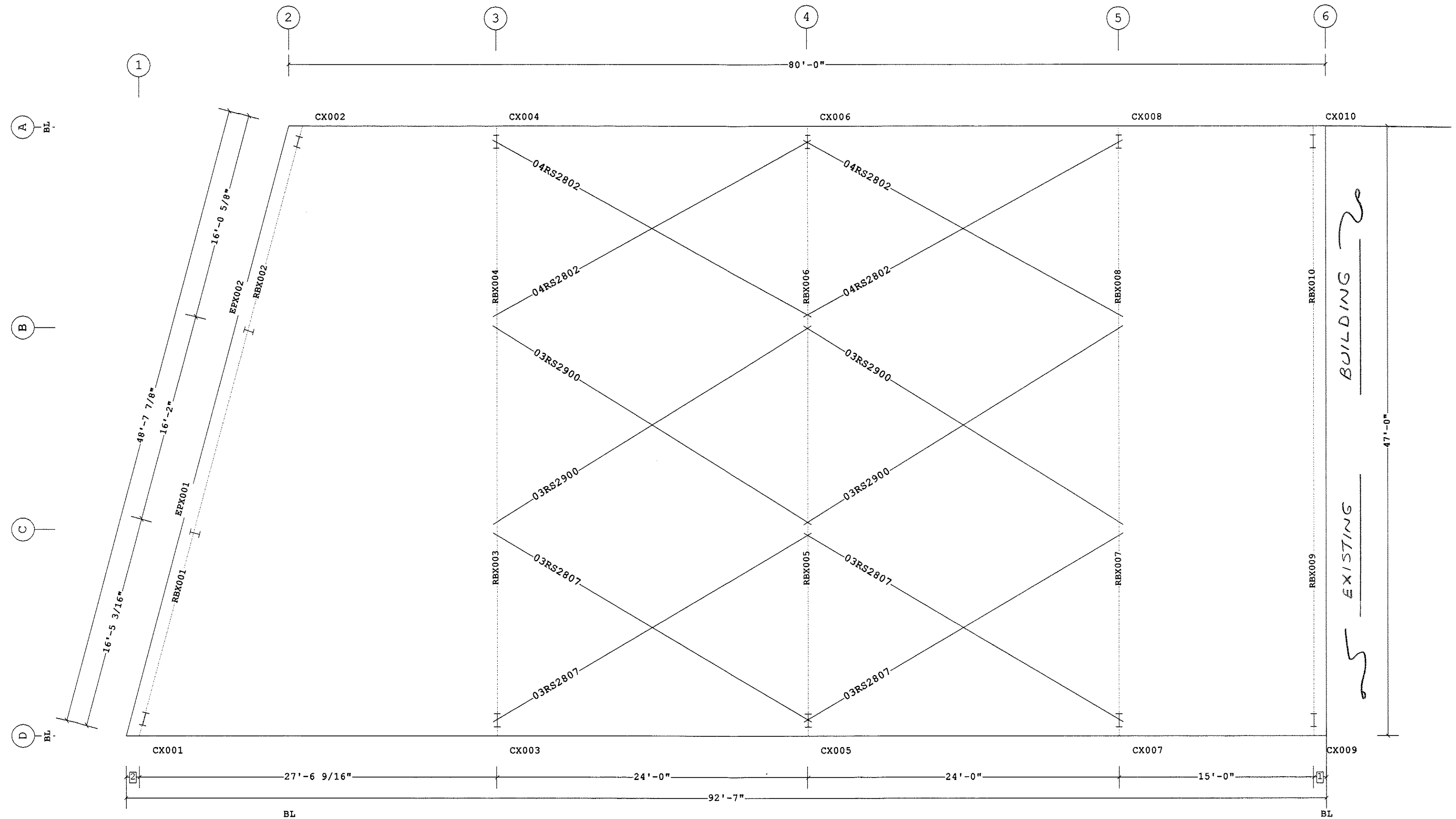
PRIMARY AND ROOF BRACING PLAN
