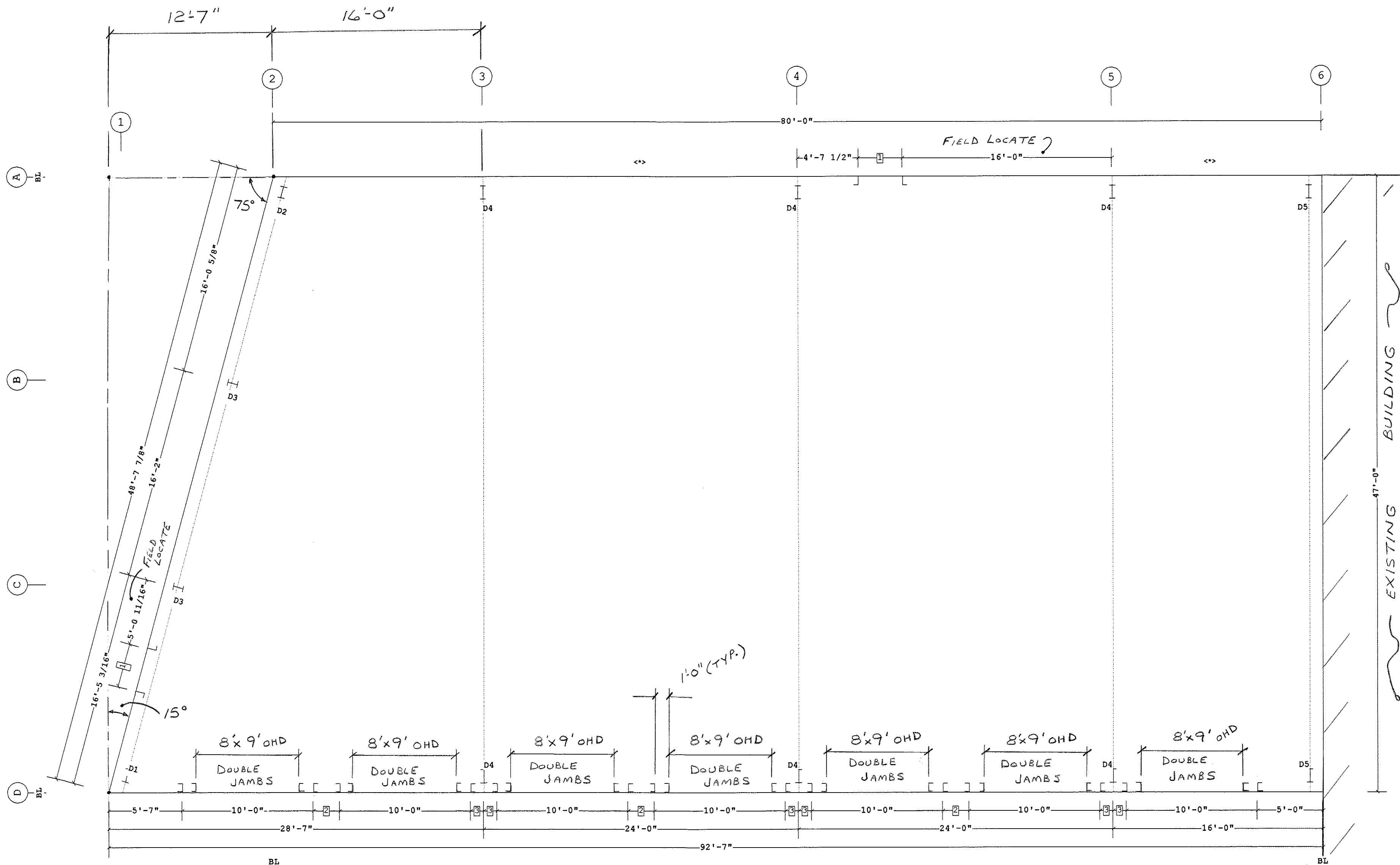
ANCHOR ROD PLAN
