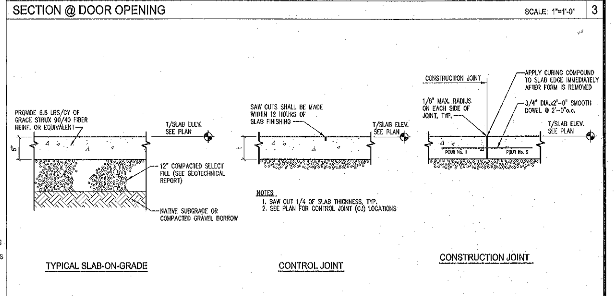
SECTION @ DOOR OPENING SCALE: 1"=1'-0"
