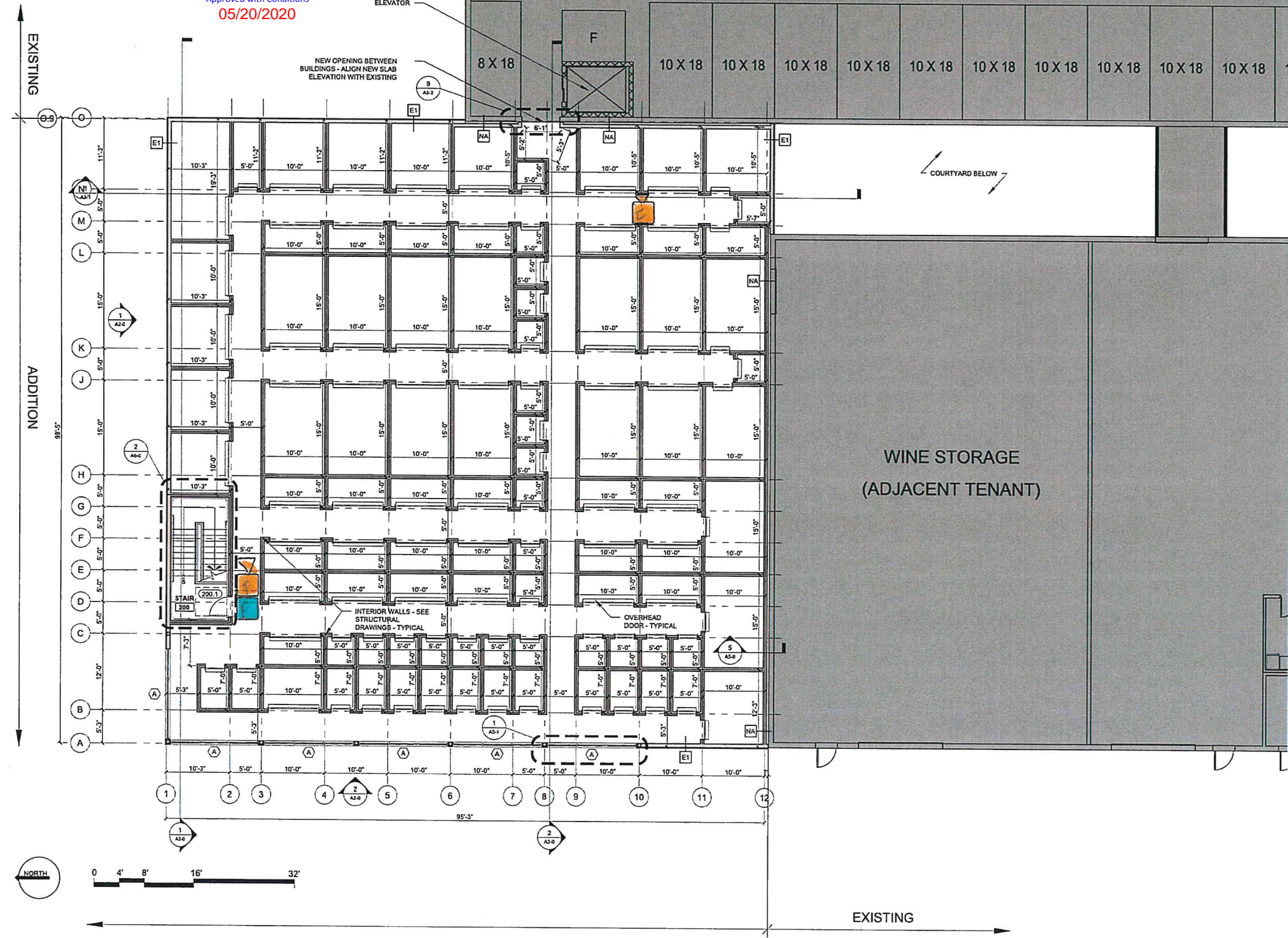
1 SECOND FLOOR PLAN 1/8" = 1'-0"
