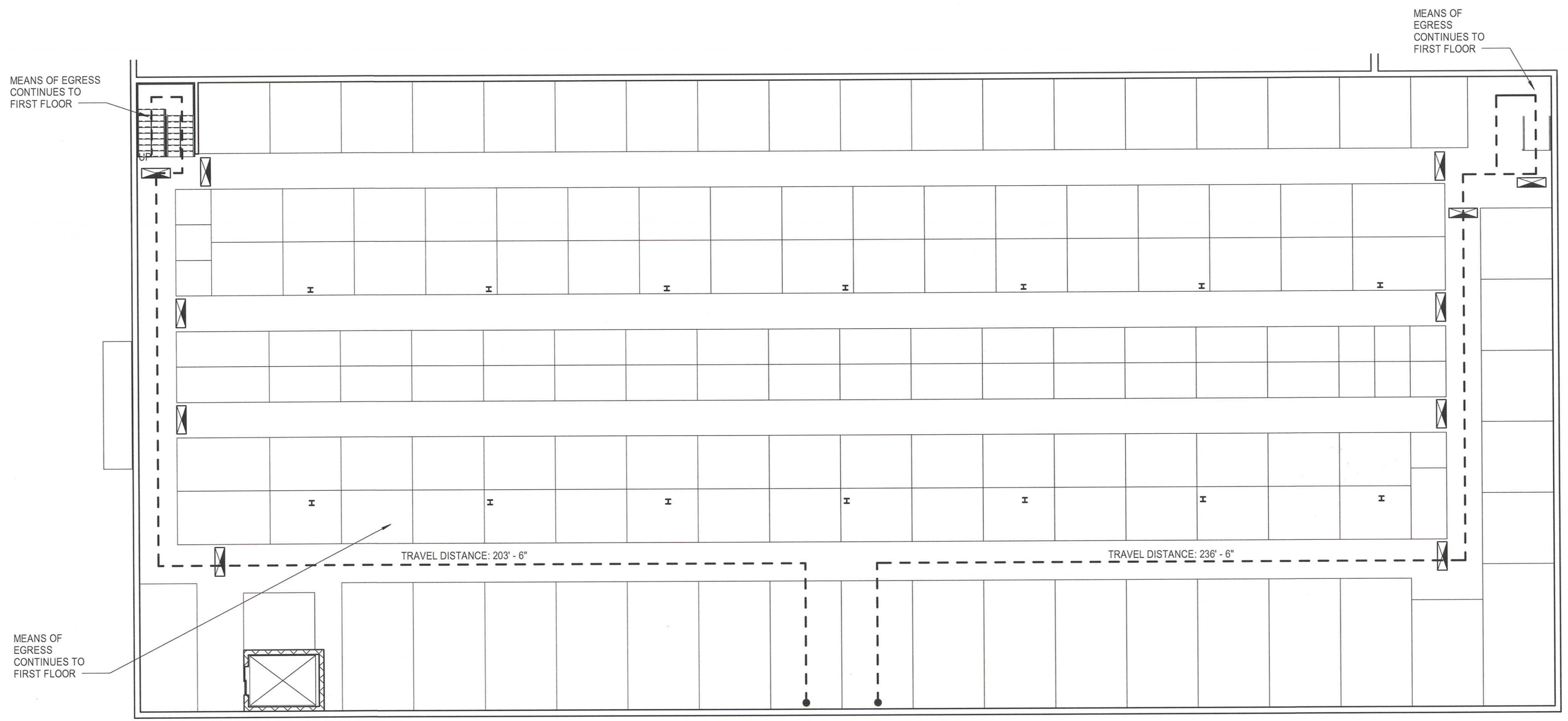
G4 SECOND FLOOR - LIFE SAFETY 3/32" = 1'-0"
