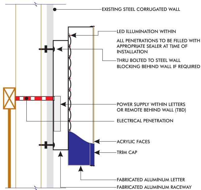
TYPICAL SECTION NO SCALE
