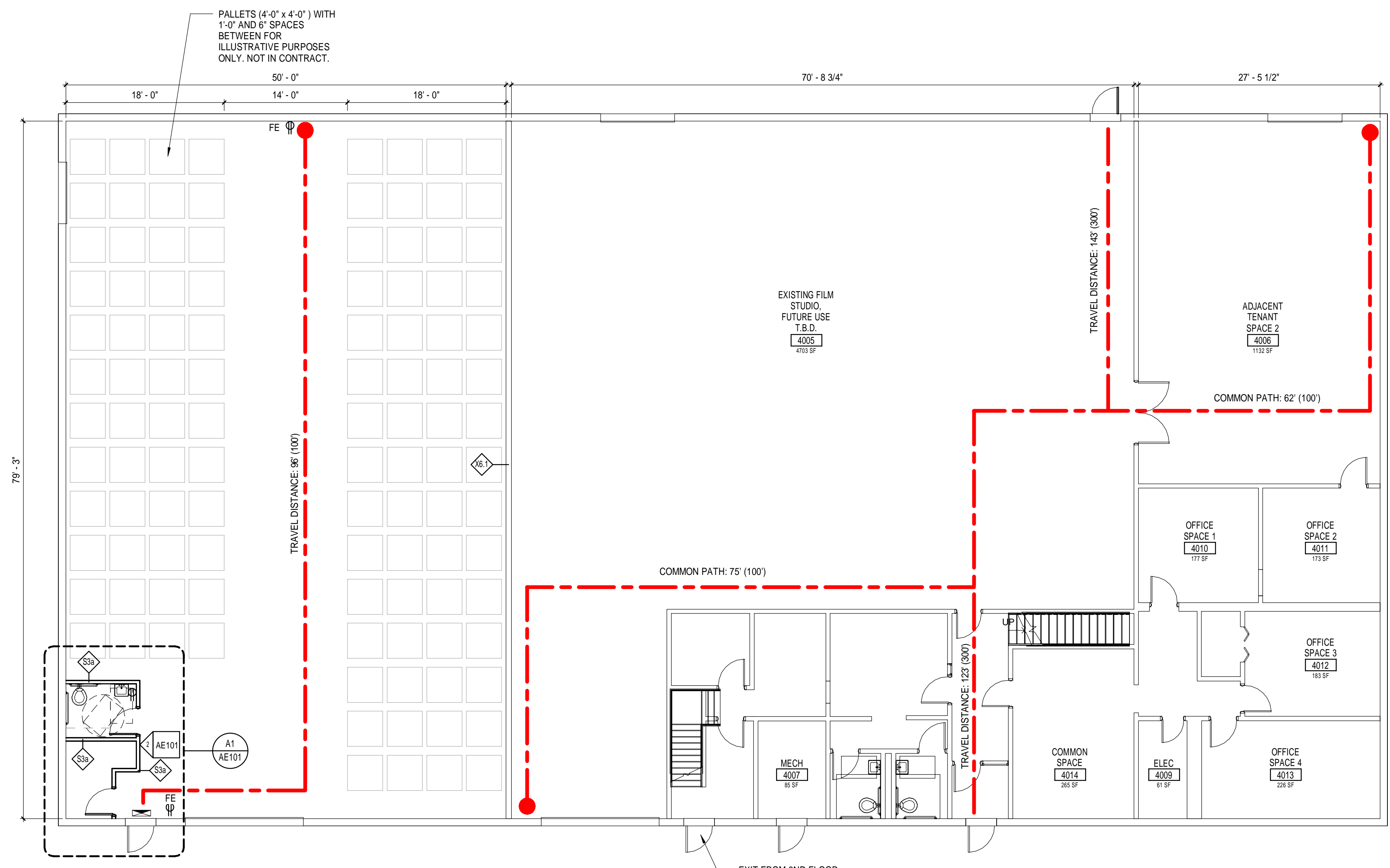
A5 FIRST FLOOR
