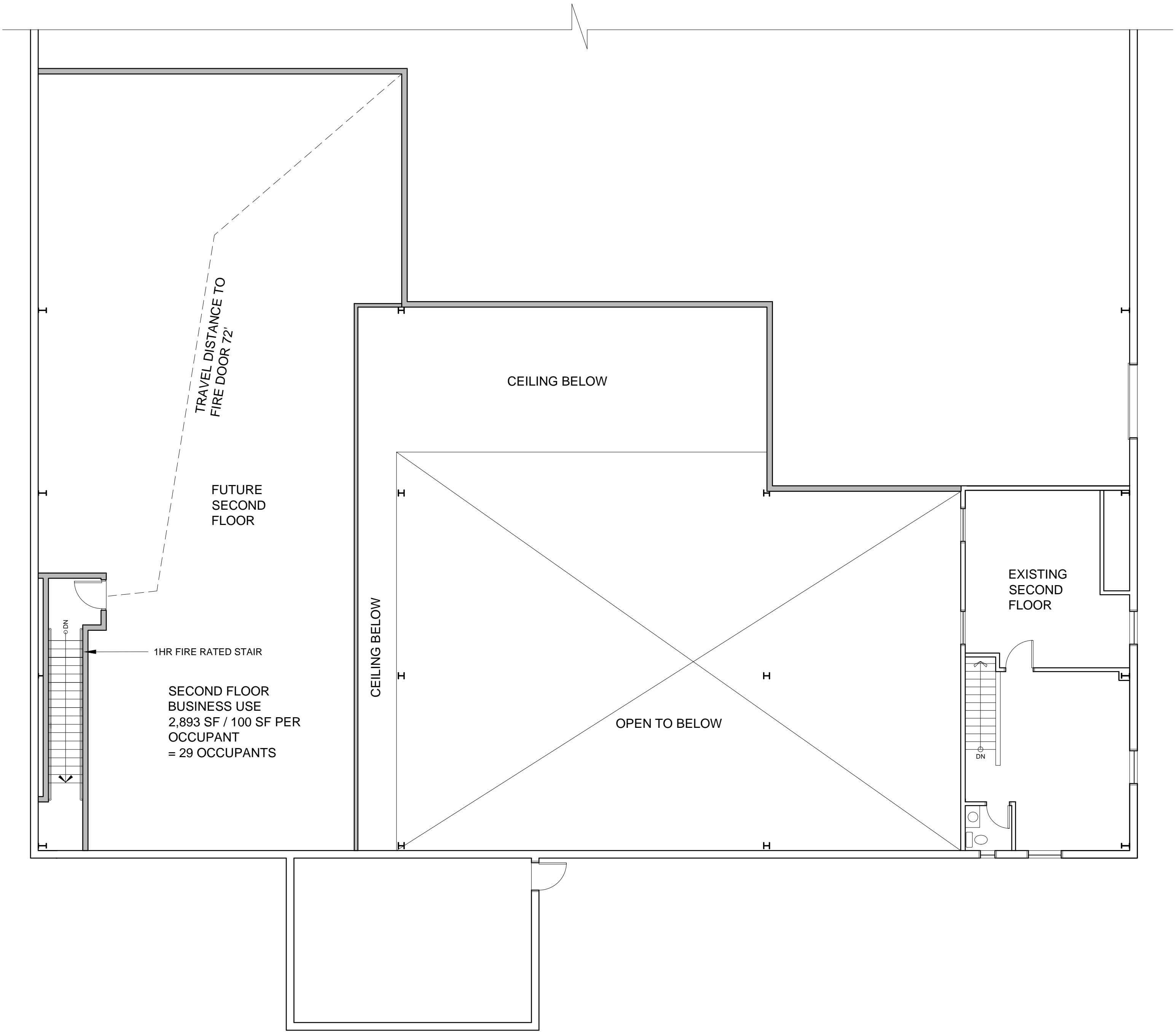
1 SECOND FLOOR PLAN 1/8" = 1'-0"
