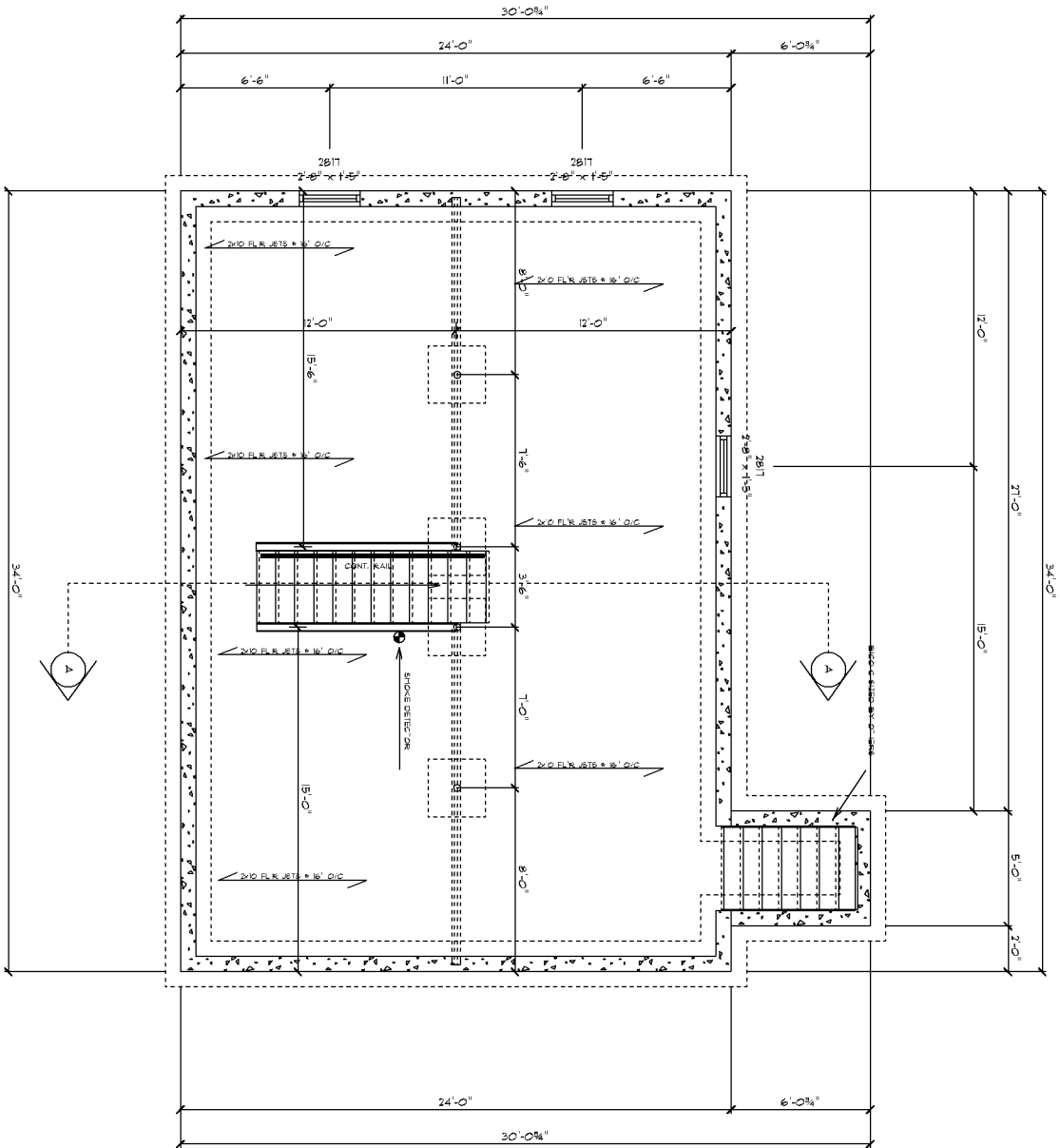
FOUNDATION PLAN
