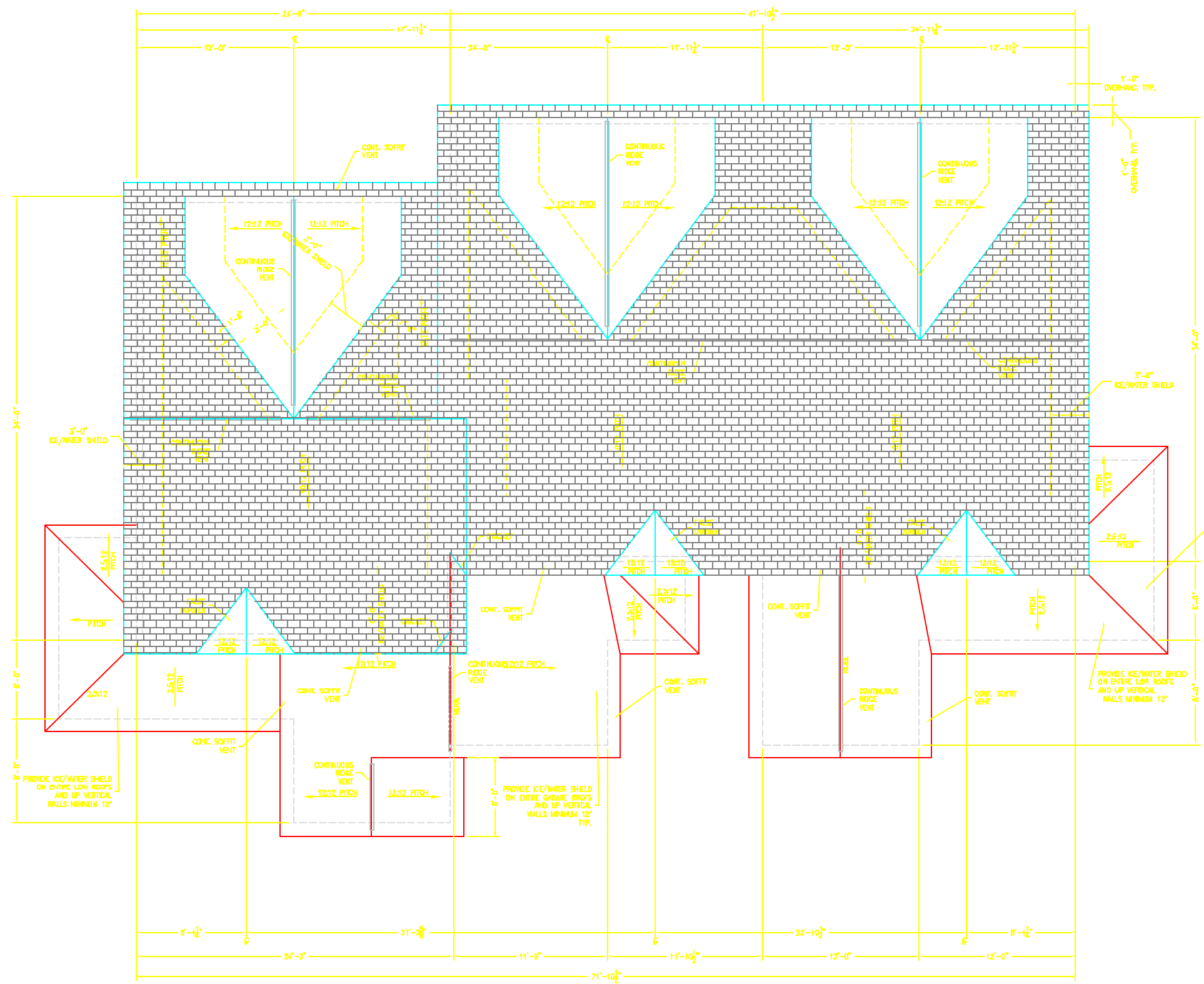
ROOF PLAN 1/4"=1'-0"
