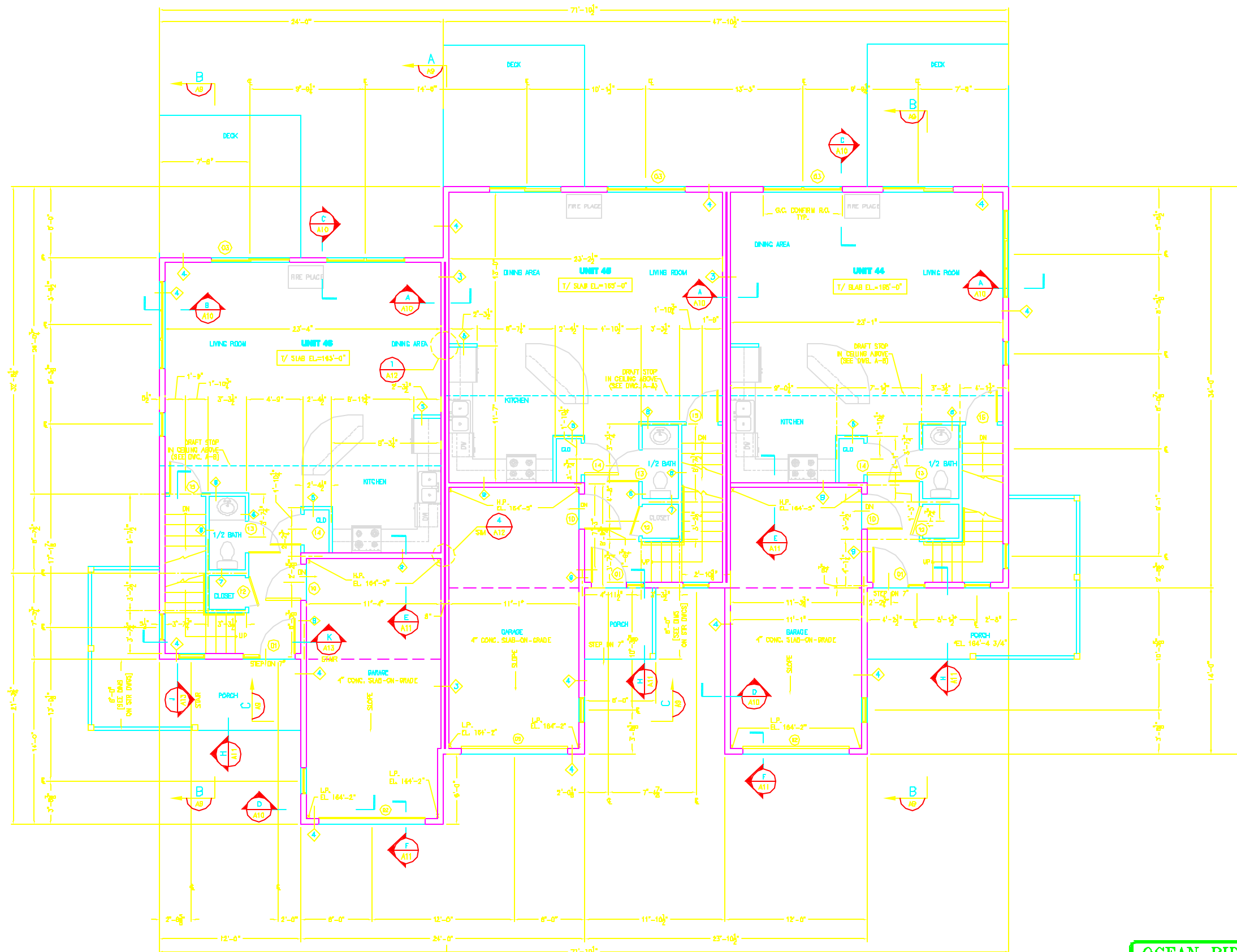
FIRST FLOOR PLAN 1/4"=1'-0"
