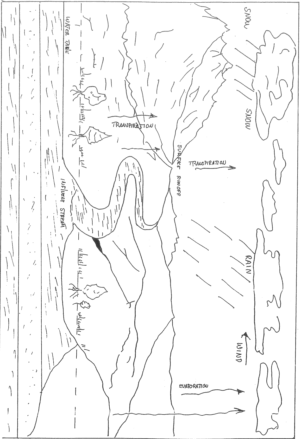
IDEALIZED Hydrologic Cycle
