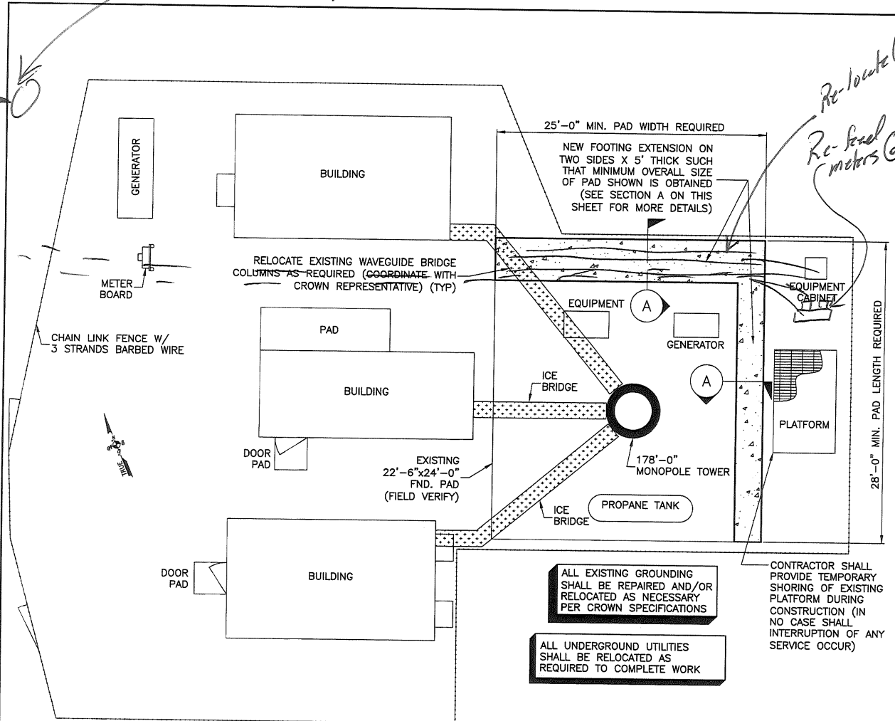
ENLARGED SITE PLAN SCALE: 1/8" = 1'-0"
