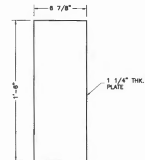
TRANSFER PLATE SIDE VIEW
