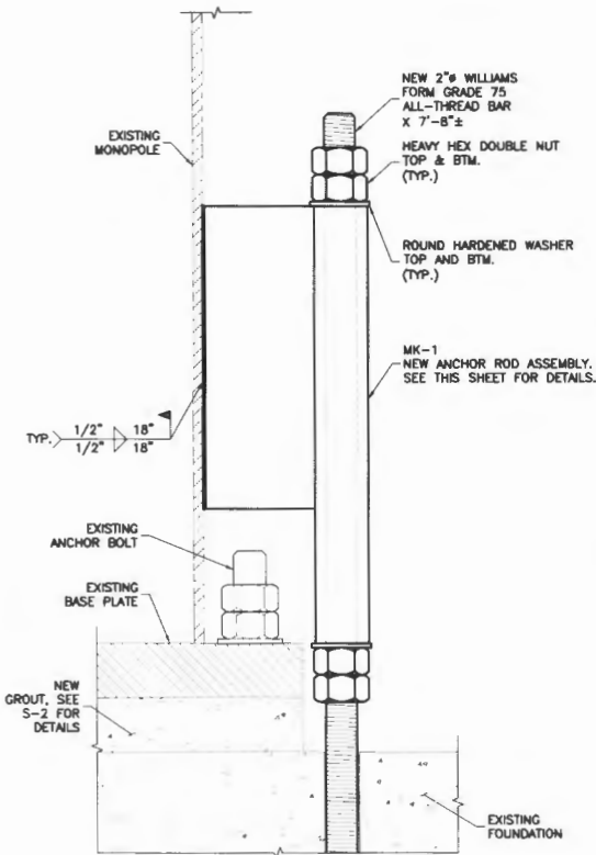
ANCHOR ROD ASSEMBLY WELD DETAIL ELEVATION VIEW
