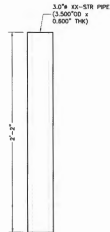
ANCHOR ROD SLEEVE SIDE VIEW
