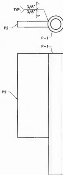
ANCHOR ROD ASSEMBLY TOP & SIDE VIEW
