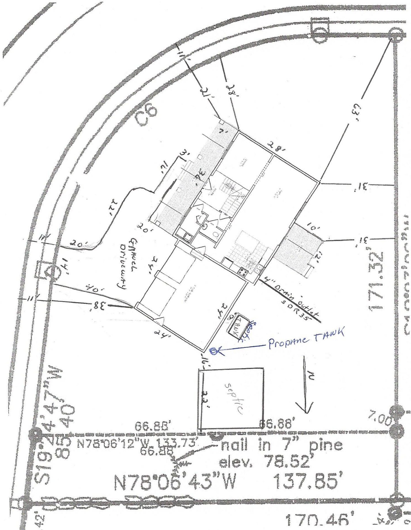
Plot Plan - Gervais
