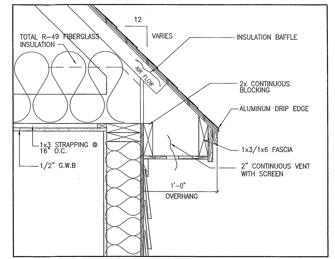
① EAVE DETAIL SCALE: 1 1/2" = 1'-0"
