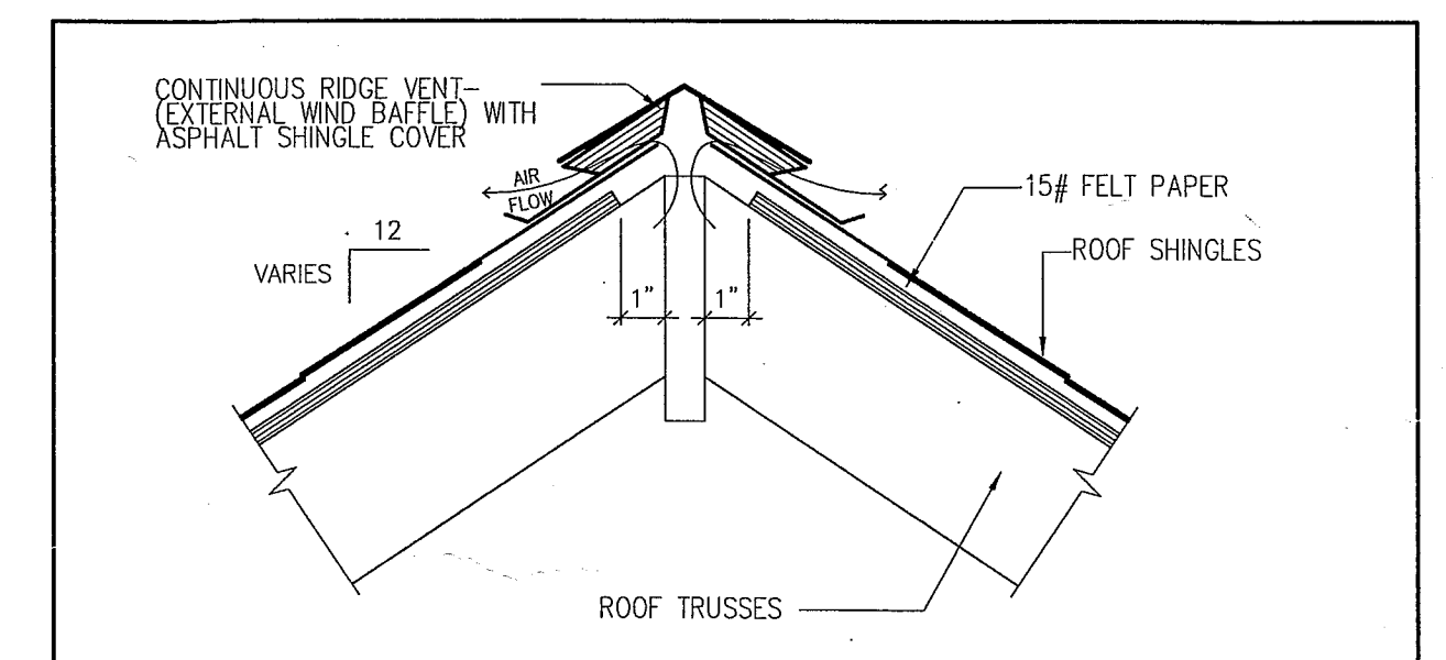
② RIDGE VENT DETAIL SCALE: 1 1/2" = 1'-0"
