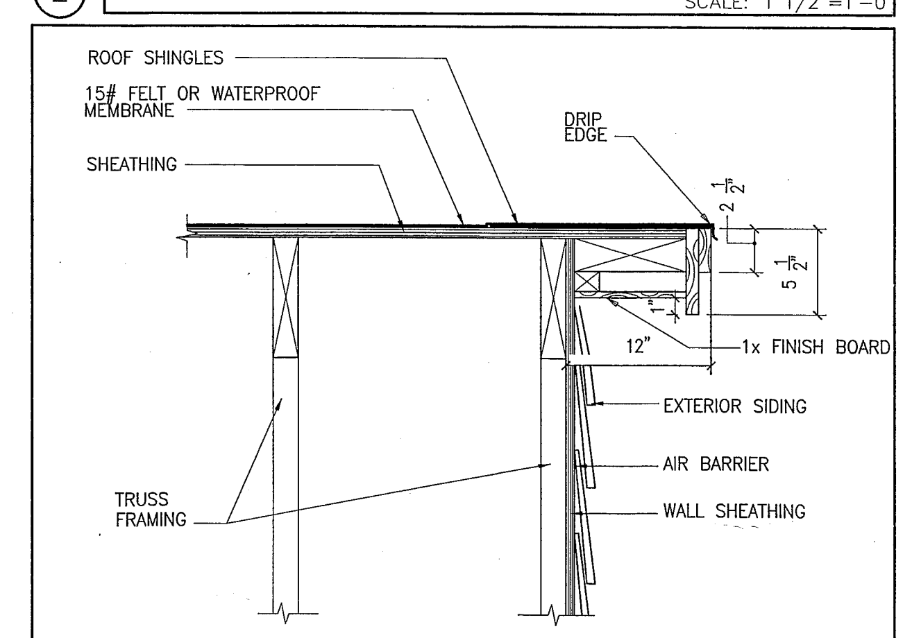
③ RAKE DETAIL SCALE: 1 1/2" = 1'-0"
