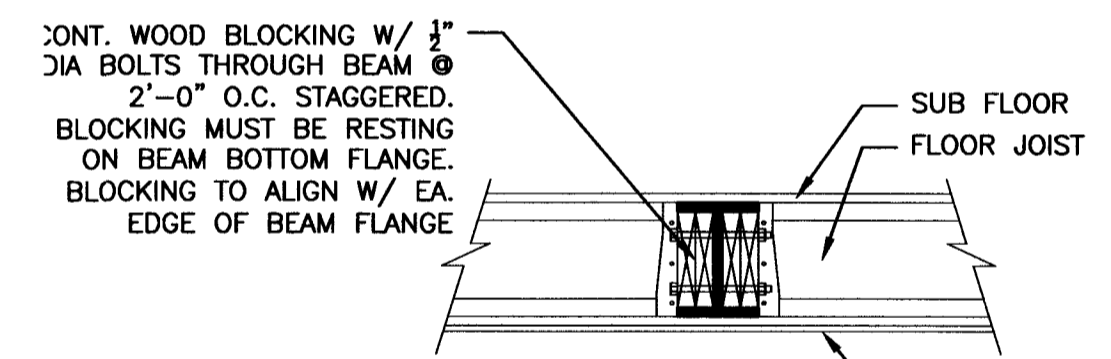
2 TYP. FLUSH FRAMED JOIST-TO-STEEL BEAM 3/8" = 1'-0"
