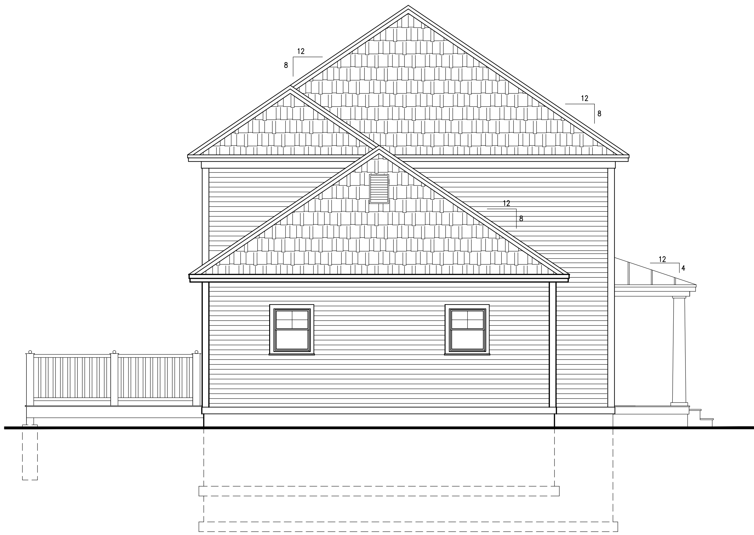
LEFT ELEVATION 1/4"=1'-0"
