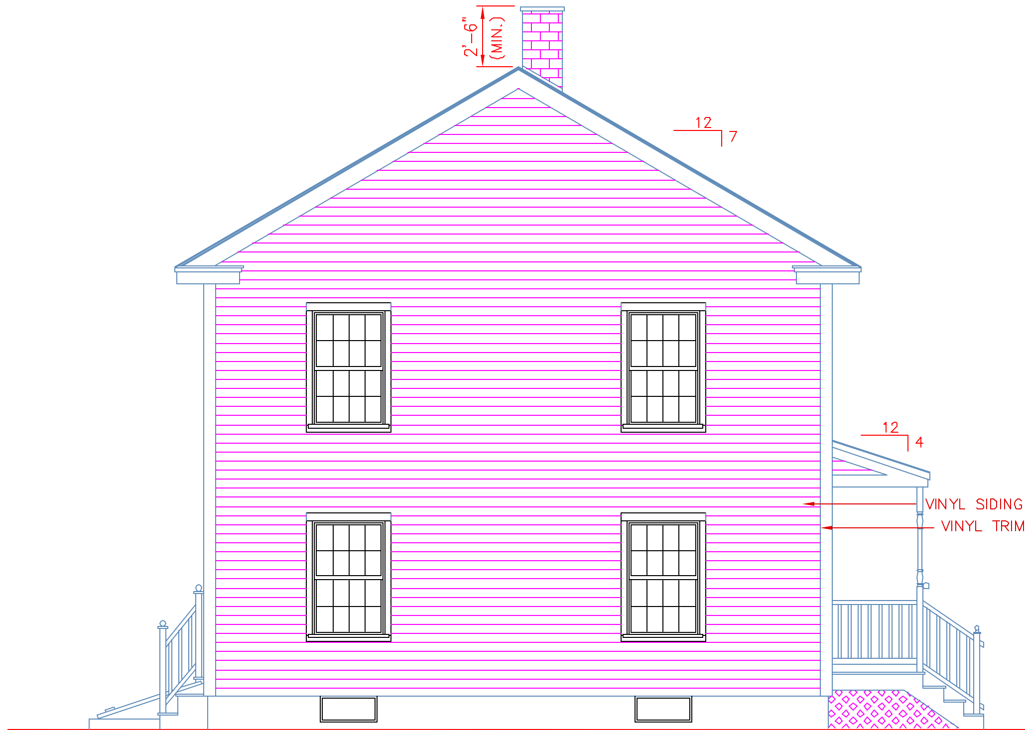
LEFT ELEVATION
