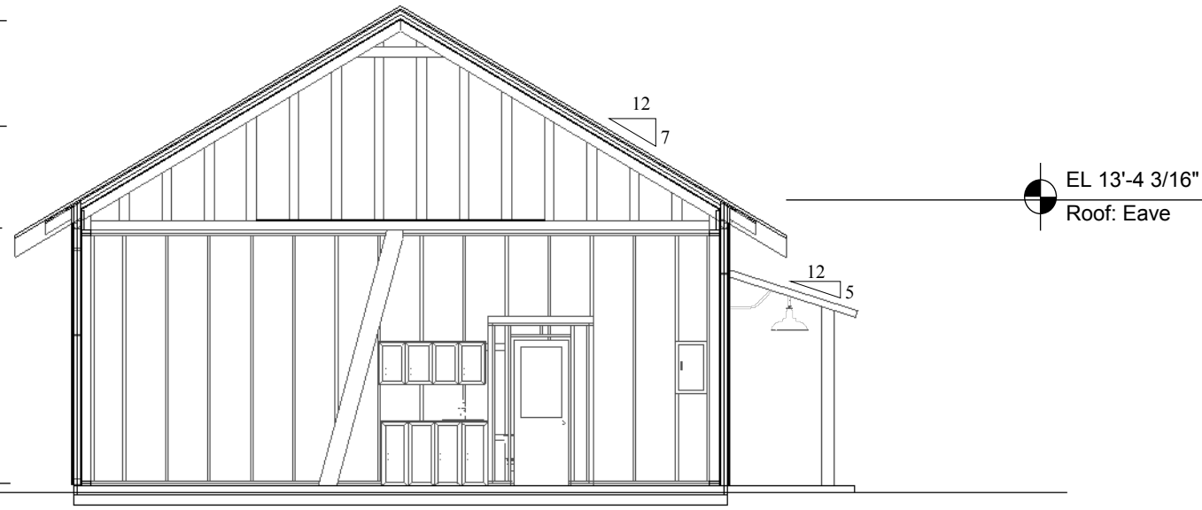
1 Building Section: East to West A6.1 Scale: 1/8" : 1'
