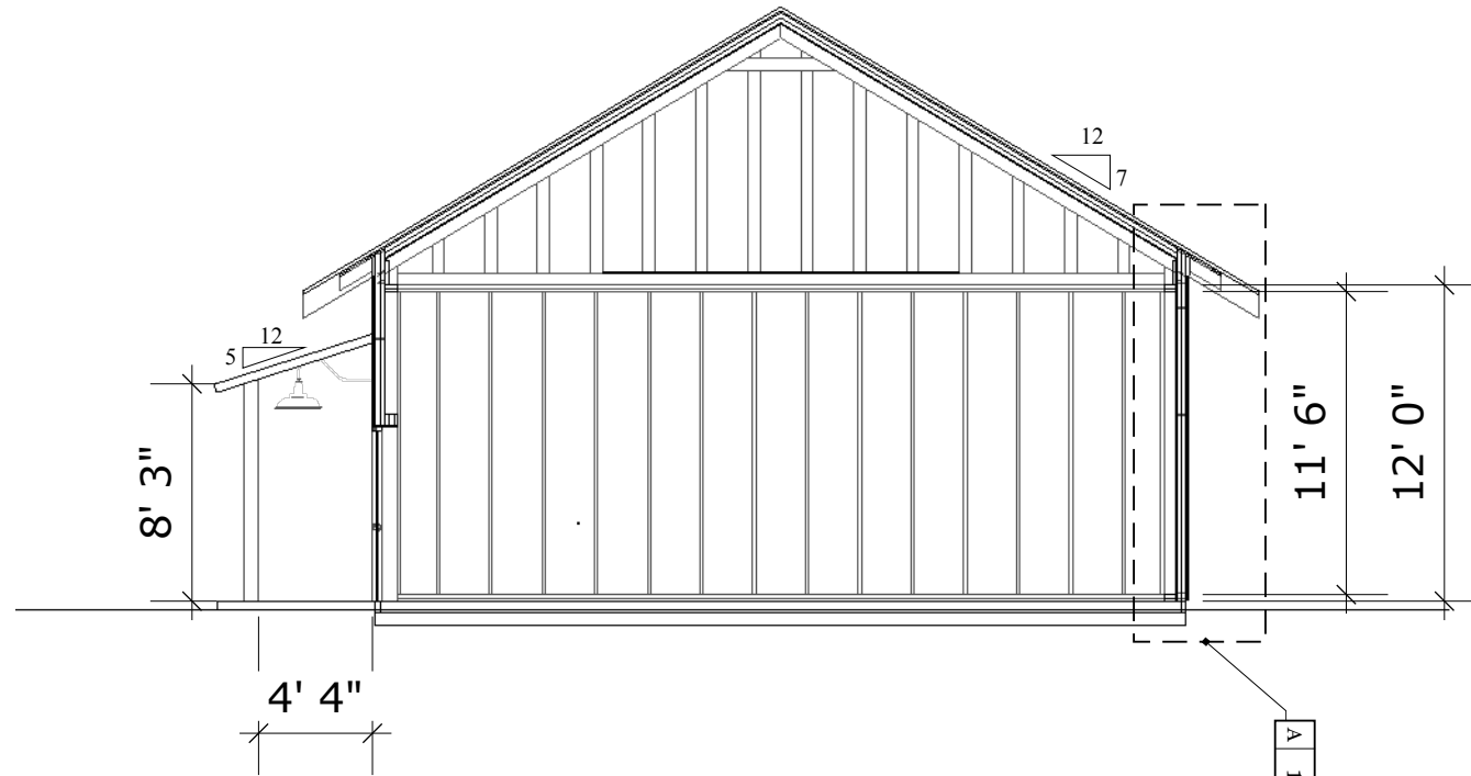
2 Building Section: West to East A6.1 Scale: 1/8" : 1'
