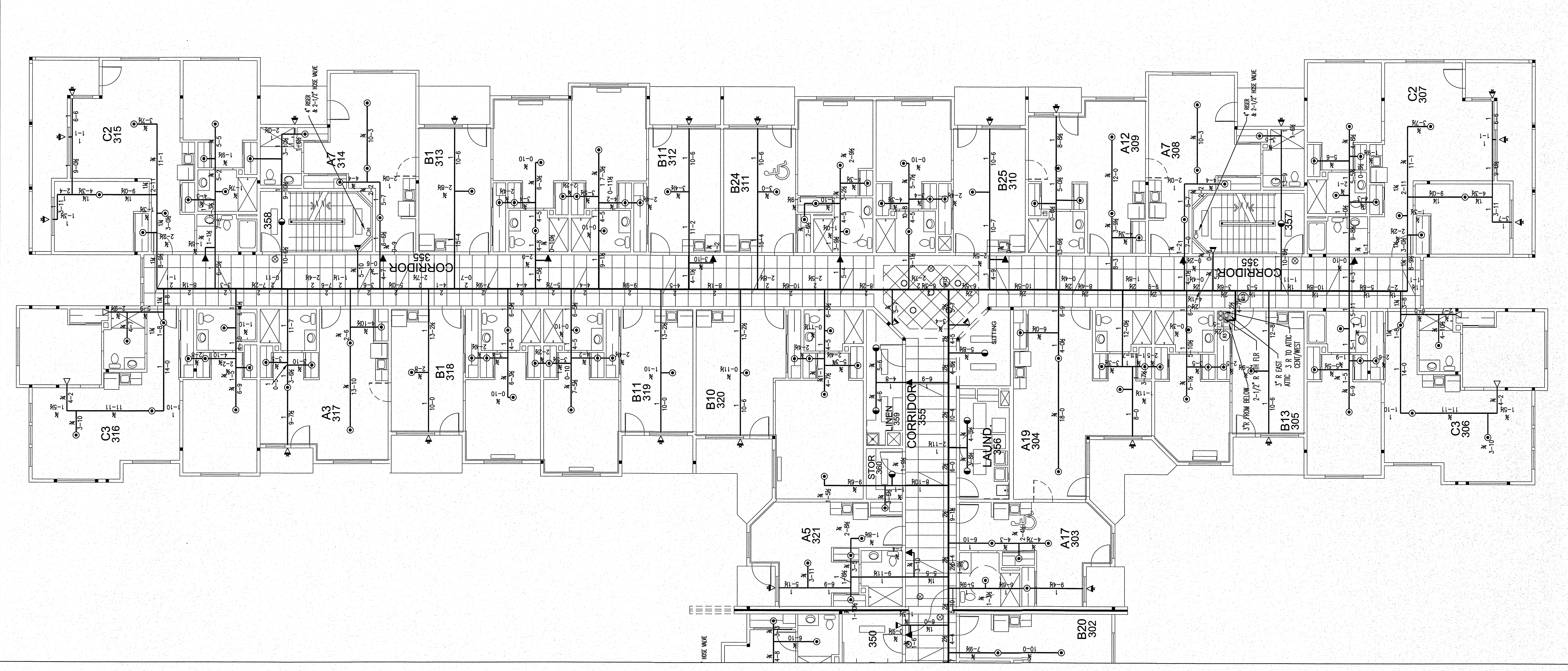
3rd FLOOR EAST PLAN SCALE: 1/8" = 1'-0"
