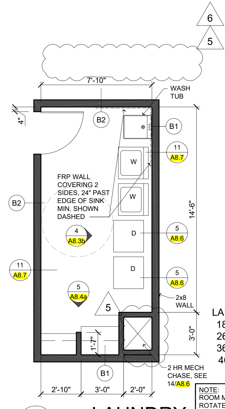
8 LAUNDRY SCALE: 1/4"=1'-0"
