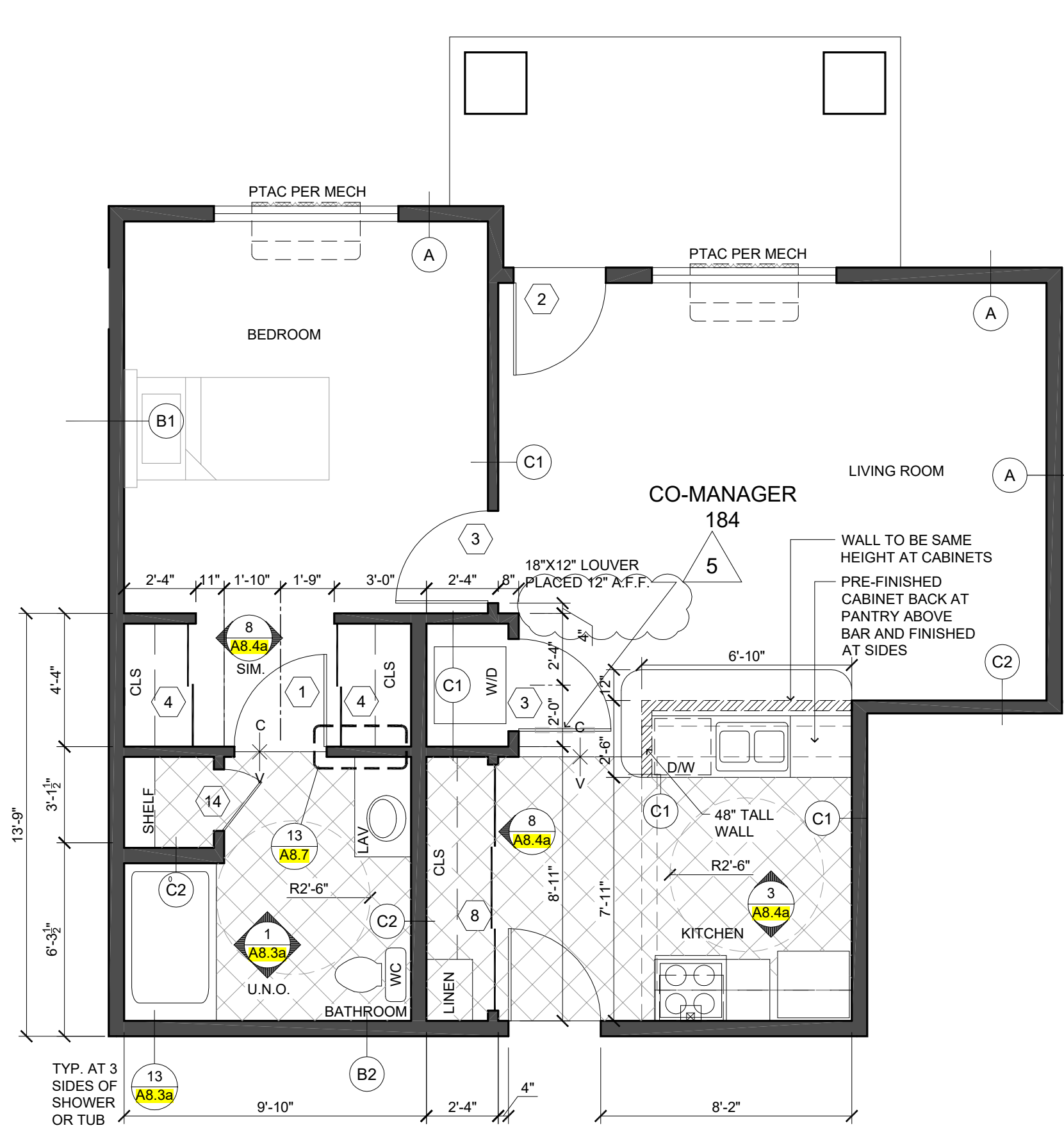
3 CO-MANAGER SCALE: 1/4"=1'-0"
