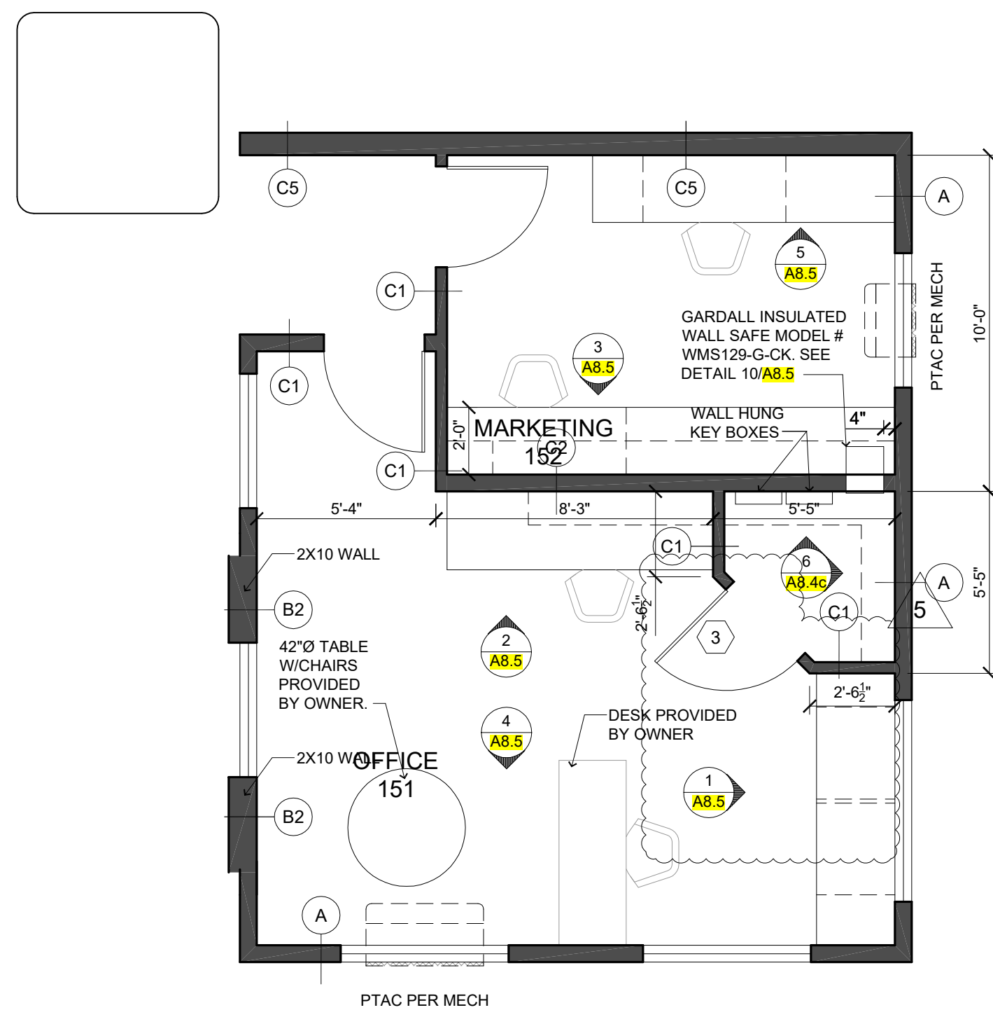
1 OFFICE / MARKETING SCALE: 1/4"=1'-0"
