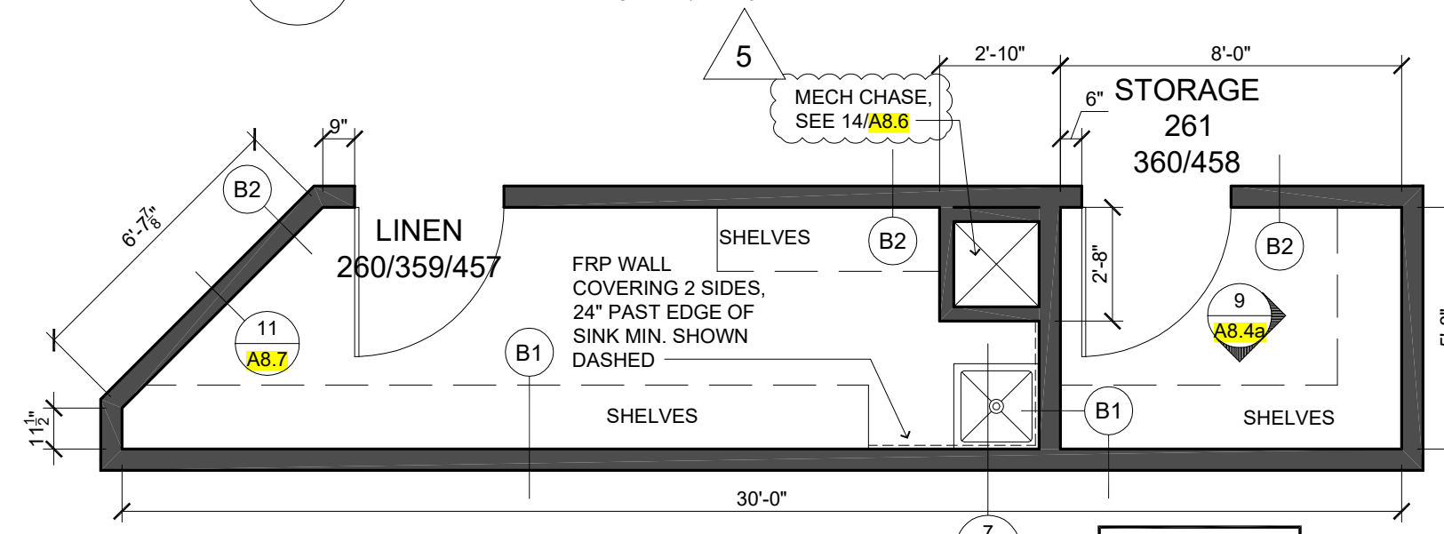
7 LINEN/STORAGE SCALE: 1/4"=1'-0"
