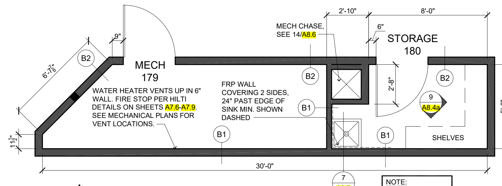
13 MECH/STORAGE SCALE: 1/4"=1'-0"
