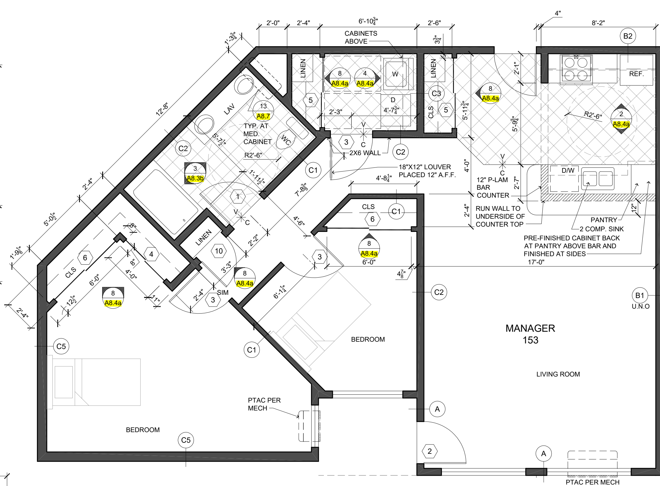
2 MANAGER SCALE: 1/4"=1'-0"
