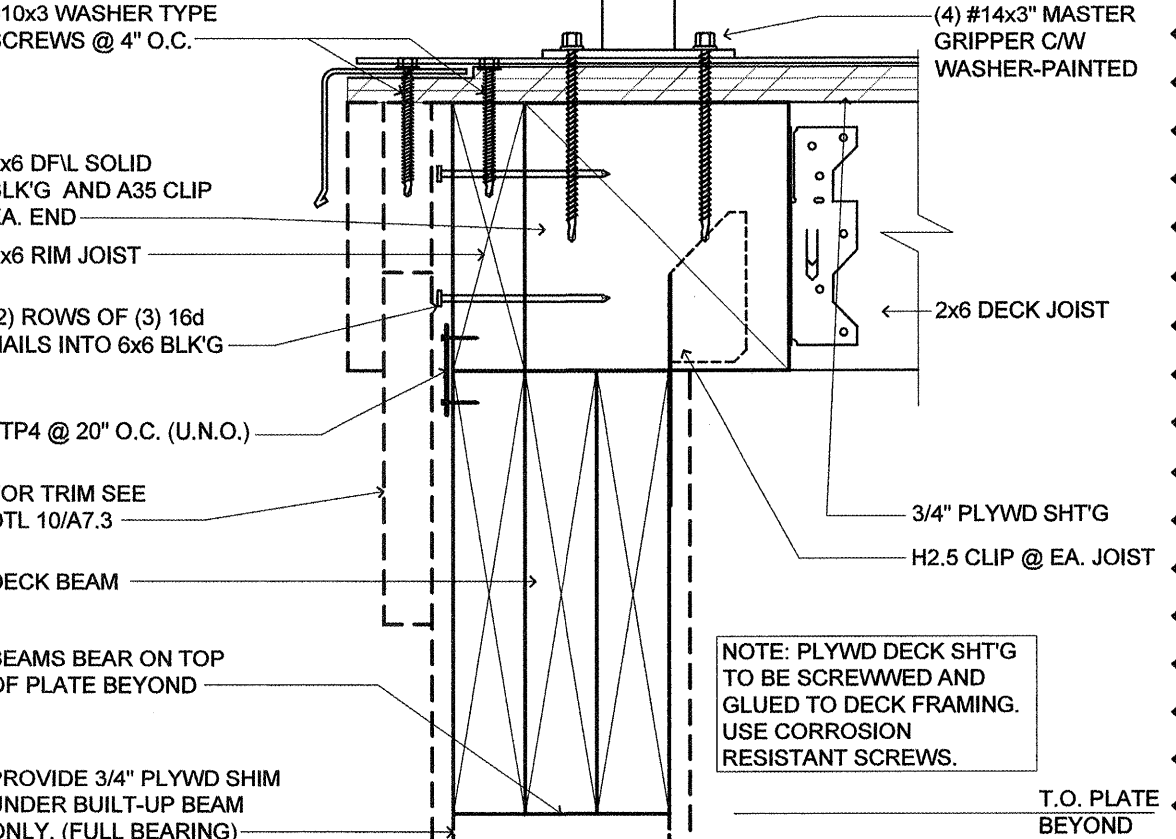
6 DECK FRAMING (DECK BEAM) SCALE: 3" = 1'-0"
