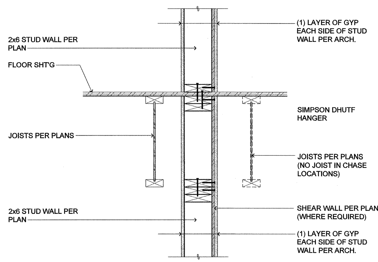
16 1 HOUR SEPARATION (NON-LOAD BEARING PARALLEL TO WALL) SCALE: 1" = 1'-0"
