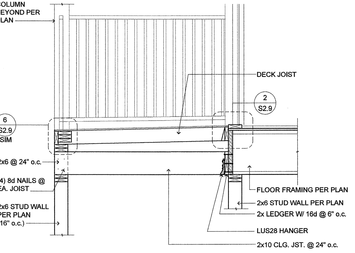
8 DECK FRAMING (ABOVE HVAC/ELEV. EQ. RM.) SCALE: 1/2" = 1'-0"
