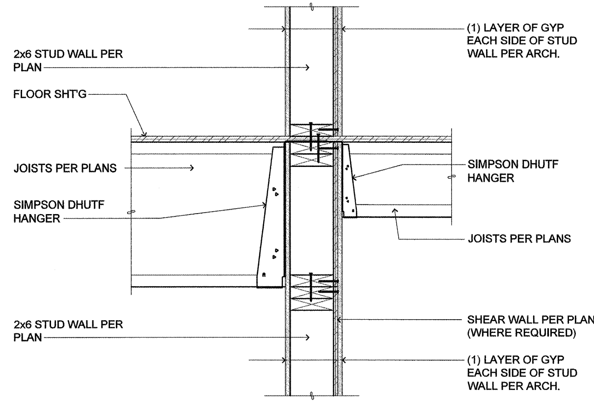
15 1 HOUR SEPARATION (LOAD BEARING PERP. TO JOIST) SCALE: 1" = 1'-0"
