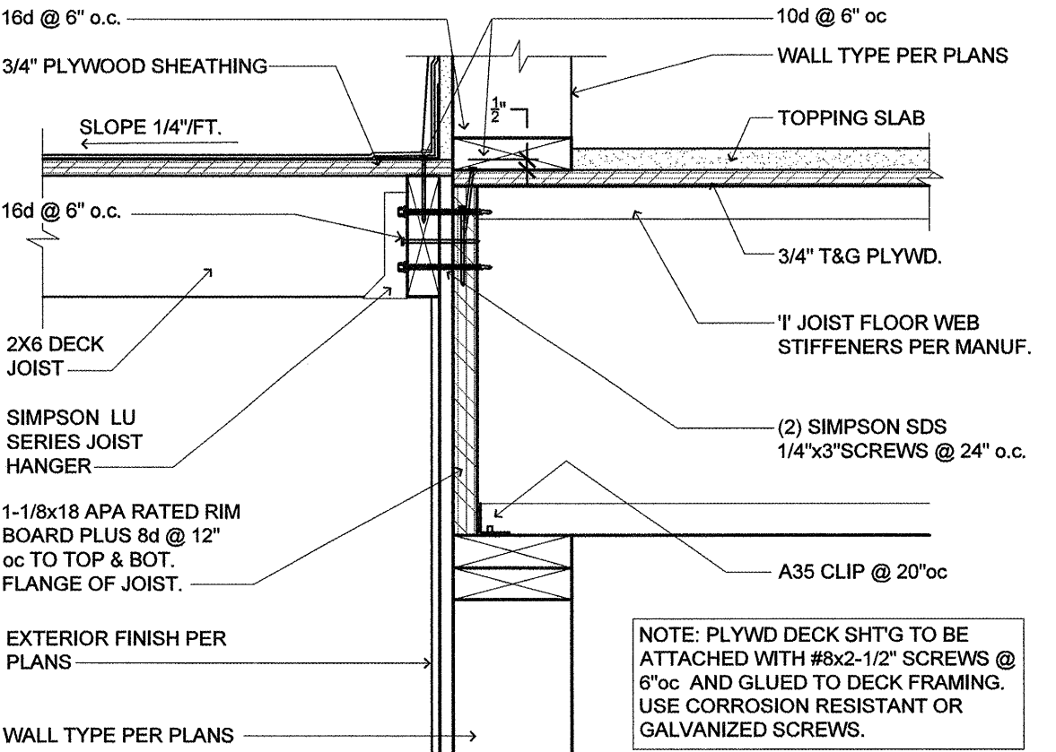
2 DECK FRAMING (DECK-WALL INTERSECTION) SCALE: 1 1/2" = 1'-0"
