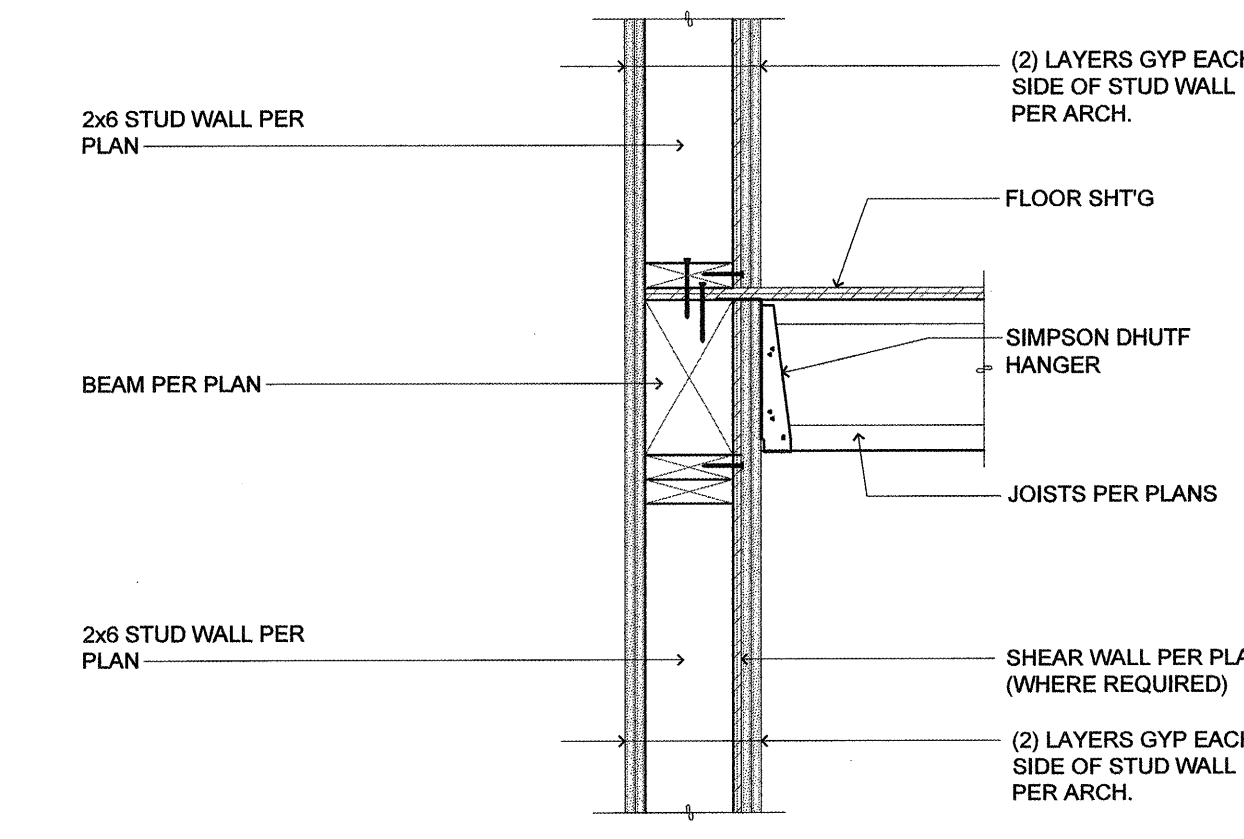
18 2 HOUR SEPARATION (LOAD BEARING - AT MIDLANDING) SCALE: 1" = 1'-0"
