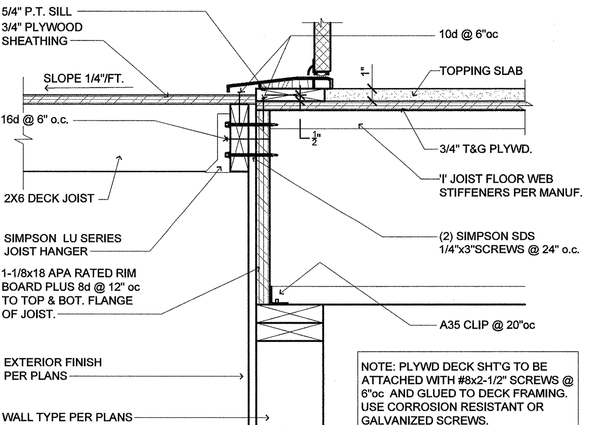
1 DECK FRAMING (DECK AT THRESHOLD) SCALE: 1 1/2" = 1'-0"
