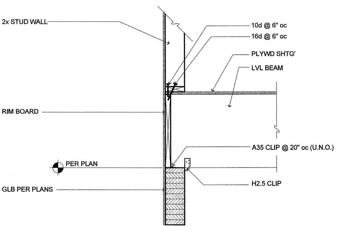
9 CONNECTION DETAIL SCALE: 3/4" = 1'-0"
