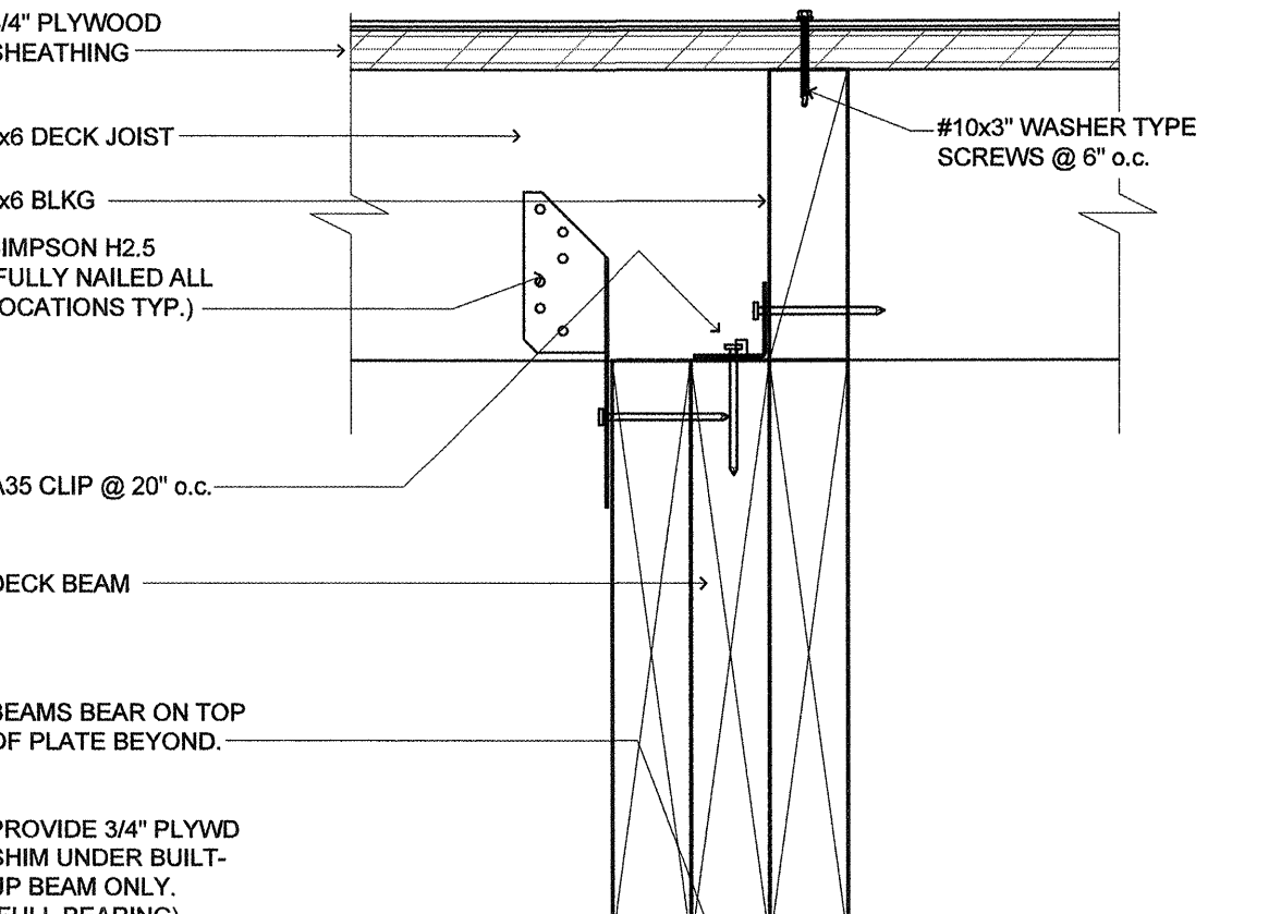
5 DECK FRAMING (DECK BEAM) SCALE: 3" = 1'-0"
