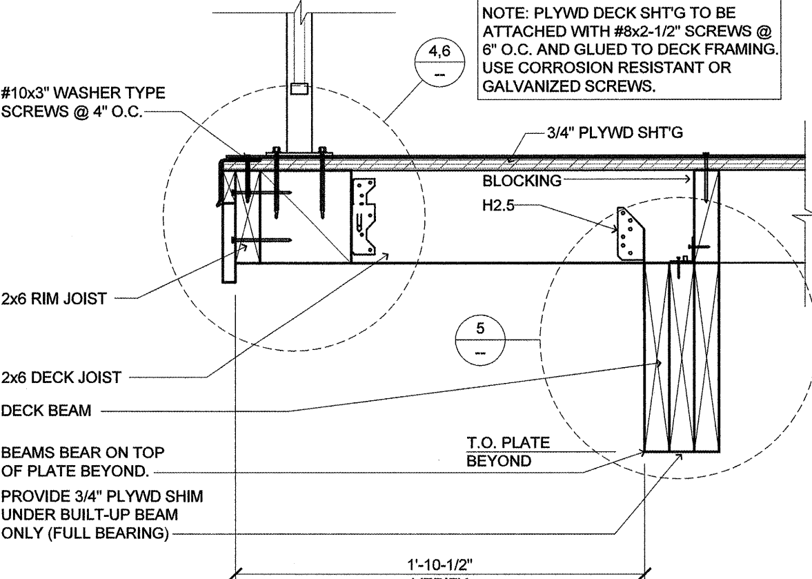
3 DECK FRAMING (DECK EDGE) SCALE: 1 1/2" = 1'-0"
