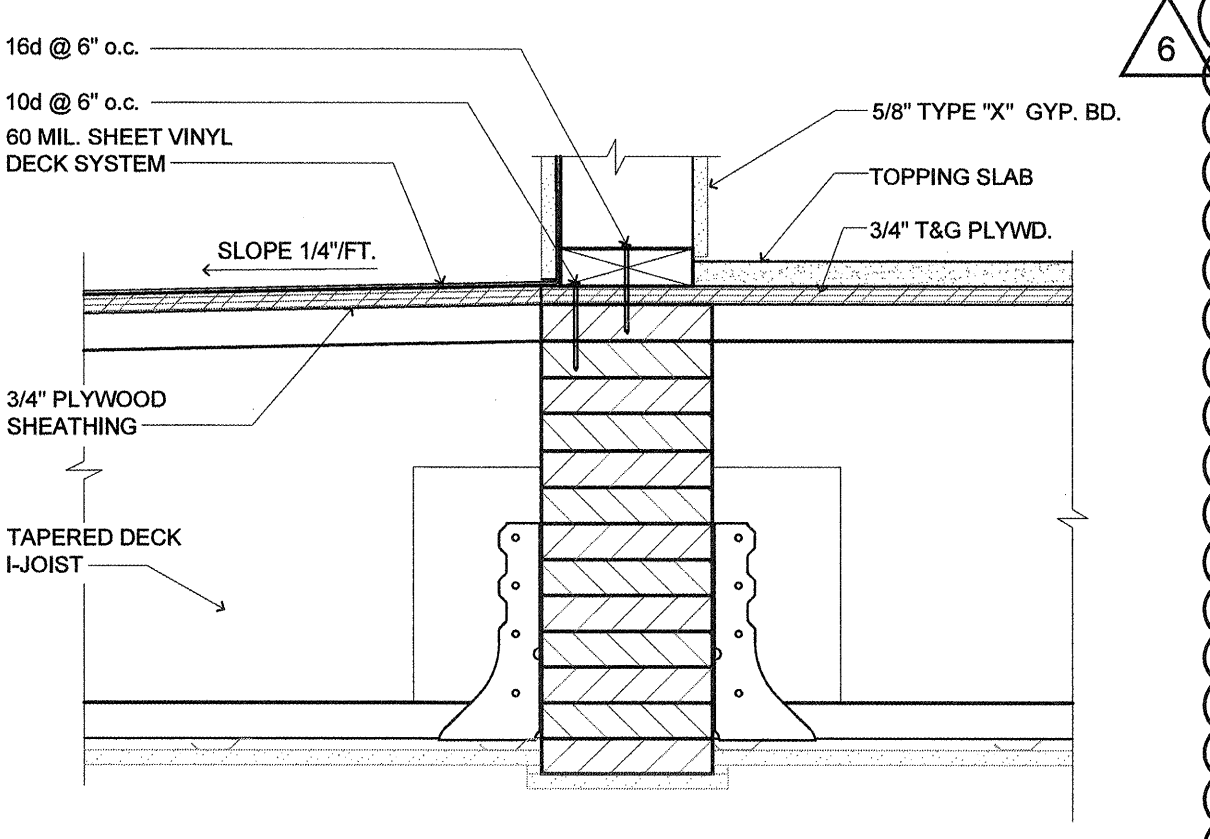
11 DECK-WALL INTERSECTION (SOFFIT ON UNDERSIDE OF DECK) SCALE: 1 1/2" = 1'-0"
