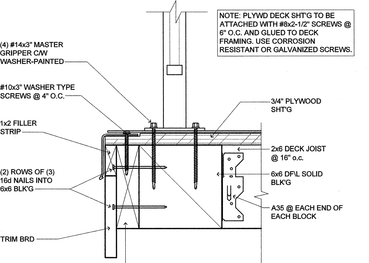
4 DECK FRAMING (DECK EDGE) SCALE: 3" = 1'-0"
