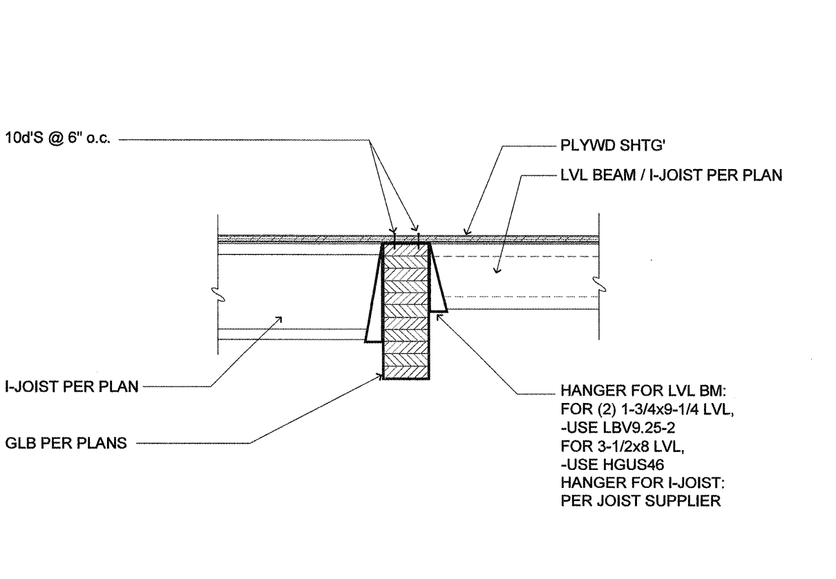
10 CONNECTION DETAIL (JOIST TO BEAM) SCALE: 3/4" = 1'-0"
