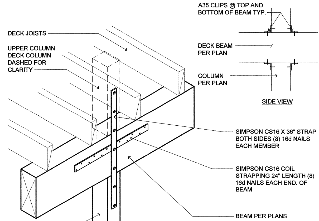
13 DECK BEAM/COLUMN INTERSECTION (TYPICAL OF WING END UNITS) SCALE: N.T.S.
