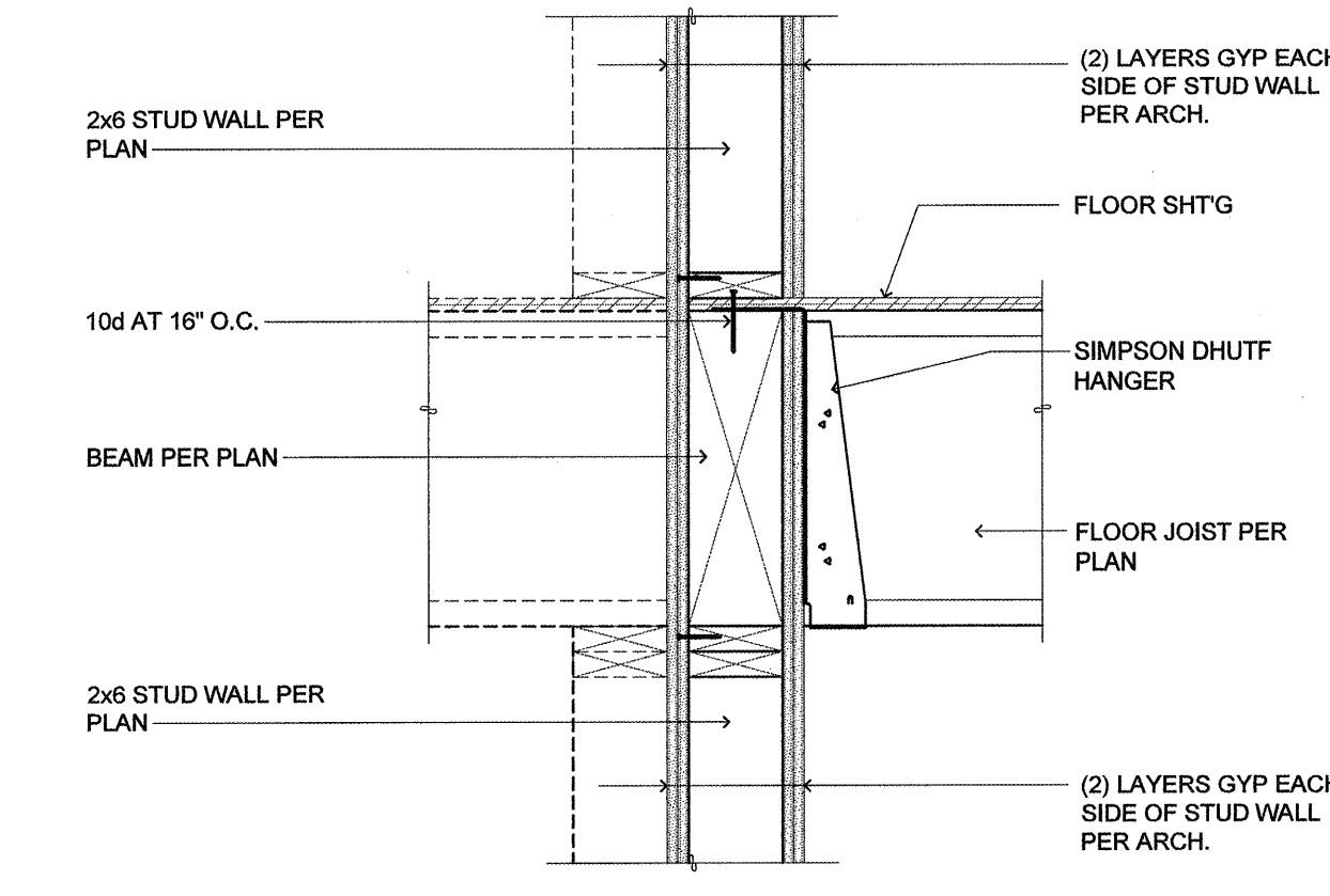
19 2 HOUR SEPARATION (LOAD BEARING) SCALE: 1" = 1'-0"
