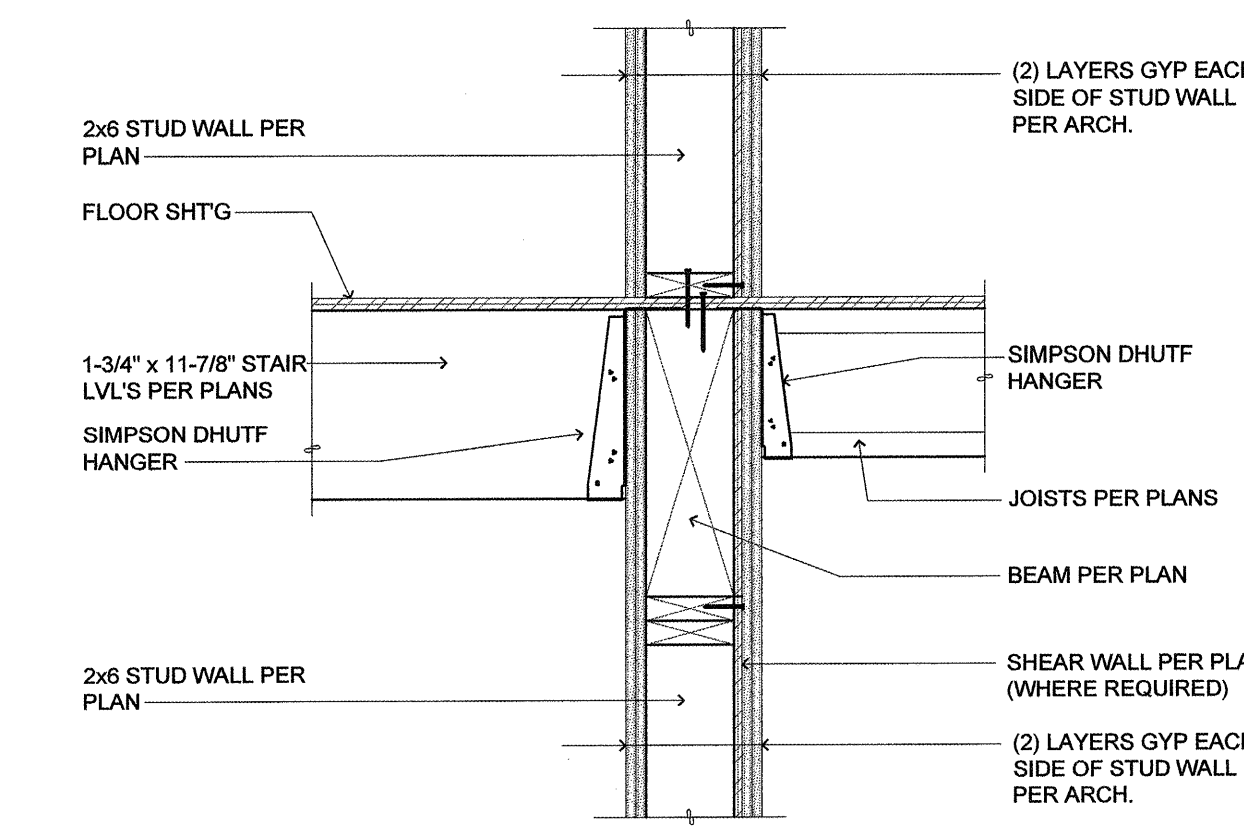
17 2 HOUR SEPARATION (LOAD BEARING PERP. TO JOIST) SCALE: 1" = 1'-0"
