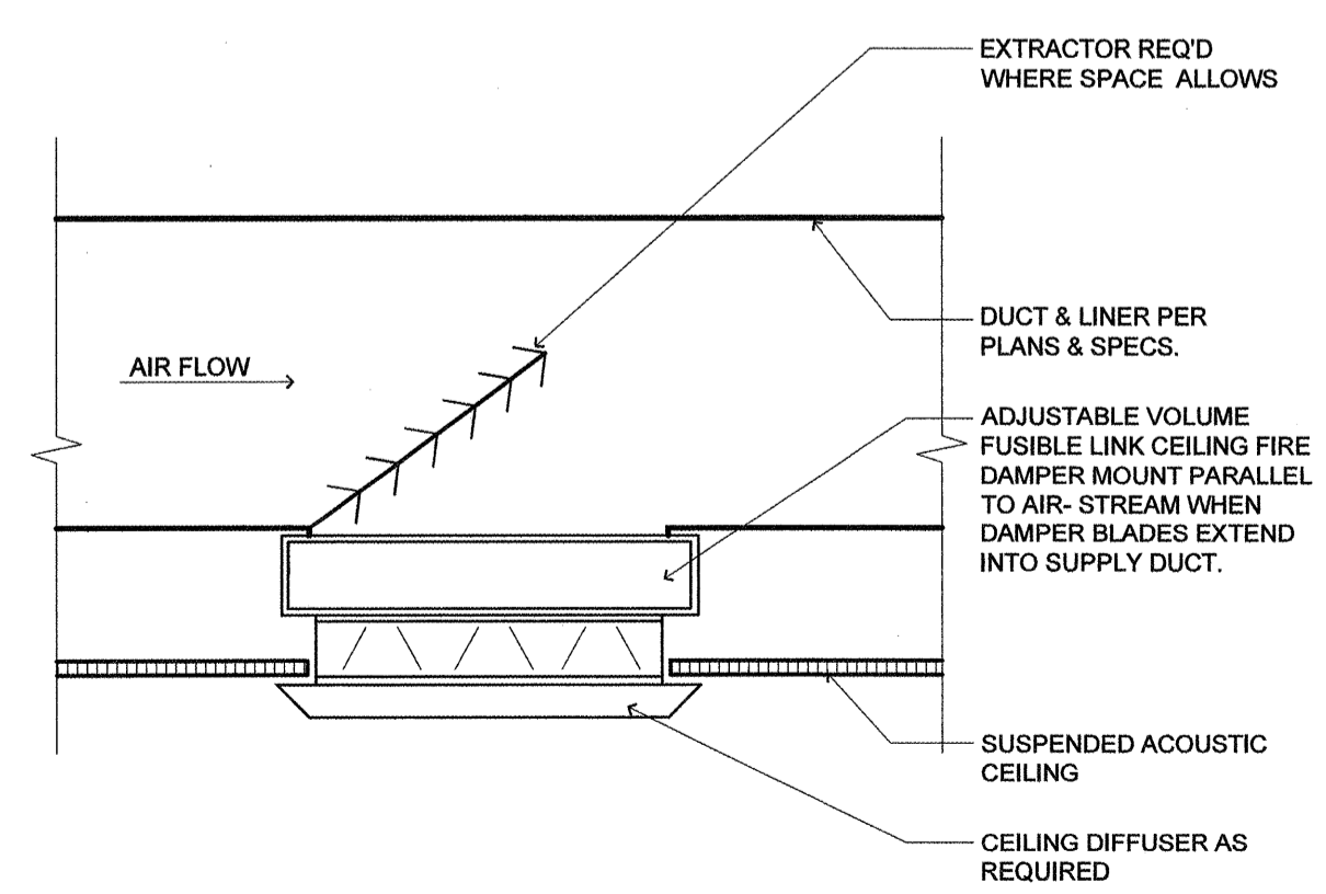
10 CEILING DIFFUSER (DUCT MOUNTED) SCALE: NOT TO SCALE
