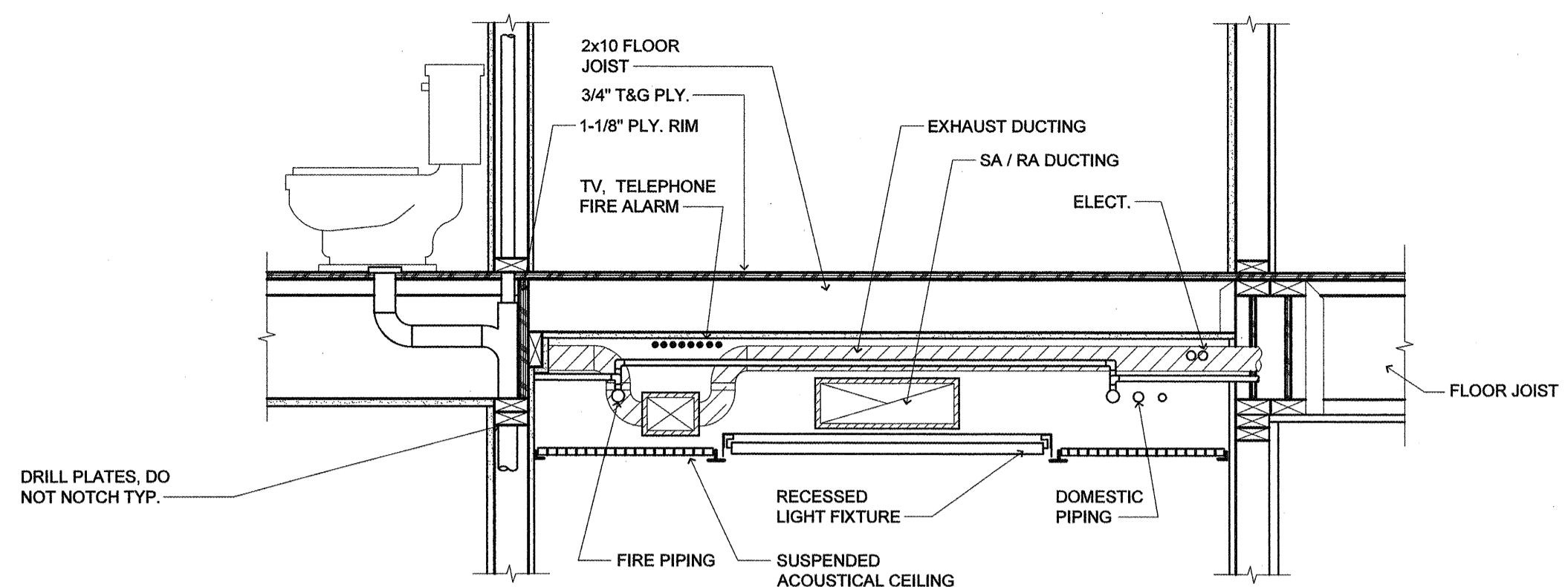
14 SCHEMATIC - SECTION AT CORRIDOR WOOD CONSTRUCTION (ALL TRADES TO COORDINATE AVAILABLE SPACE) SCALE: N.T.S.
