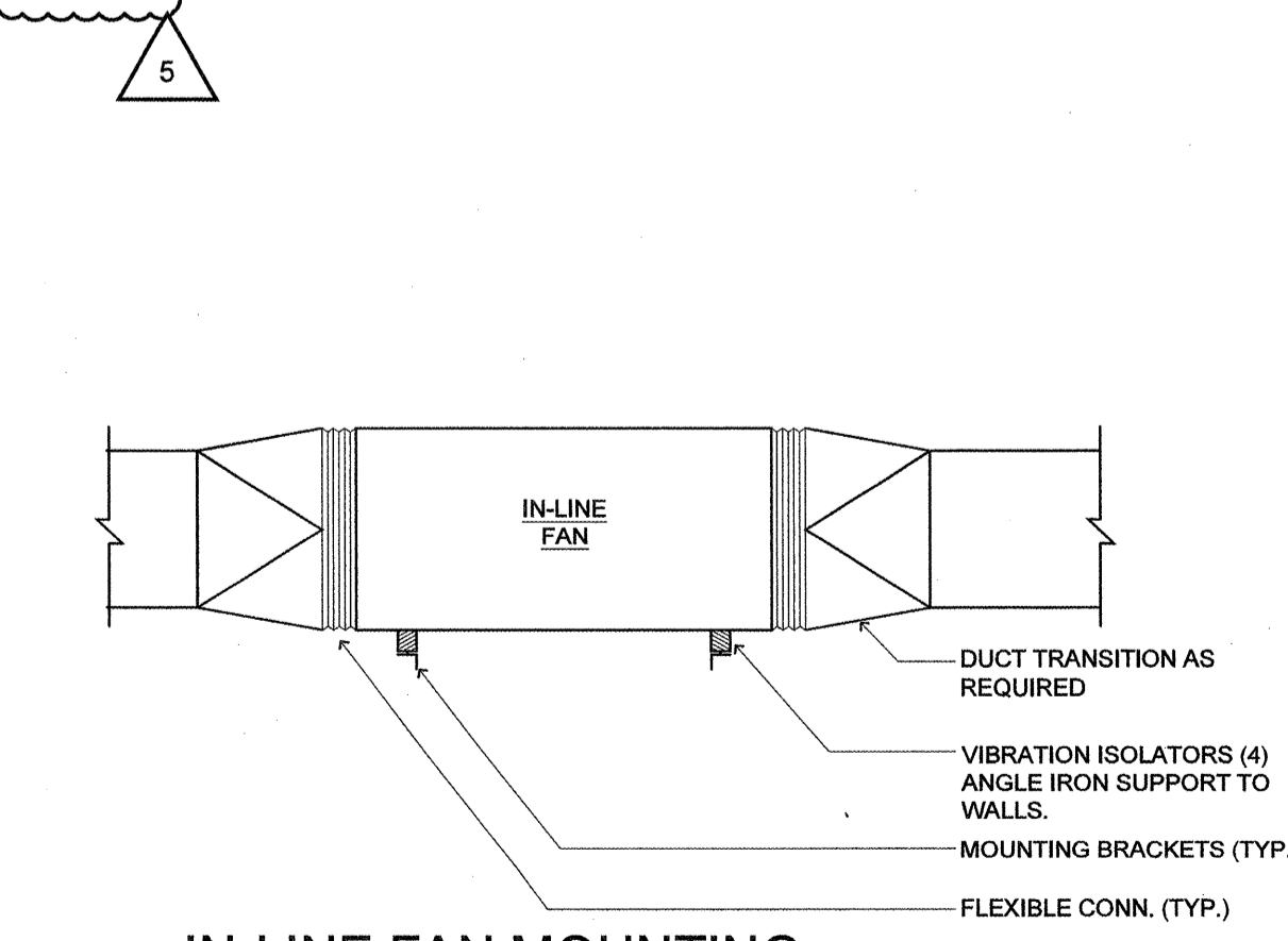
1 IN-LINE FAN MOUNTING SCALE: NOT TO SCALE (1:1)
