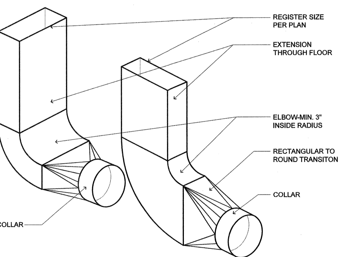
5 DUCT CONNECTION (RECTANGLE TO ROUND) SCALE: N.T.S.
