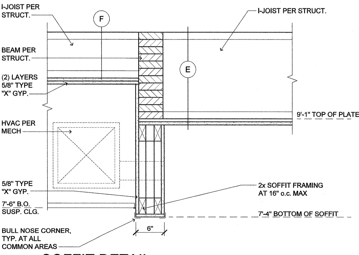
8 SOFFIT DETAIL (TV ROOM) SCALE: 1"=1'-0"
