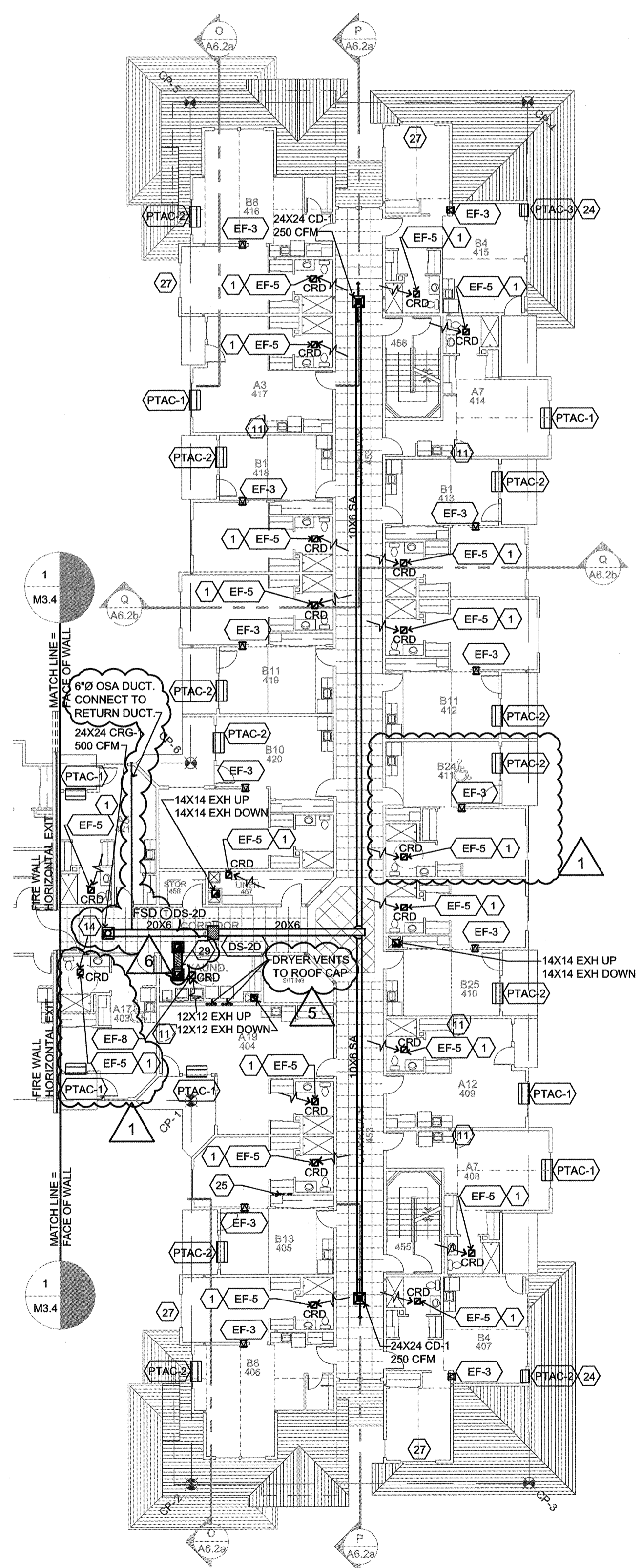
4 FOURTH FLOOR - HVAC SCALE: 1/16" = 1'-0"
