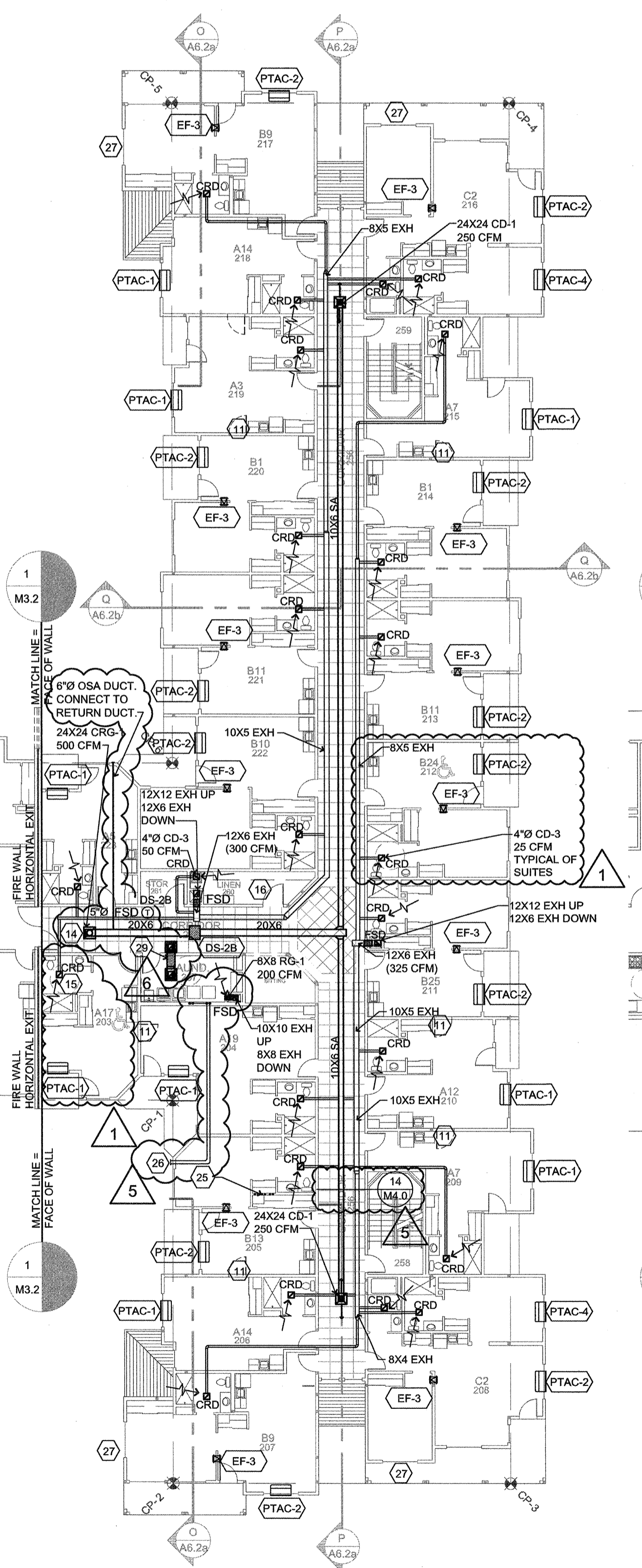
2 SECOND FLOOR - HVAC SCALE: 1/16" = 1'-0"
