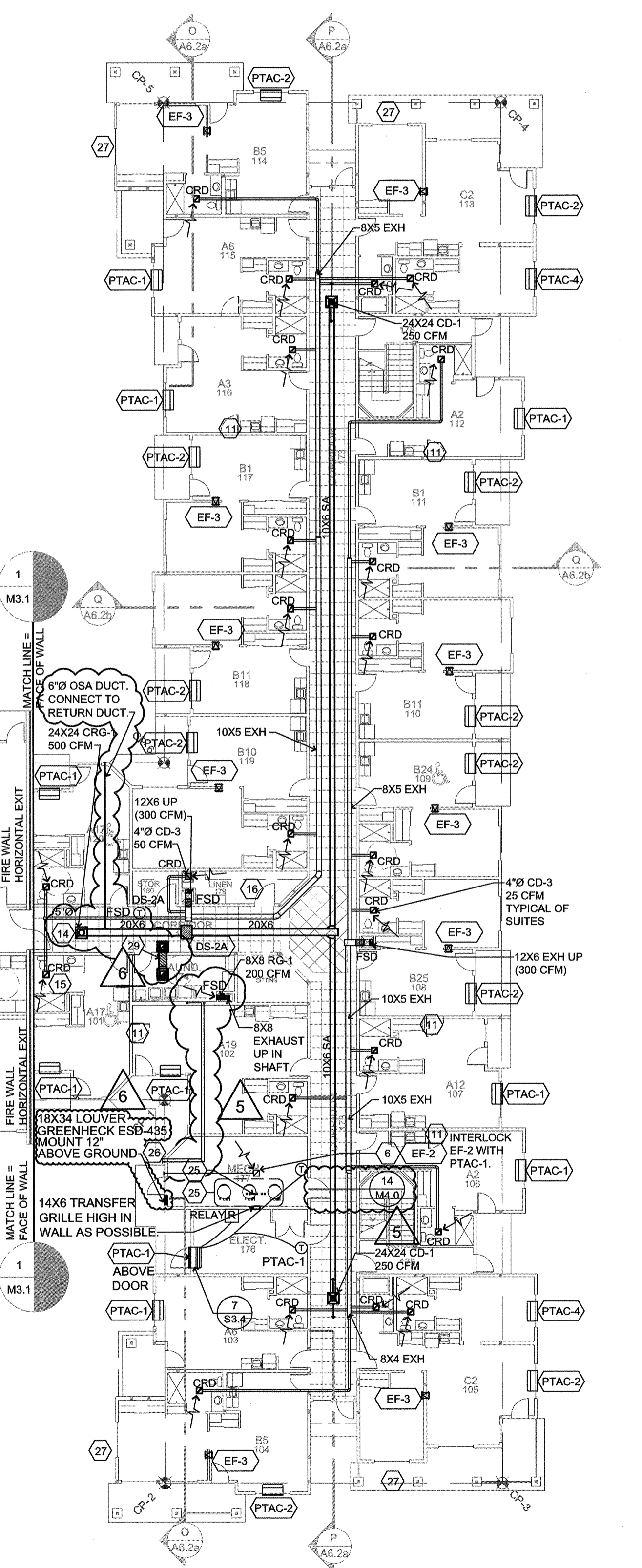
1 FIRST FLOOR - HVAC SCALE: 1/16" = 1'-0"
