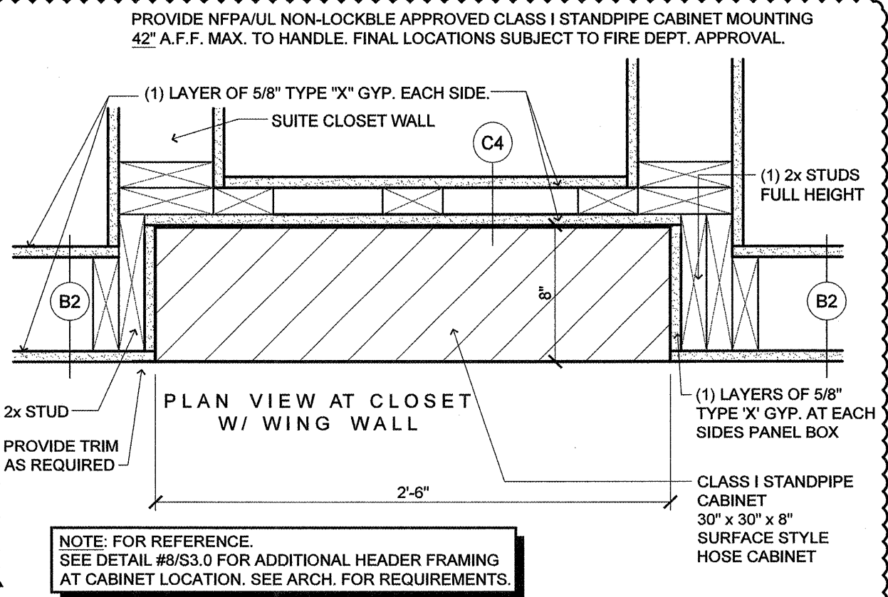
3 STANDPIPE CABINET (FIRE RATED) SCALE: N.T.S.
