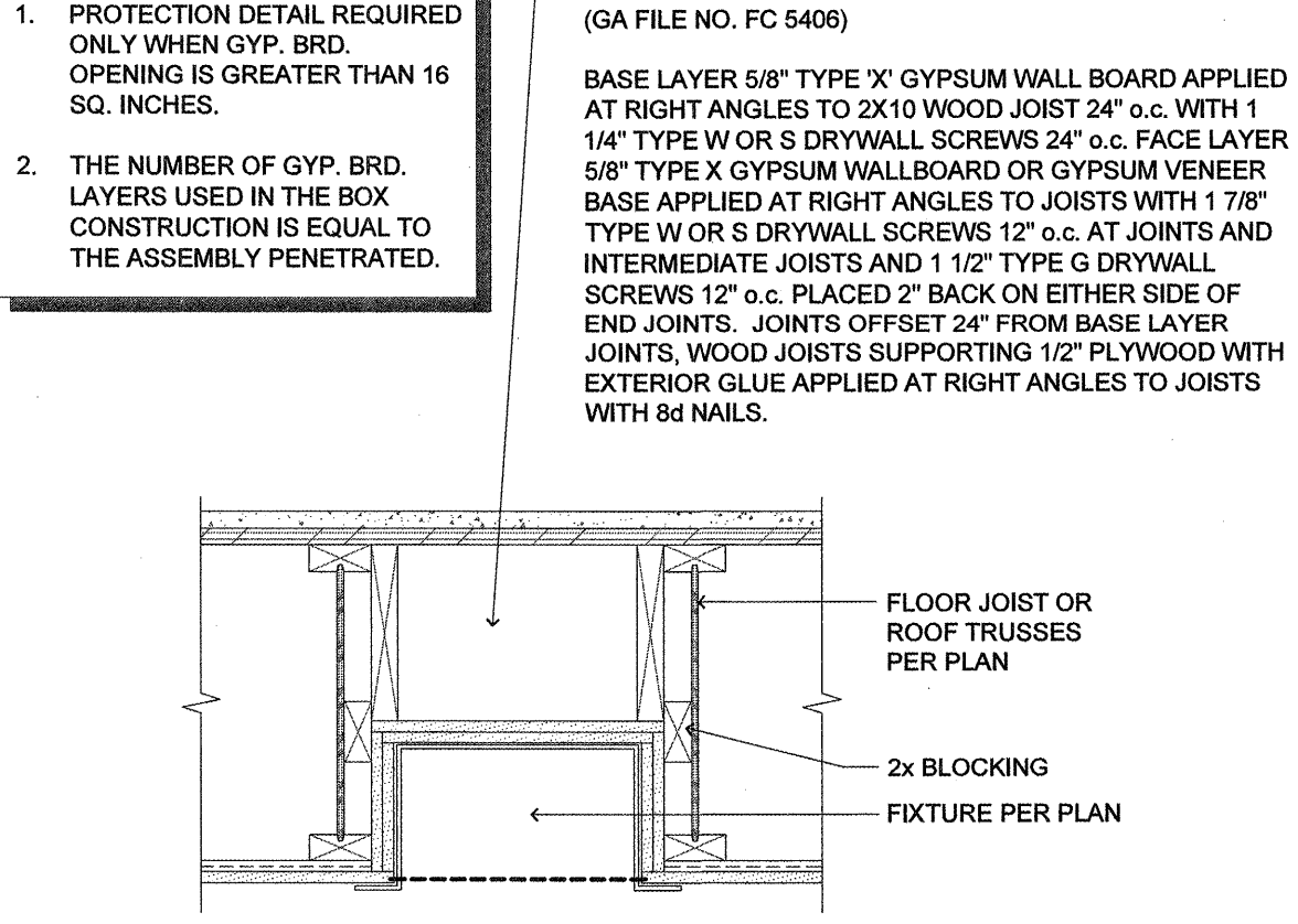
7 FIXTURE PROTECTION HEAT LAMP, LIGHT FIXTURE/SPEAKER SCALE: N.T.S.
