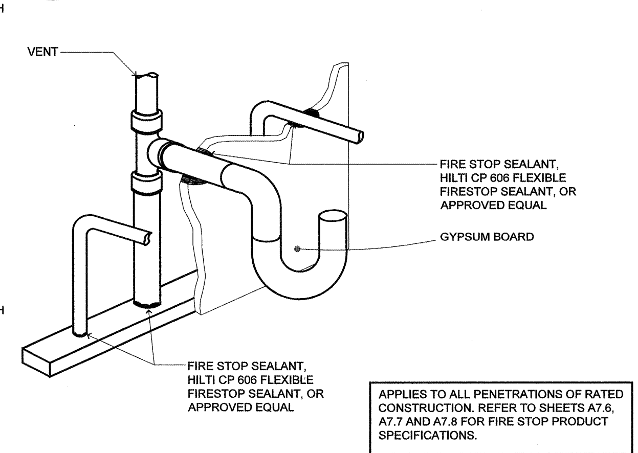
1 PLUMBING DETAIL (AT FIRE RATED CONSTRUCTION) SCALE: N.T.S.
