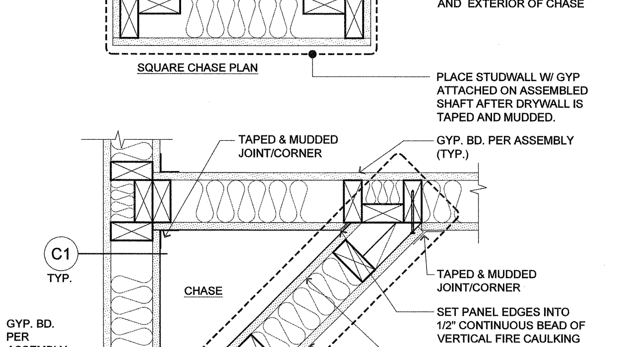
8 INT. WALL ASSEMBLY (1 HR MECHANICAL CHASE) SCALE: 1-1/2" = 1'-0"
