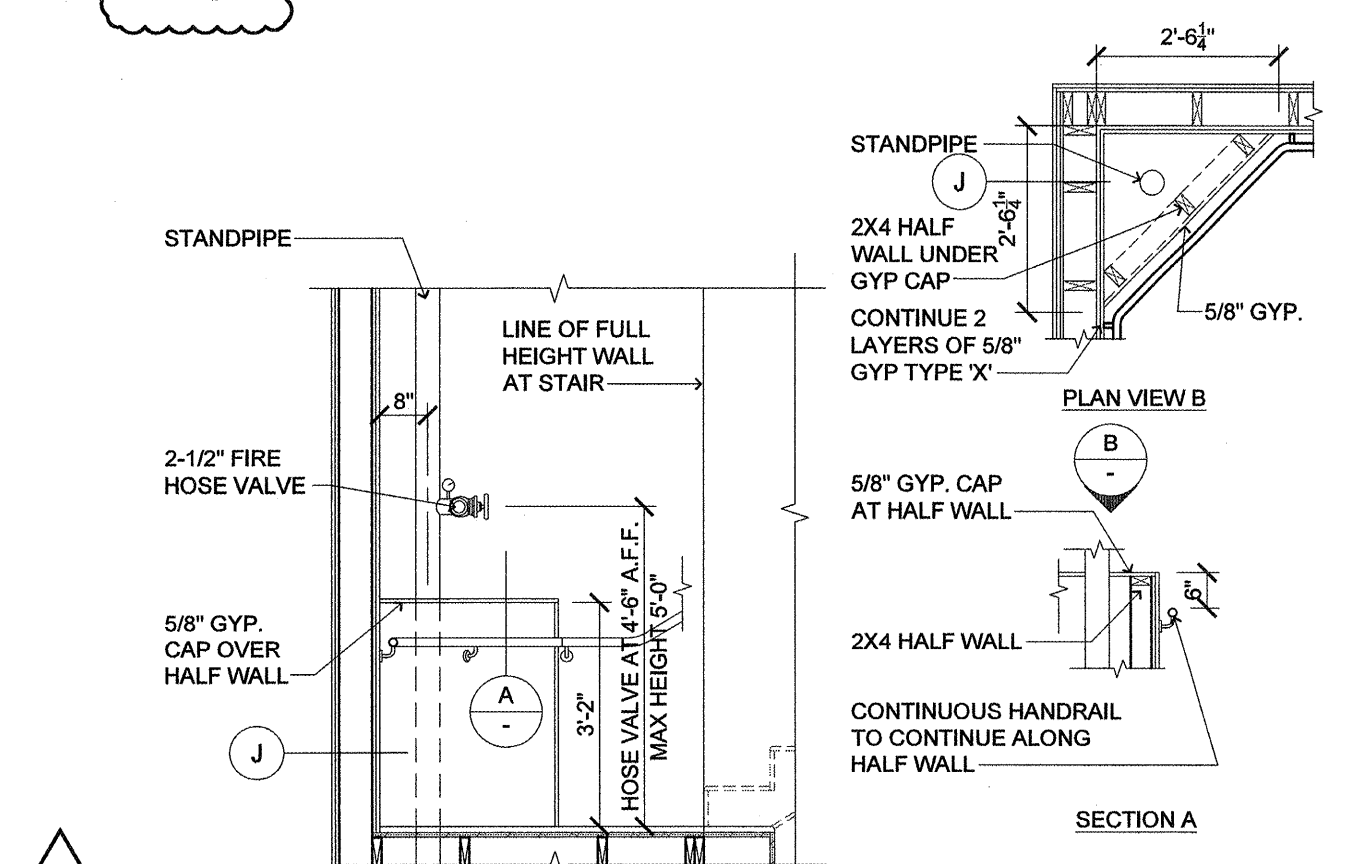
10 STANDPIPE HALF WALL (AT 2 HOUR STAIRS) SCALE: 3/8" = 1'-0"
