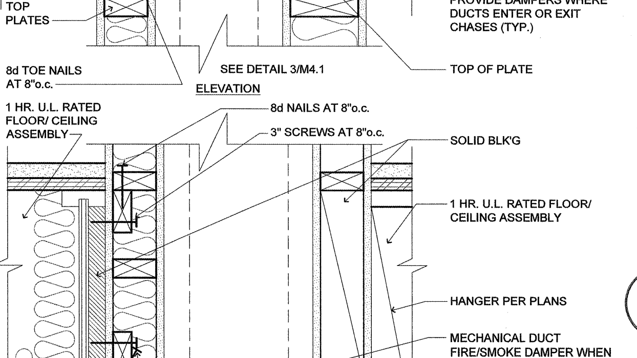
6 SECTION AT CORRIDOR (ALL TRADES TO COORDINATE AVAILABLE SPACE) SCALE: 1-1/2" = 1'-0"
