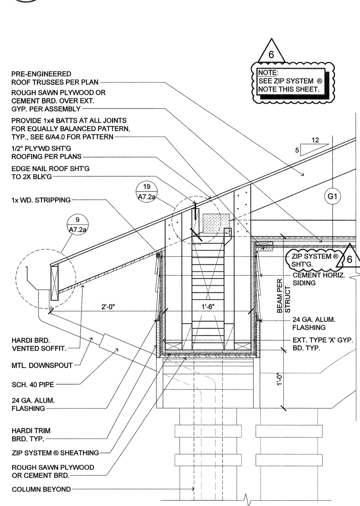
4 TRIM WORK ON SOFFIT BOX (ENTRY CANOPY) SCALE: 1" = 1'-0"
