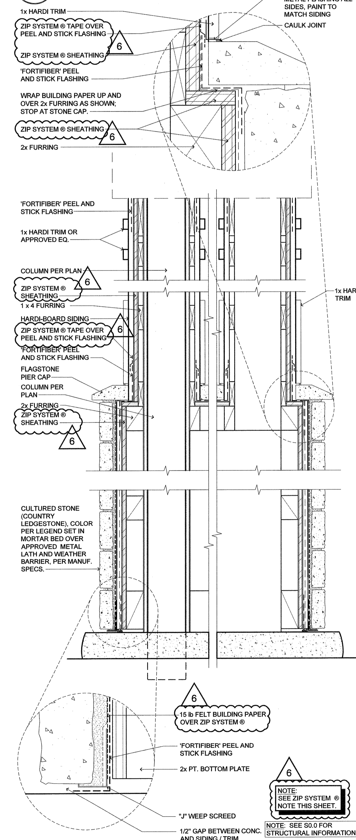
5 ENTRY CANOPY COLUMN (TRIM AND FLASHING) SCALE: 1 1/2" = 1'-0"
