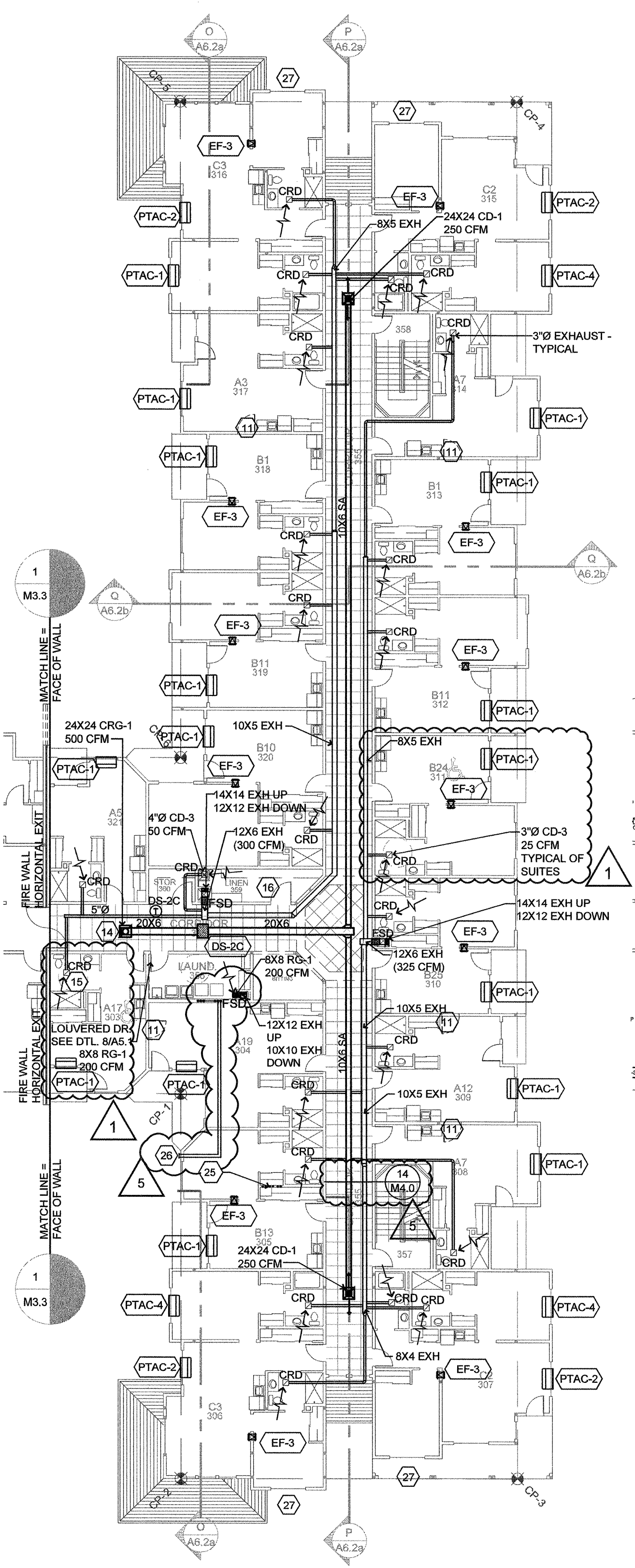
3 THIRD FLOOR - HVAC M3.6 SCALE: 1/16" = 1'-0"
