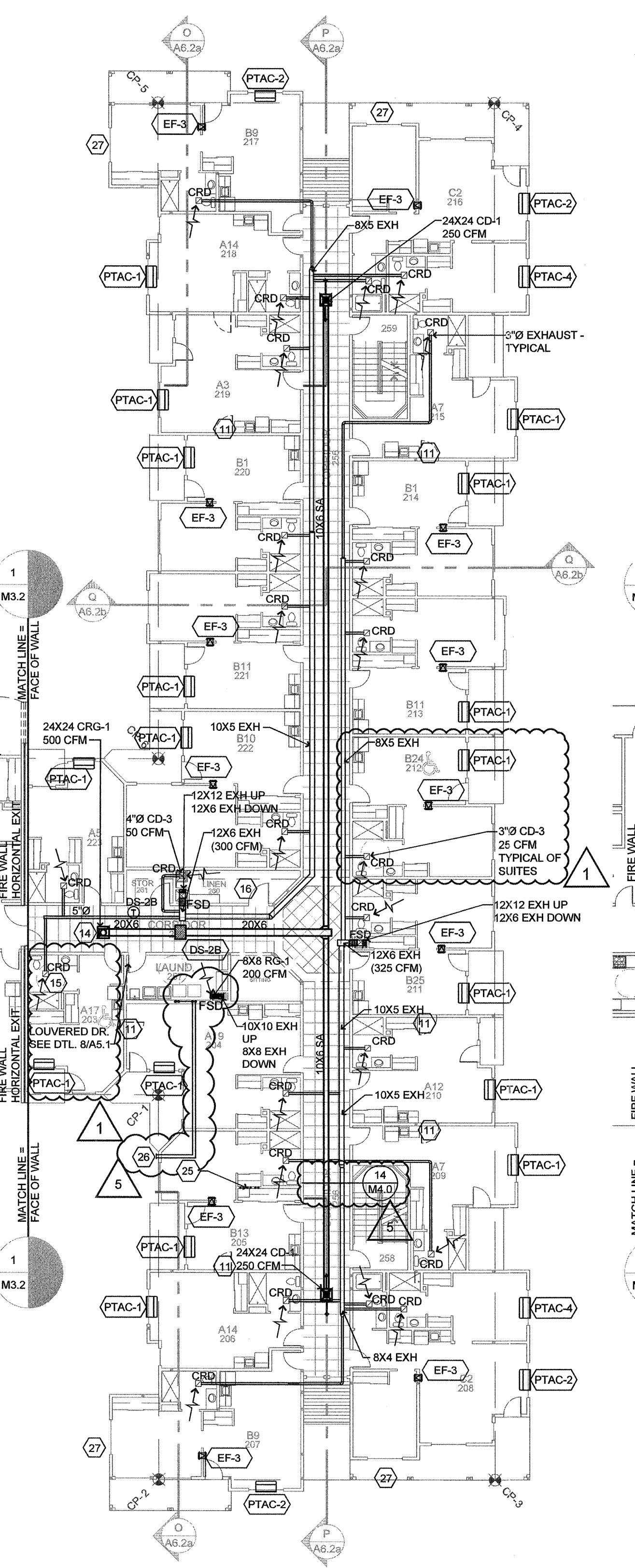
2 SECOND FLOOR - HVAC M3.6 SCALE: 1/16" = 1'-0"
