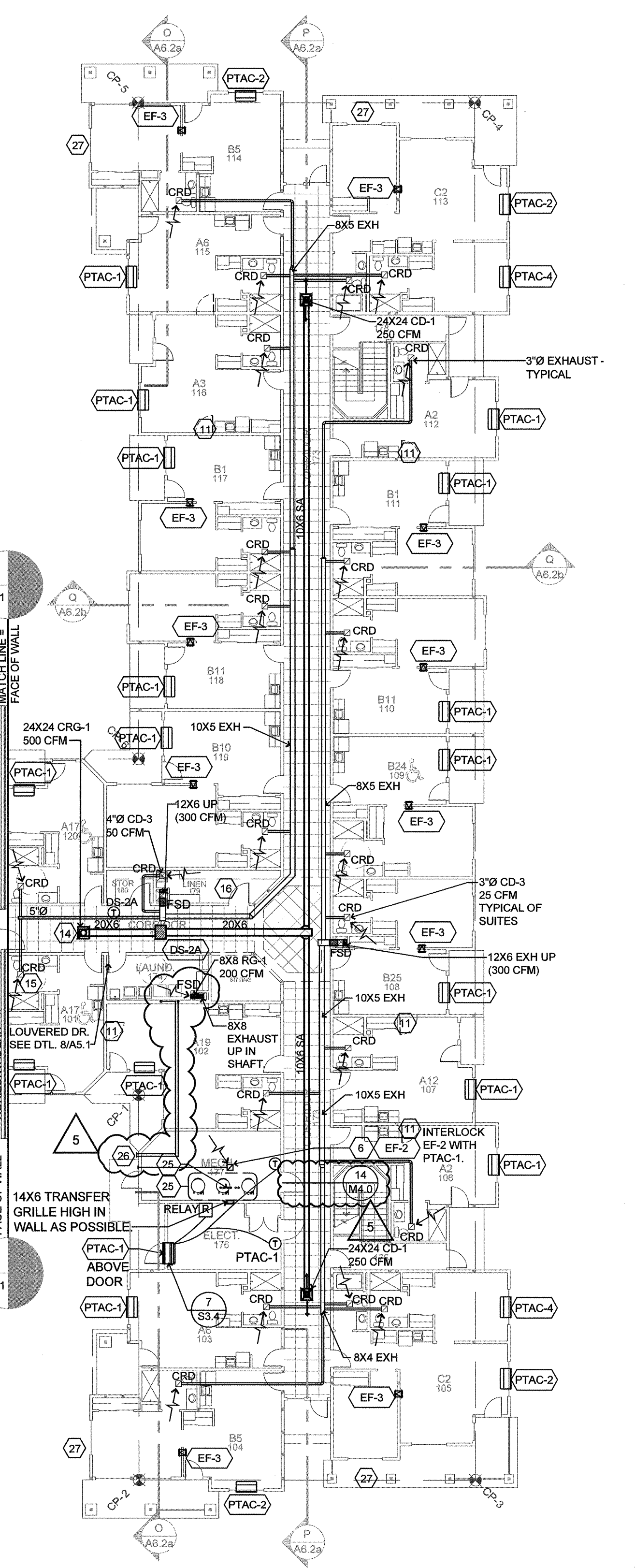
1 FIRST FLOOR - HVAC M3.6 SCALE: 1/16" = 1'-0"
