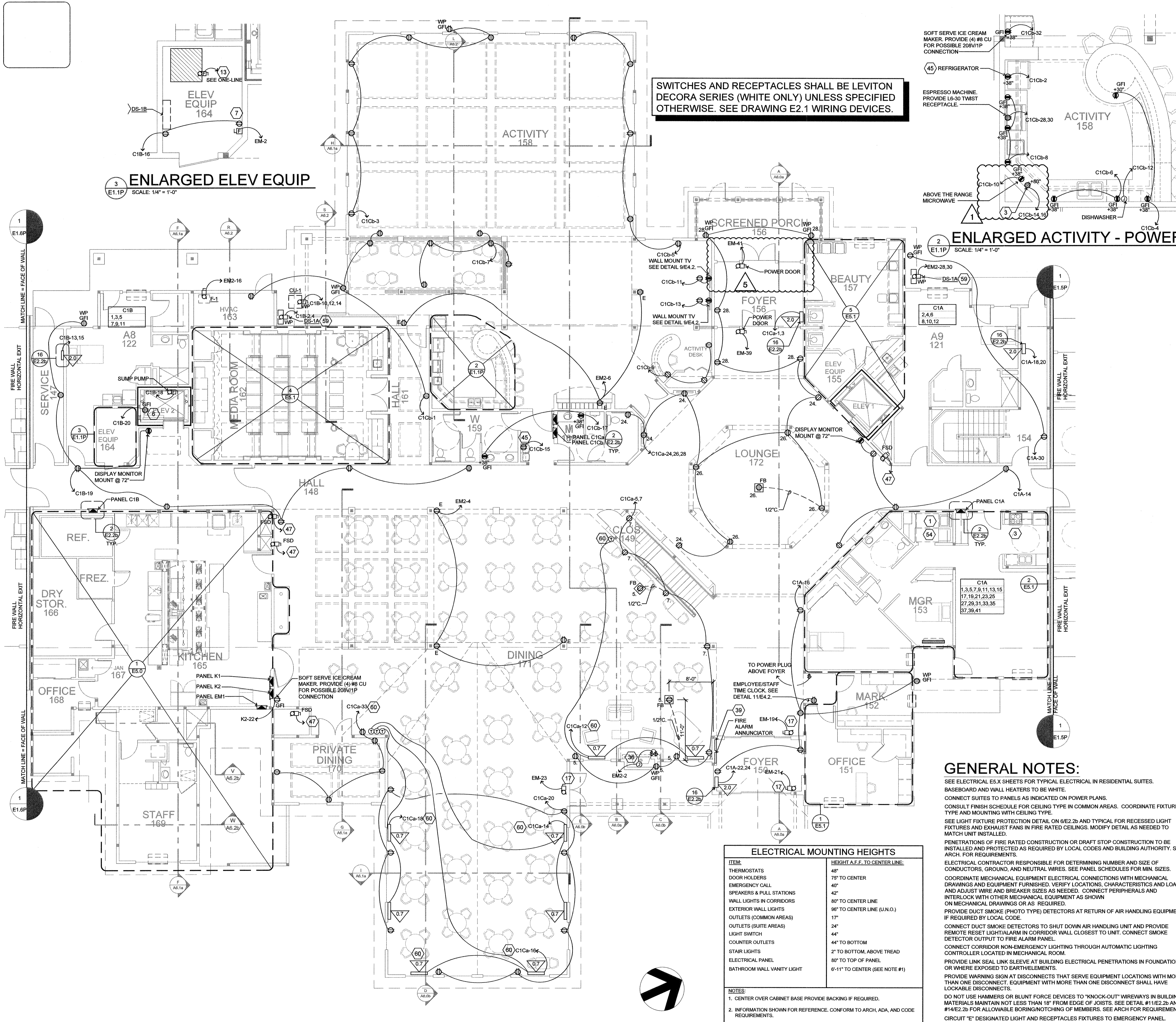
FIRST FLOOR - POWER SCALE: 1/8" = 1'-0"
