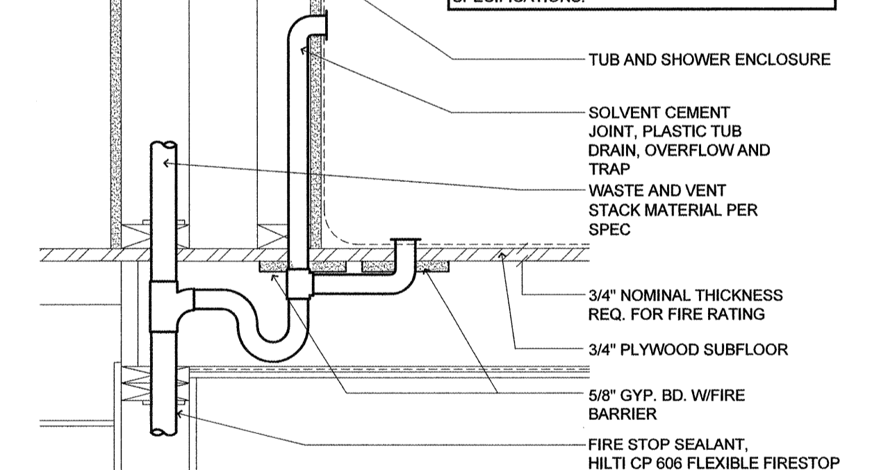
3 SECTION AT CORRIDOR (ALL TRADES TO COORDINATE AVAILABLE SPACE) SCALE: 1-1/2" = 1'-0"
