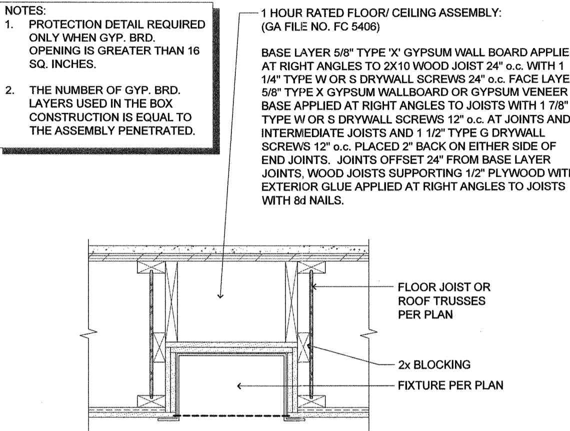
6 SECTION AT CORRIDOR (ALL TRADES TO COORDINATE AVAILABLE SPACE) SCALE: 1-1/2" = 1'-0"
