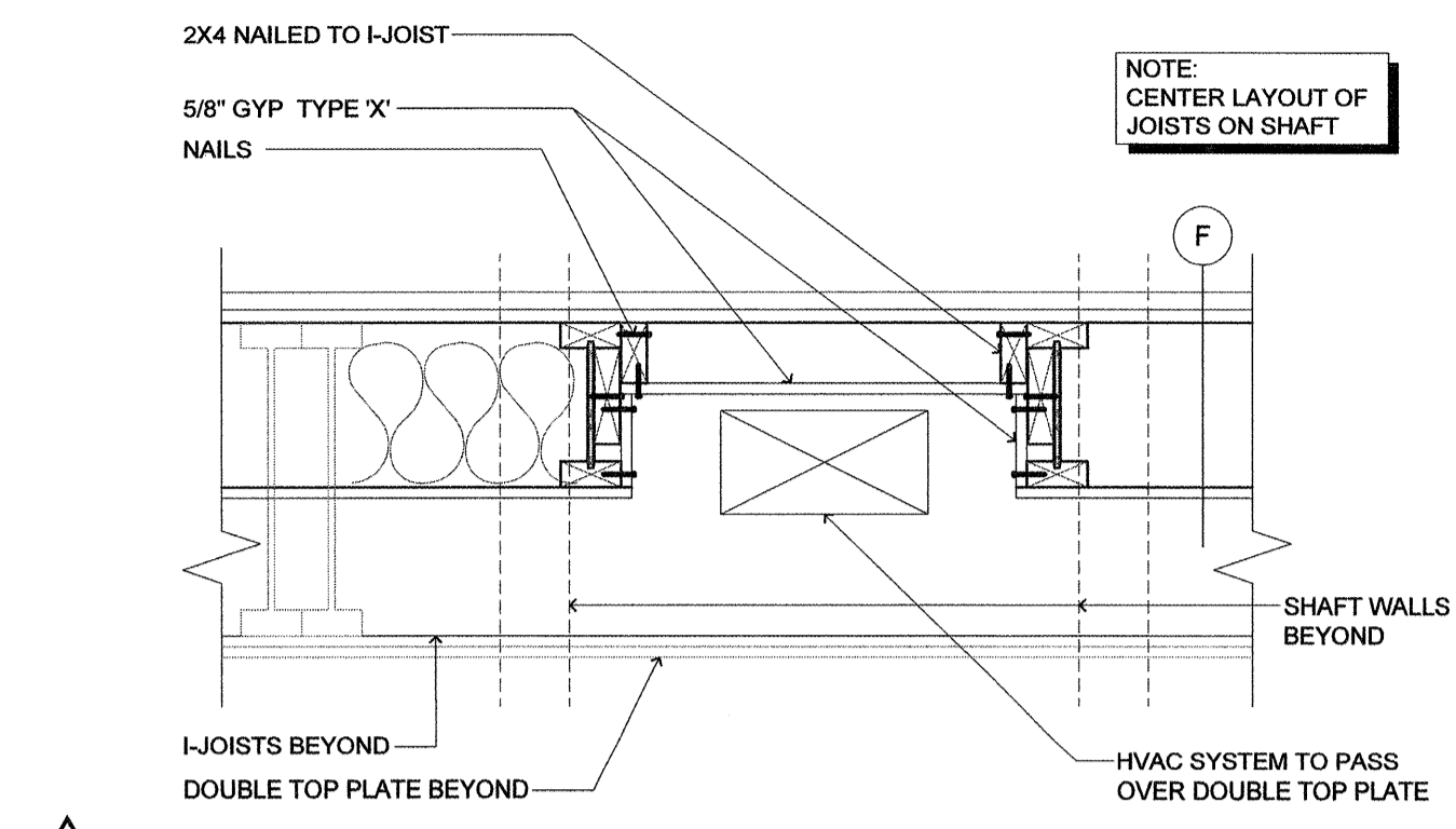
11 HVAC ABOVE DOUBLE TOP PLATE (TRANSFER FROM SHAFT TO CORRIDOR) SCALE: 1" = 1'-0"
