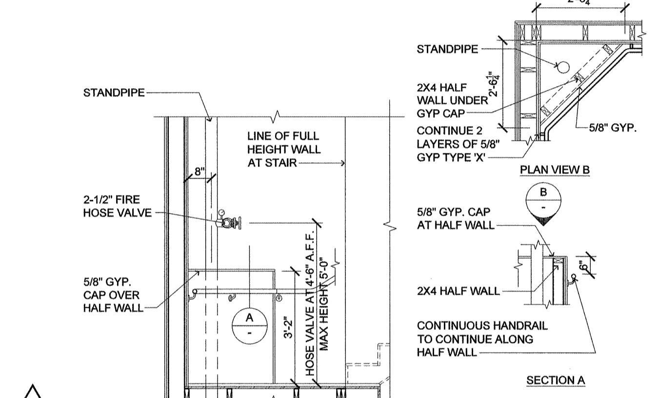
10 STANDPIPE HALF WALL (AT 2 HOUR STAIRS) SCALE: 3/8" = 1'-0"
