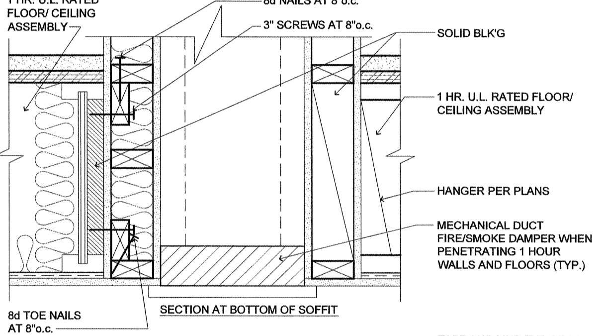
3 SECTION AT CORRIDOR (ALL TRADES TO COORDINATE AVAILABLE SPACE) SCALE: 1-1/2" = 1'-0"
