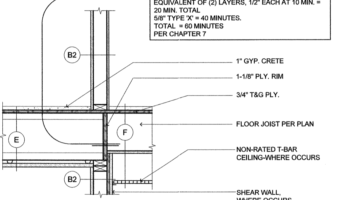
5 ELEC. PANEL (FIRE RATED) SCALE: N.T.S.
