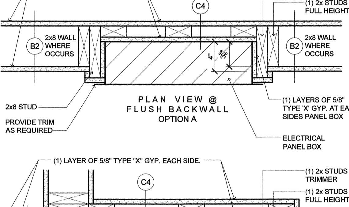
8 INT. WALL ASSEMBLY (1 HR MECHANICAL CHASE) SCALE: 1-1/2" = 1'-0"
