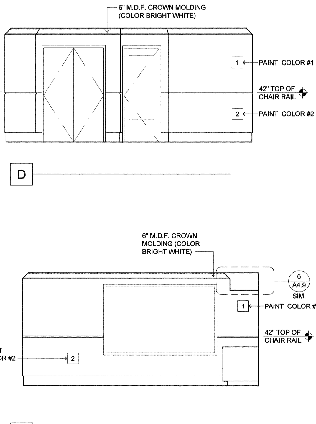
2 ENLARGED PLANS, ELEVATIONS (READING ROOM) SCALE: 1/4" = 1'-0"
