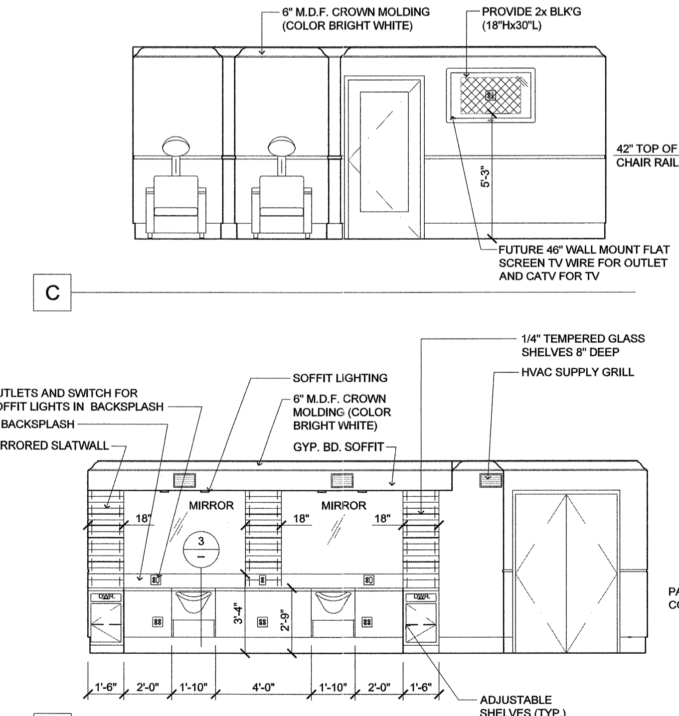
1 INTERIOR ELEVATIONS (BEAUTY) SCALE: 1/4" = 1'-0"
