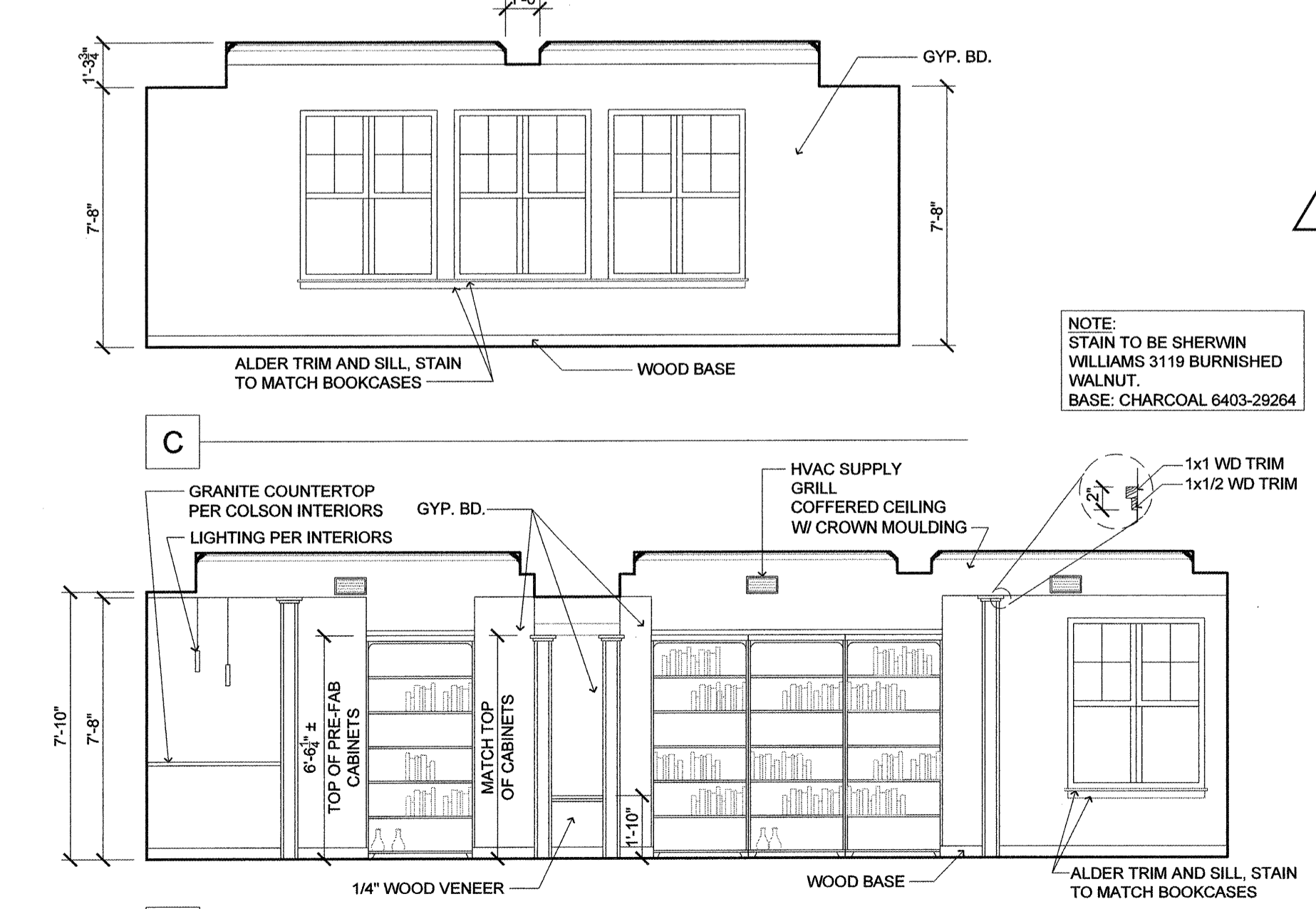
2 ENLARGED PLANS, ELEVATIONS (READING ROOM) SCALE: 1/4" = 1'-0"
