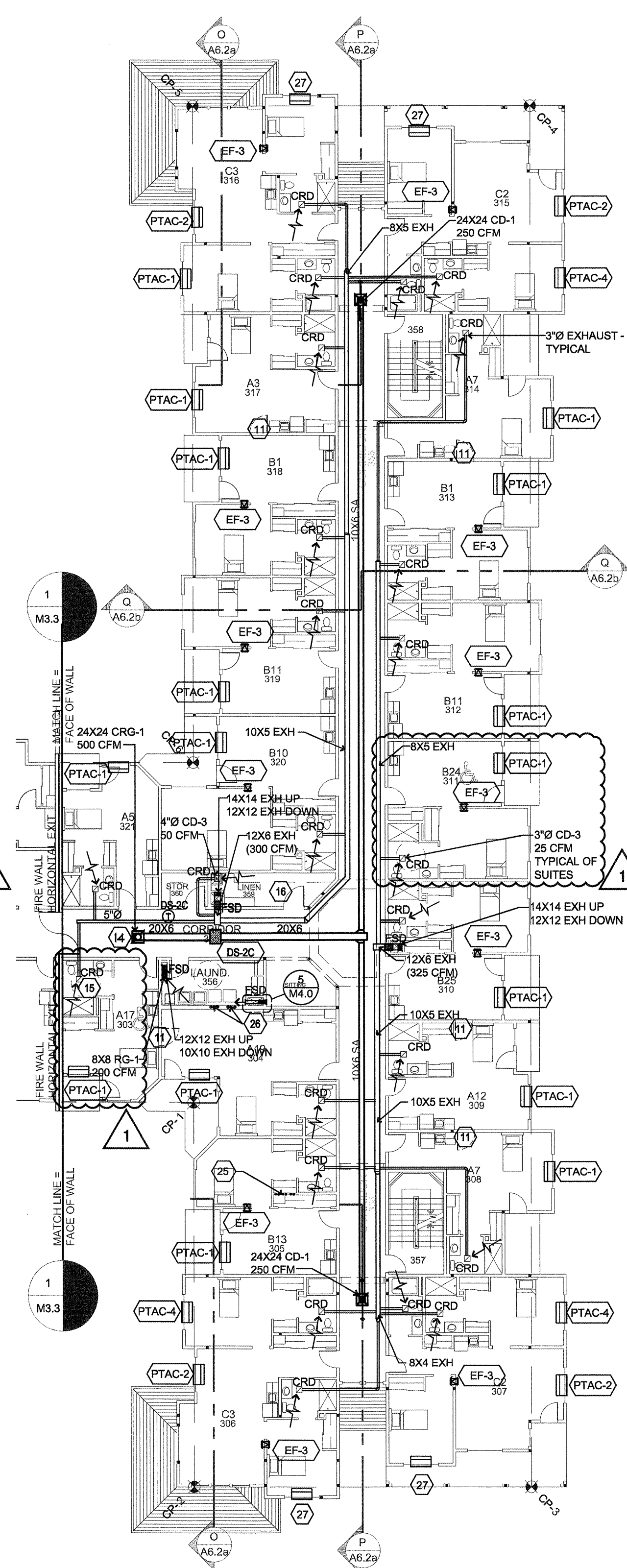
3 THIRD FLOOR - HVAC M3.6 SCALE: 1/16" = 1'-0"
