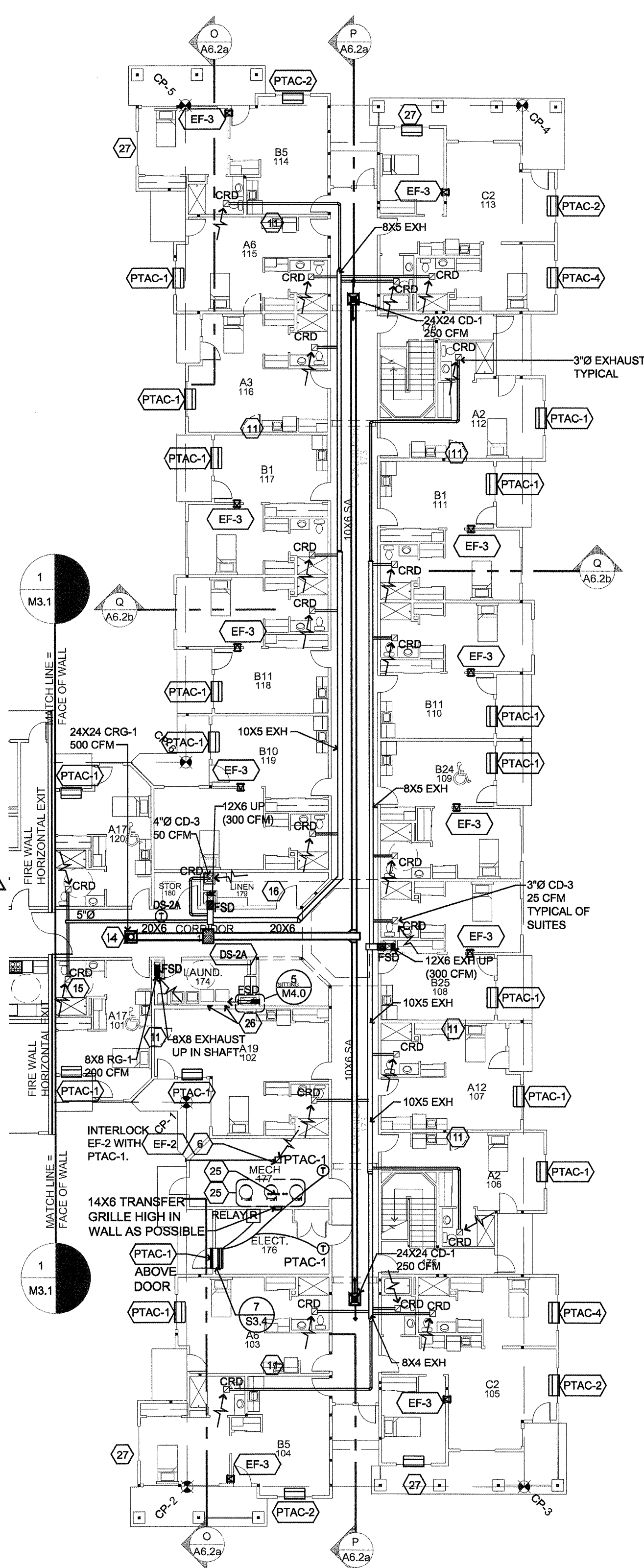
1 FIRST FLOOR - HVAC M3.6 SCALE: 1/16" = 1'-0"
