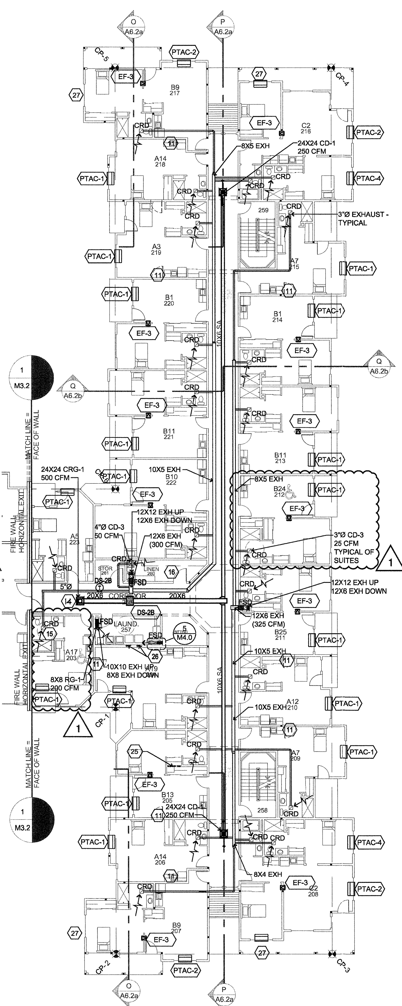
2 SECOND FLOOR - HVAC M3.6 SCALE: 1/16" = 1'-0"
