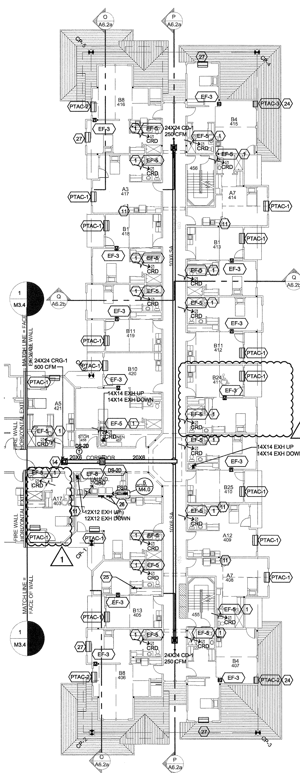
4 FOURTH FLOOR - HVAC M3.6 SCALE: 1/16" = 1'-0"
