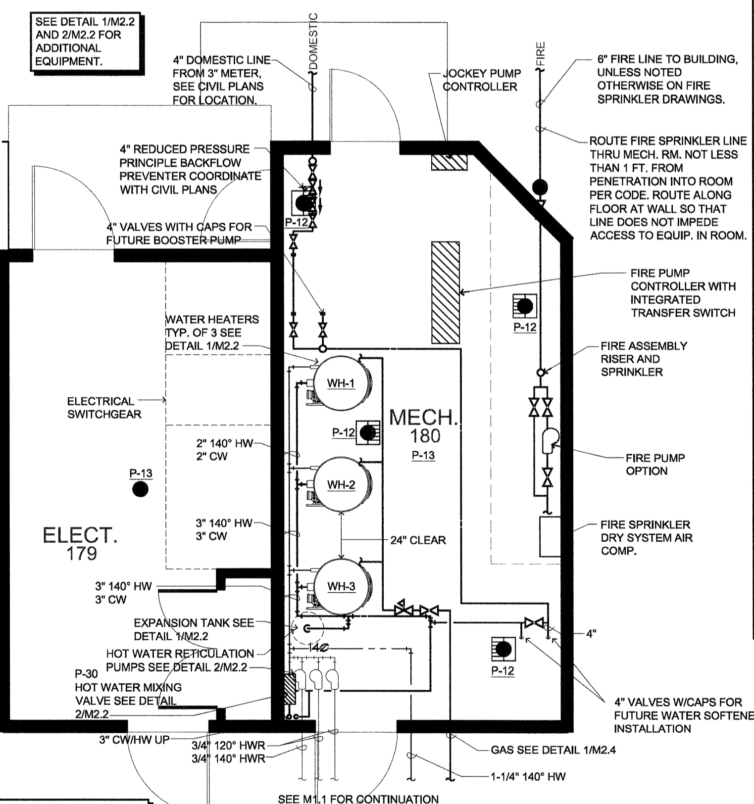
1 PLUMBING DETAIL (MECHANICAL ROOM PLAN) SCALE: 1/4" = 1'-0"
