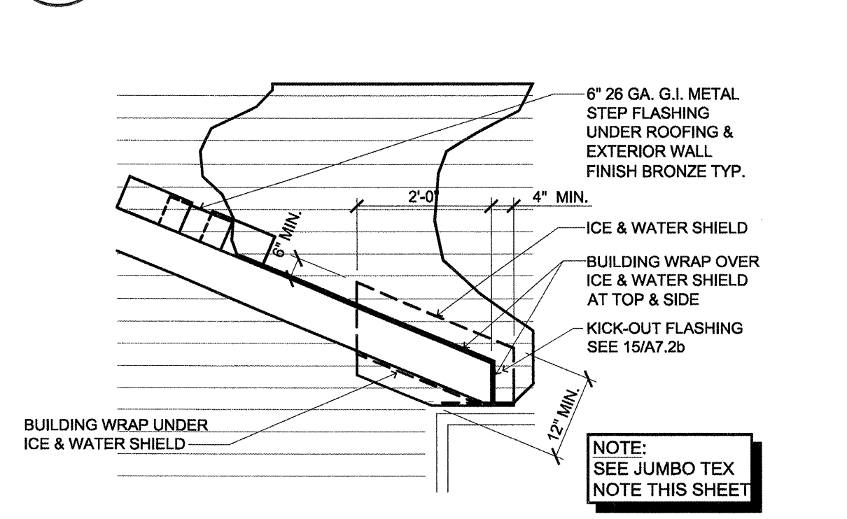
18 ROOF FLASHING SCALE: 1/2" = 1'-0"
