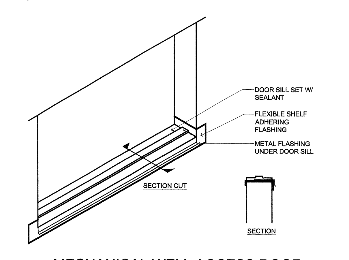
14 MECHANICAL WELL ACCESS DOOR (SILL DETAIL) SCALE: 1" = 1'-0"
