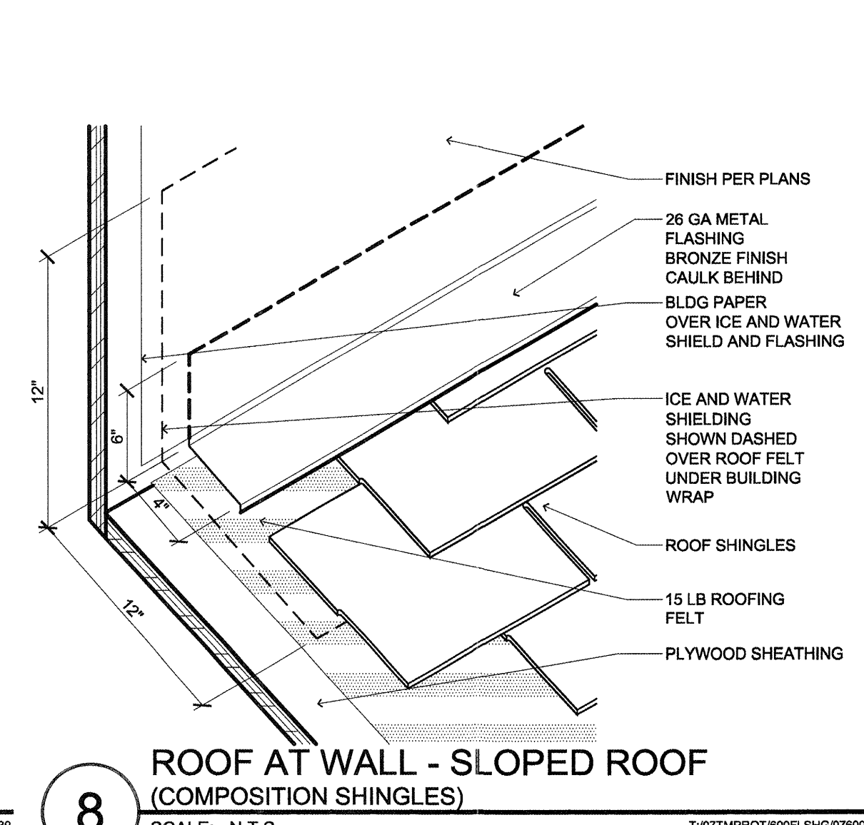
8 ROOF AT WALL - SLOPED ROOF (COMPOSITION SHINGLES) SCALE: N.T.S.
