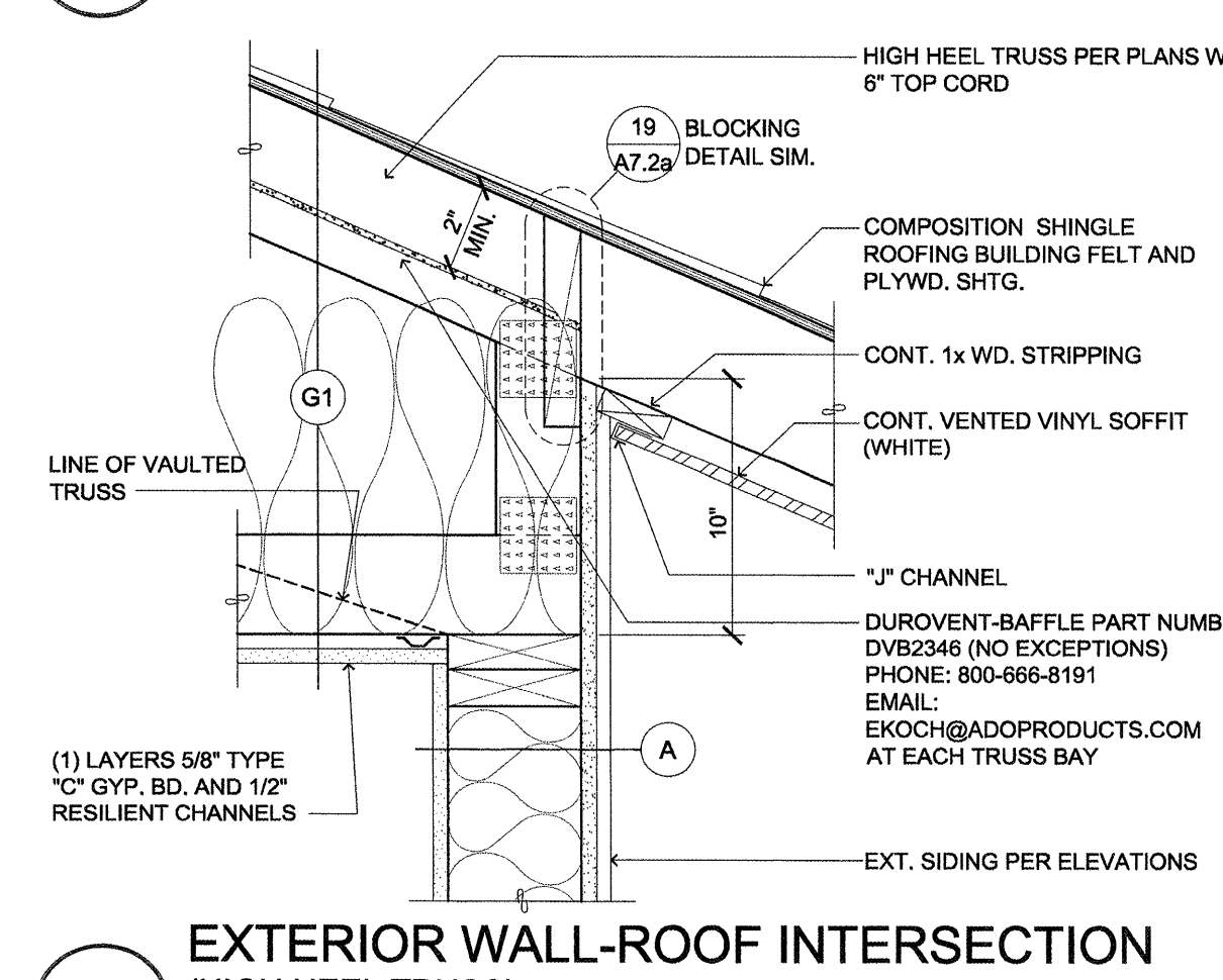
13 EXTERIOR WALL-ROOF INTERSECTION (HIGH HEEL TRUSSES) SCALE: N.T.S.
