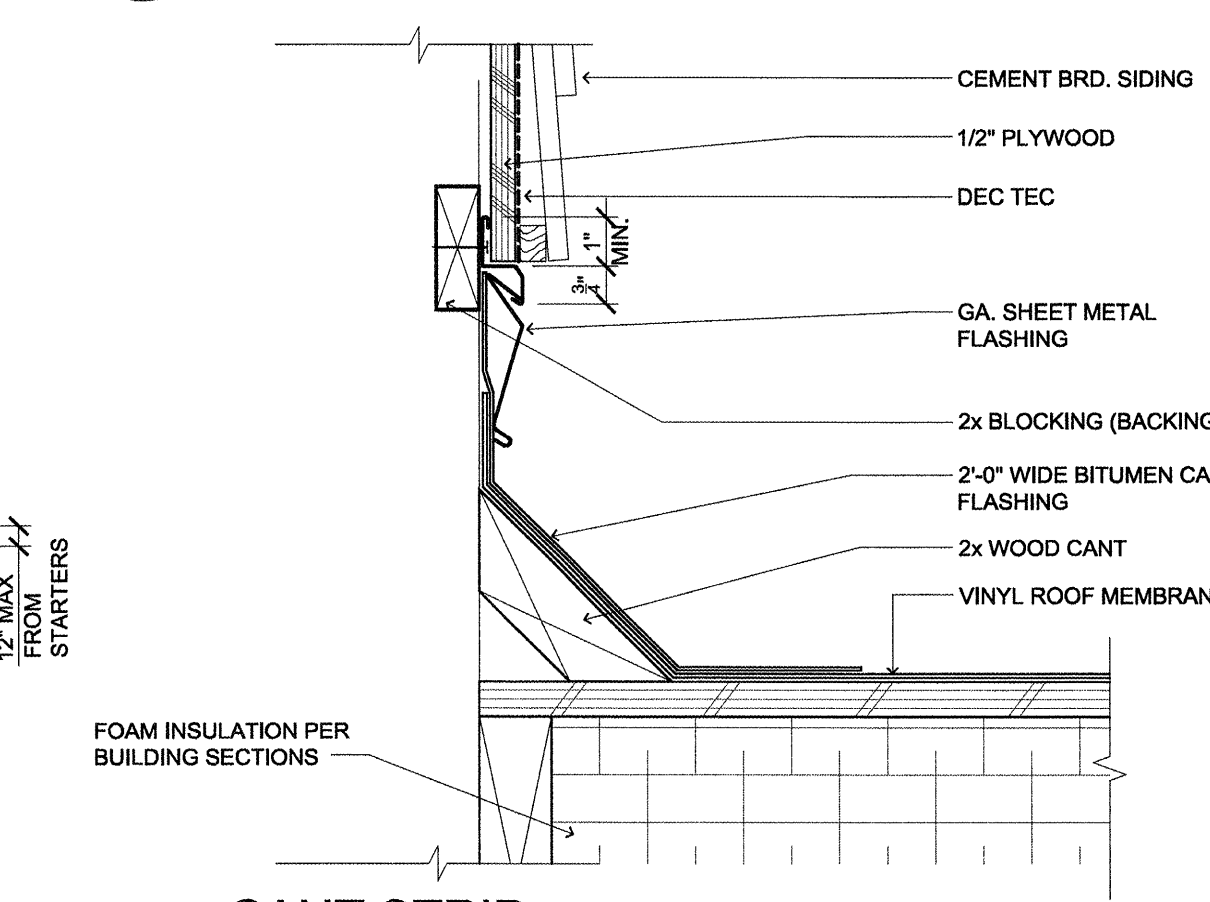
2 CANT STRIP (BUILT-UP ROOFING) SCALE: 3" = 1'-0"
