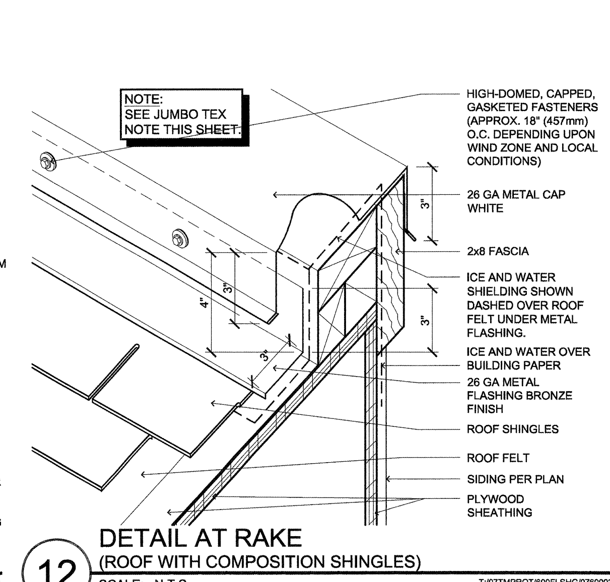
12 DETAIL AT RAKE (ROOF WITH COMPOSITION SHINGLES) SCALE: N.T.S.
