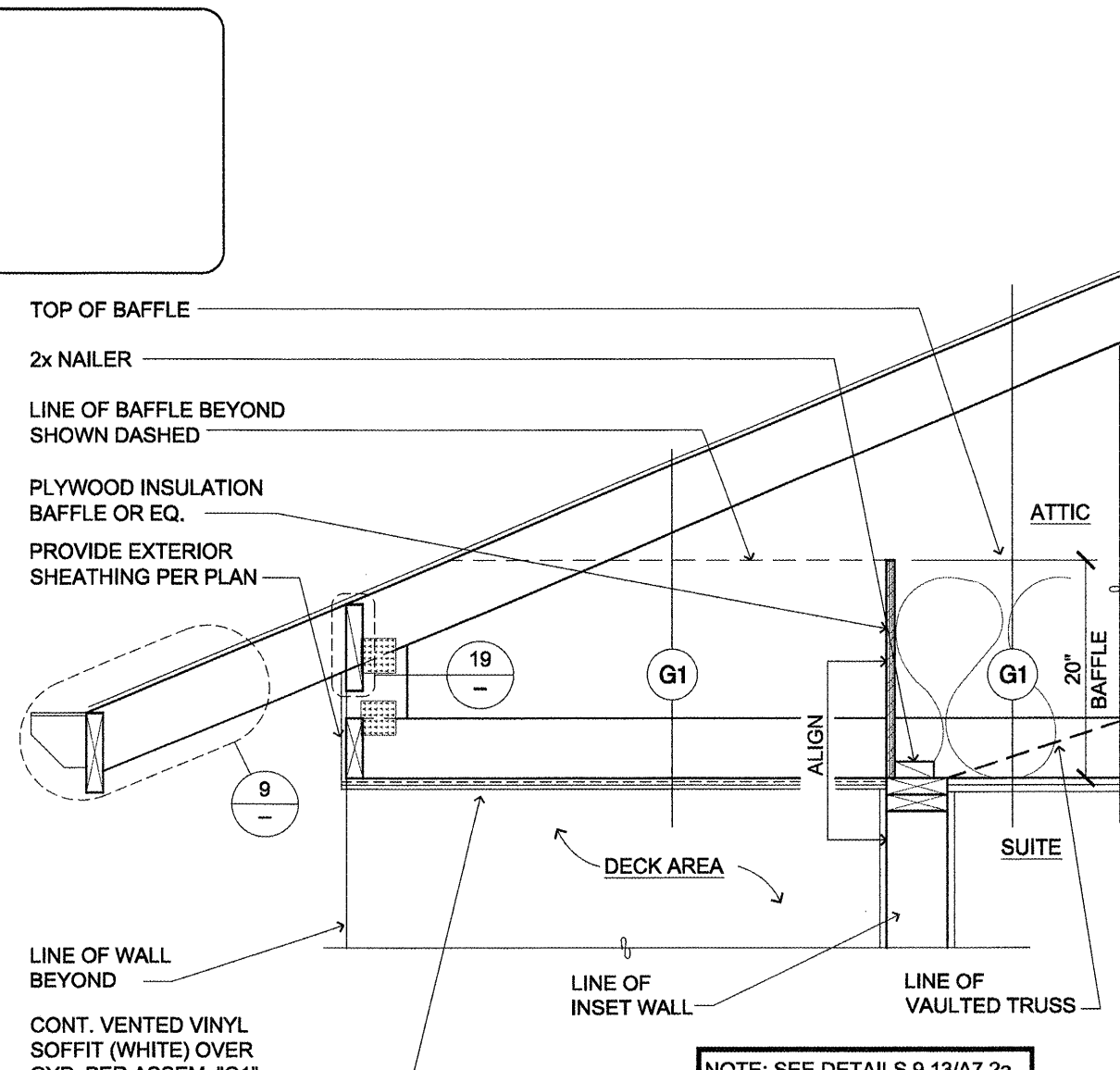
20 INSUL. BAFFLE (AT DECK AND OVERHANGS GREATER THAN 24") SCALE: 3/4" = 1'-0"
