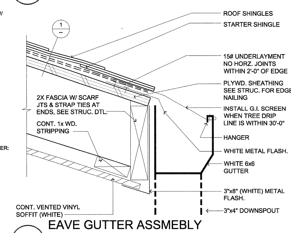
9 EAVE GUTTER ASSEMBLY (ROOF WITH COMPOSITION SHINGLES) SCALE: 3" = 1'-0"
