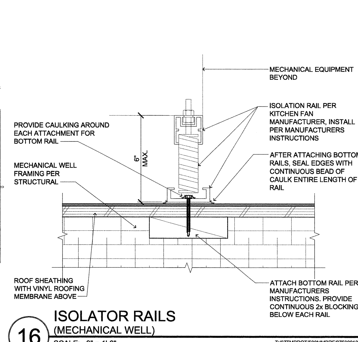
16 ISOLATOR RAILS (MECHANICAL WELL) SCALE: 3" = 1'-0"
