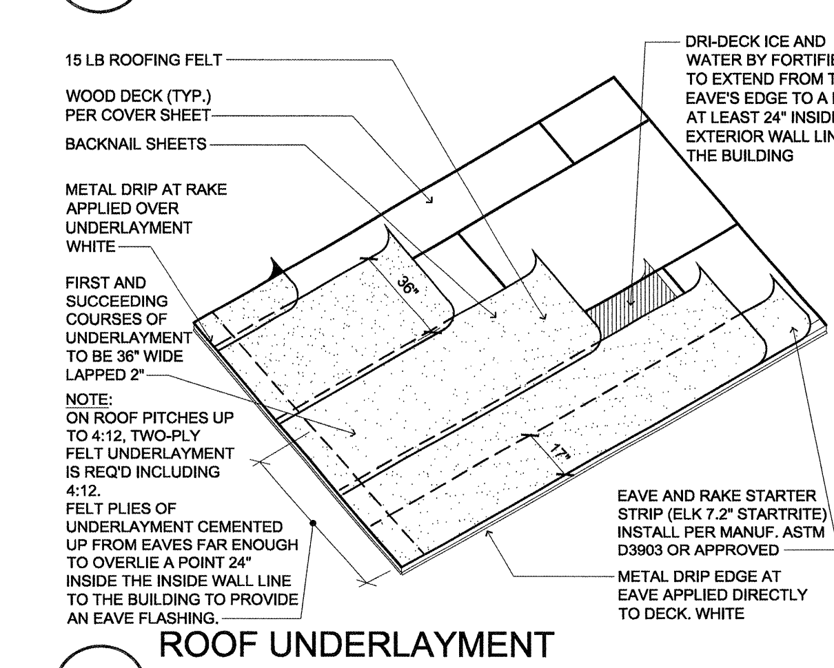
1 ROOF UNDERLAYMENT (ASSEMBLY DETAIL) SCALE: N.T.S.
