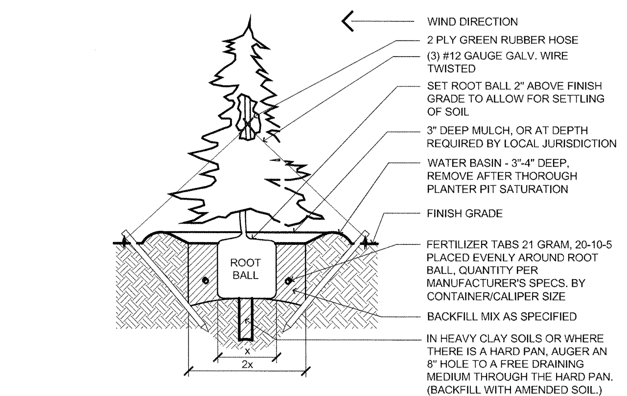
1 CONIFER TREE PLANTING (SECTION) SCALE: NOT TO SCALE T:\02SITE\WK\220EXCAV\02220008
