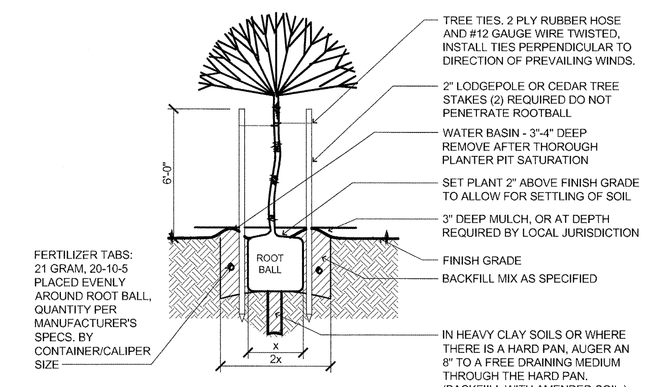
2 TREE PLANTING (SECTION) SCALE: NOT TO SCALE T:\02SITE\WK\220EXCAV\02220007
