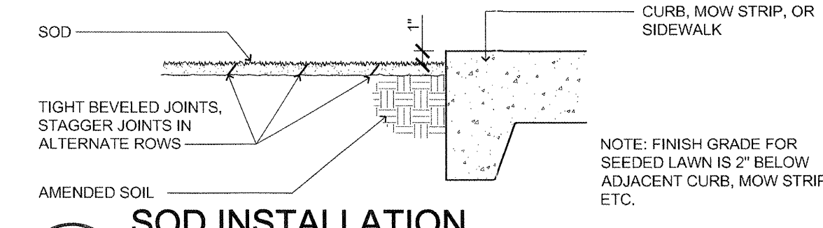
5 SOD INSTALLATION SCALE: NOT TO SCALE T:\02SITE\WK\220EXCAV\02220010
