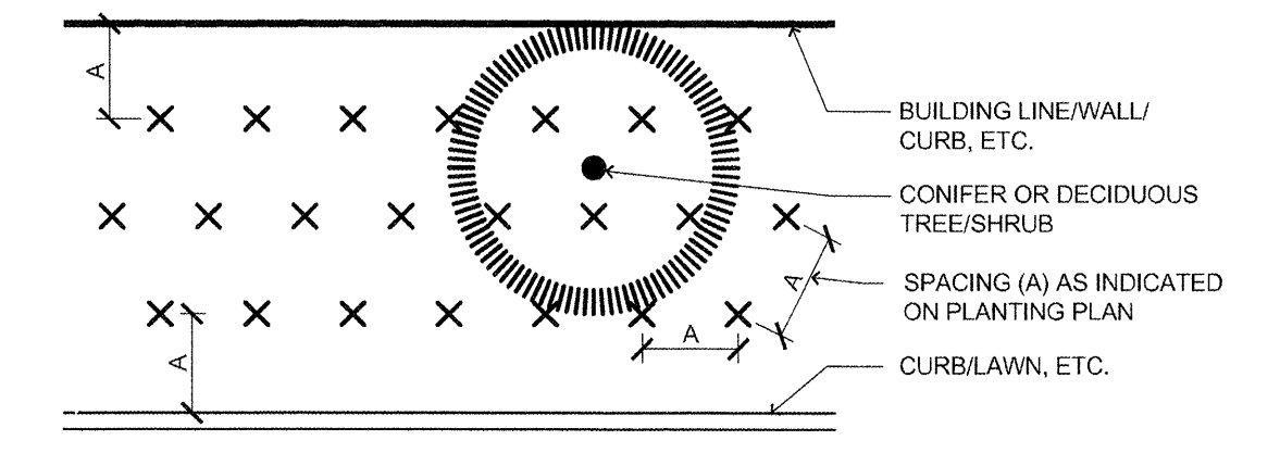
4 GROUNDCOVER PLANTING SCALE: NOT TO SCALE T:\02SITE\WK\220EXCAV\02220008
