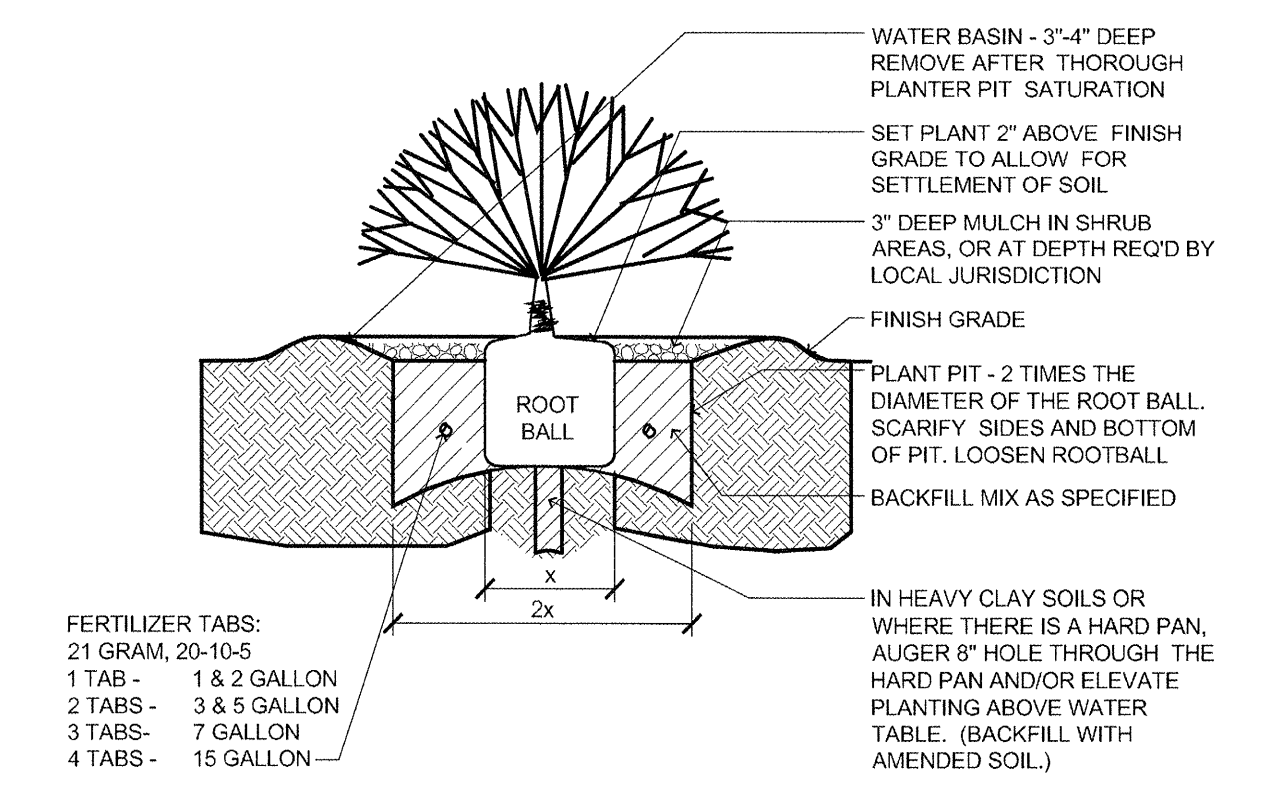
3 SHRUB/GROUNDCOVER PLANTING (SECTION) SCALE: NOT TO SCALE T:\02SITE\WK\220EXCAV\02220008
