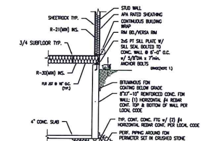
NOTE: 1. THE GROUND IMMEDIATELY ADJACENT TO THE FOUNDATION SHALL BE SLOPED AWAY FROM THE BUILDING AT A SLOPE OF 1/2\"/> 2. SUBSTITUTE FLR JOSTS AND STUD WALL SIZES WITH PLAN CALL OUT TYPICAL INS. BETWEEN FDN & 1st FLR N.T.S.
