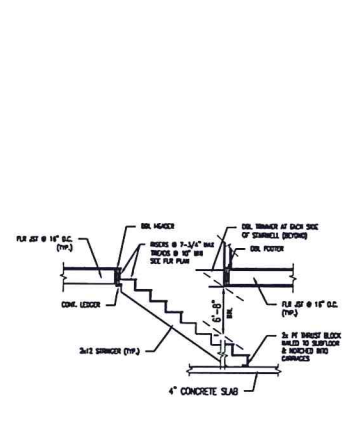
NOTE: 1. SUBSTITUTE RAFTER, CL. JSTS & STUD WALL SIZES WITH PLAN CALL OUT TYPICAL STAIR FRAMING N.T.S.
