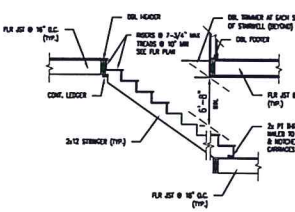
NOTE: 1. SUBSTITUTE RAFTER, CL. JSTS & STUD WALL SIZES WITH PLAN CALL OUT TYPICAL STAIR FRAMING N.T.S.
