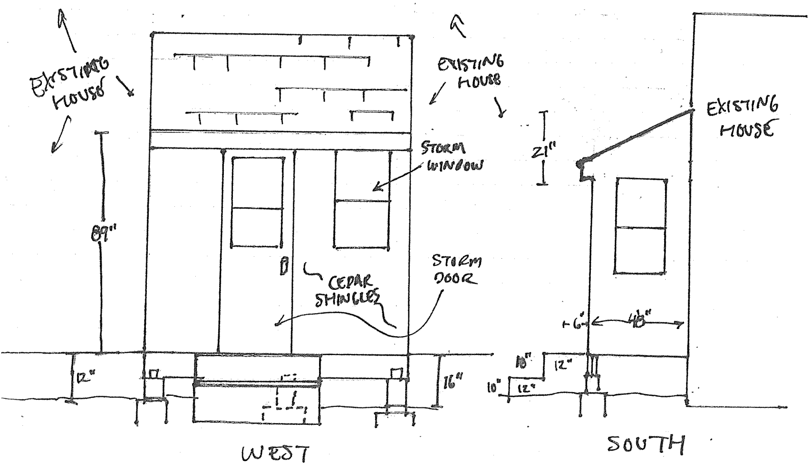
ELEVATION DRAWINGS
